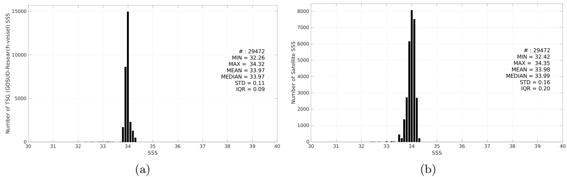
Figure 3: Histograms of SSS from TSG (GOSUD-Research-vessel) (a) and CCI SSS L4 Merged-OI v5.5 - 7-day running (ESA) (b) considering all match-up pairs per bins of 0.1 over the Southern Ocean Pi-MEP region and for the full satellite product period.
