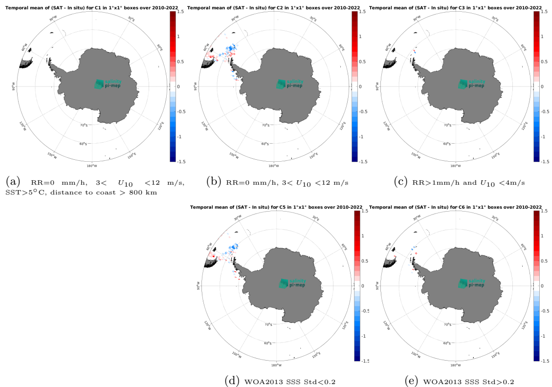
Figure 14: Temporal mean gridded over spatial boxes of size 1^\circ \times 1^\circ of \Delta SSS (CCI SSS L4 Merged-OI v5.5 - 7-day running (ESA) - TSG (CSIC-UTM)) for 5 different subdatasets corresponding to:RR=0 mm/h, 3 < U_{10} < 12 m/s, SST >5^\circ\text{C} , distance to coast > 800 km (a), RR=0 mm/h, 3 < U_{10} < 12 m/s (b), RR >1 mm/h and U_{10} < 4 m/s (c), WOA2013 SSS Std <0.2 (d), WOA2013 SSS Std >0.2 (e).
