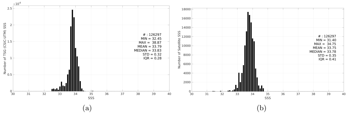
Figure 3: Histograms of SSS from TSG (CSIC-UTM) (a) and CCI SSS L4 Merged-OI v5.5 - 7-day running (ESA) (b) considering all match-up pairs per bins of 0.1 over the Southern Ocean Pi-MEP region and for the full satellite product period.
