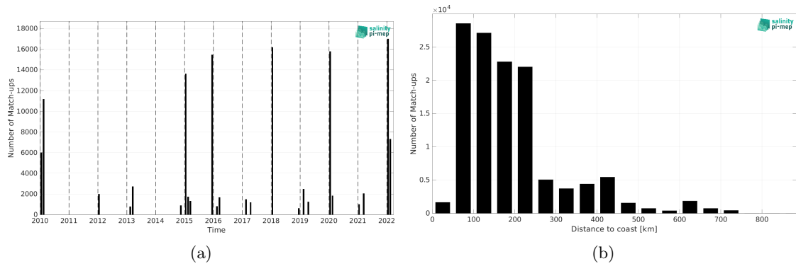
Figure 2: Number of match-ups between TSG (CSIC-UTM) and CCI SSS L4 Merged-OI v5.5 - 7-day running (ESA) SSS as a function of time (a) and as function of the distance to coast (b) over the Southern Ocean Pi-MEP region and for the full satellite product period.
