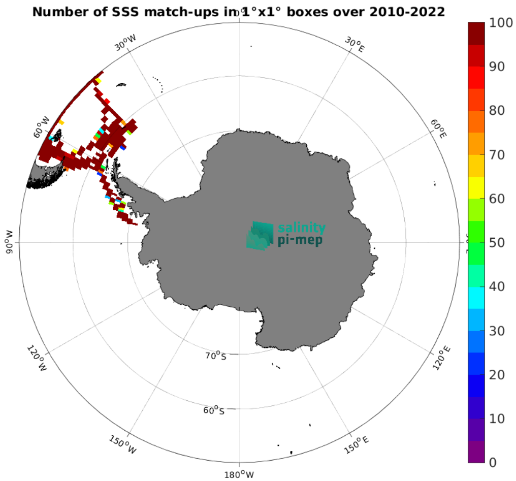
Figure 5: Number of SSS match-ups between TSG (CSIC-UTM) SSS and the CCI SSS L4 Merged-OI v5.5 - 7-day running (ESA) SSS product for the Southern Ocean Pi-MEP region over 1^\circ \times 1^\circ boxes and for the full satellite product period.
