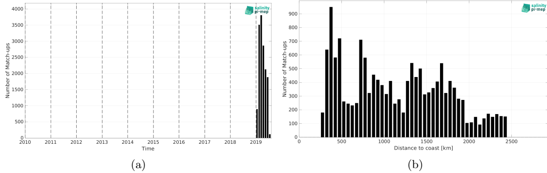
Figure 2: Number of match-ups between Saildrone and CCI SSS L4 Merged-OI v5.5 - 7-day running (ESA) SSS as a function of time (a) and as function of the distance to coast (b) over the Southern Ocean Pi-MEP region and for the full satellite product period.
