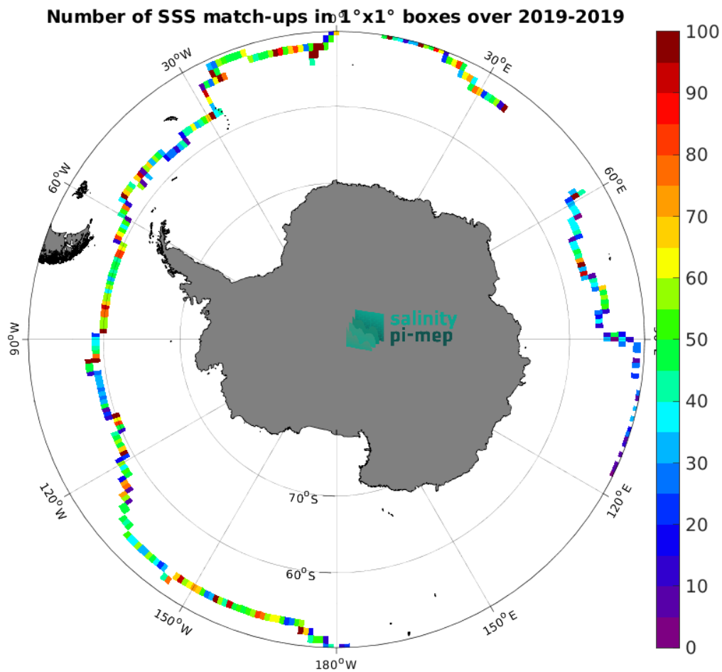
Figure 5: Number of SSS match-ups between Saildrone SSS and the CCI SSS L4 Merged-OI v5.5 - 7-day running (ESA) SSS product for the Southern Ocean Pi-MEP region over 1^{\circ} \times 1^{\circ} boxes and for the full satellite product period.
