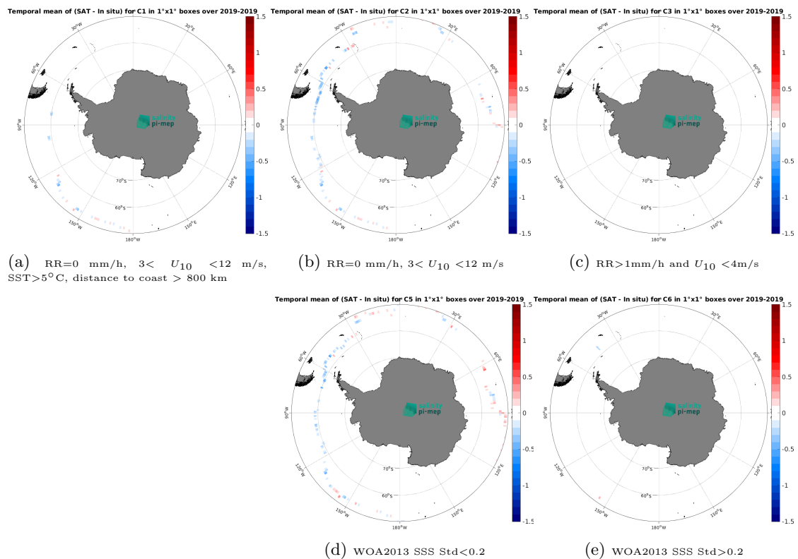
Figure 14: Temporal mean gridded over spatial boxes of size 1^\circ \times 1^\circ of \Delta SSS (CCI SSS L4 Merged-OI v5.5 - 7-day running (ESA) - Sairdrone) for 5 different subdatasets corresponding to:RR=0 mm/h, 3 < U_{10} < 12 m/s, SST > 5^\circ\text{C} , distance to coast > 800 km (a), RR=0 mm/h, 3 < U_{10} < 12 m/s (b), RR > 1 mm/h and U_{10} < 4 m/s (c), WOA2013 SSS Std < 0.2 (d), WOA2013 SSS Std > 0.2 (e).
