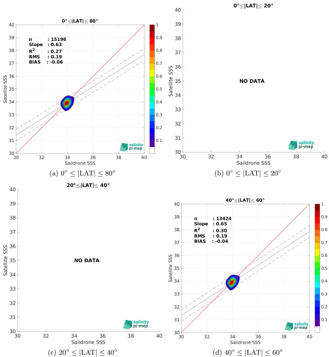
Figure 10: Contour maps of the concentration of CCI SSS L4 Merged-OI v5.5 - 7-day running (ESA) SSS (y-axis) versus Sailldrone SSS (x-axis) at match-up pairs for different latitude bands. For each plot, the red line shows x=y . The black thin and dashed lines indicate a linear fit through the data cloud and the \pm 95\% confidence levels, respectively. The number match-up pairs n , the slope and R^2 coefficient of the linear fit, the root mean square (RMS) and the mean bias between satellite and in situ data are indicated for each latitude band in each plots.
