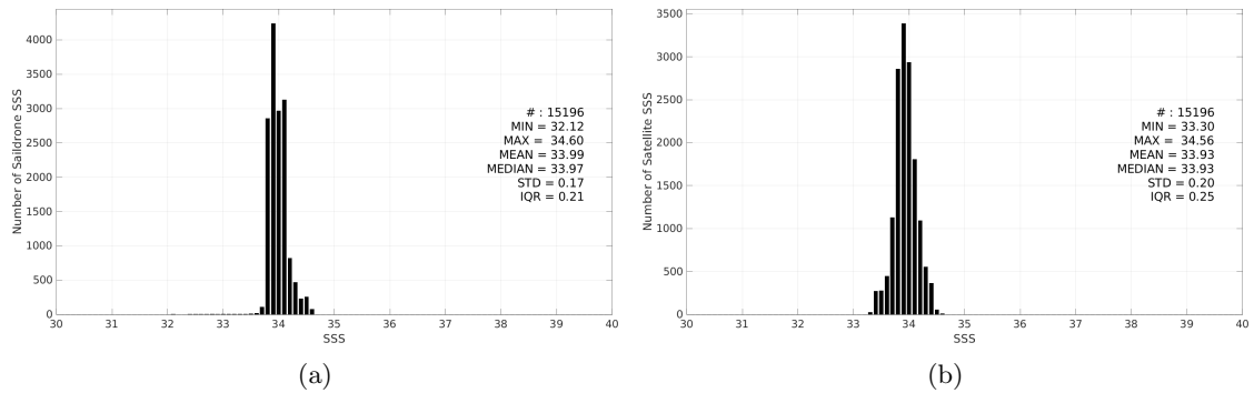
Figure 3: Histograms of SSS from Saildrone (a) and CCI SSS L4 Merged-OI v5.5 - 7-day running (ESA) (b) considering all match-up pairs per bins of 0.1 over the Southern Ocean Pi-MEP region and for the full satellite product period.
