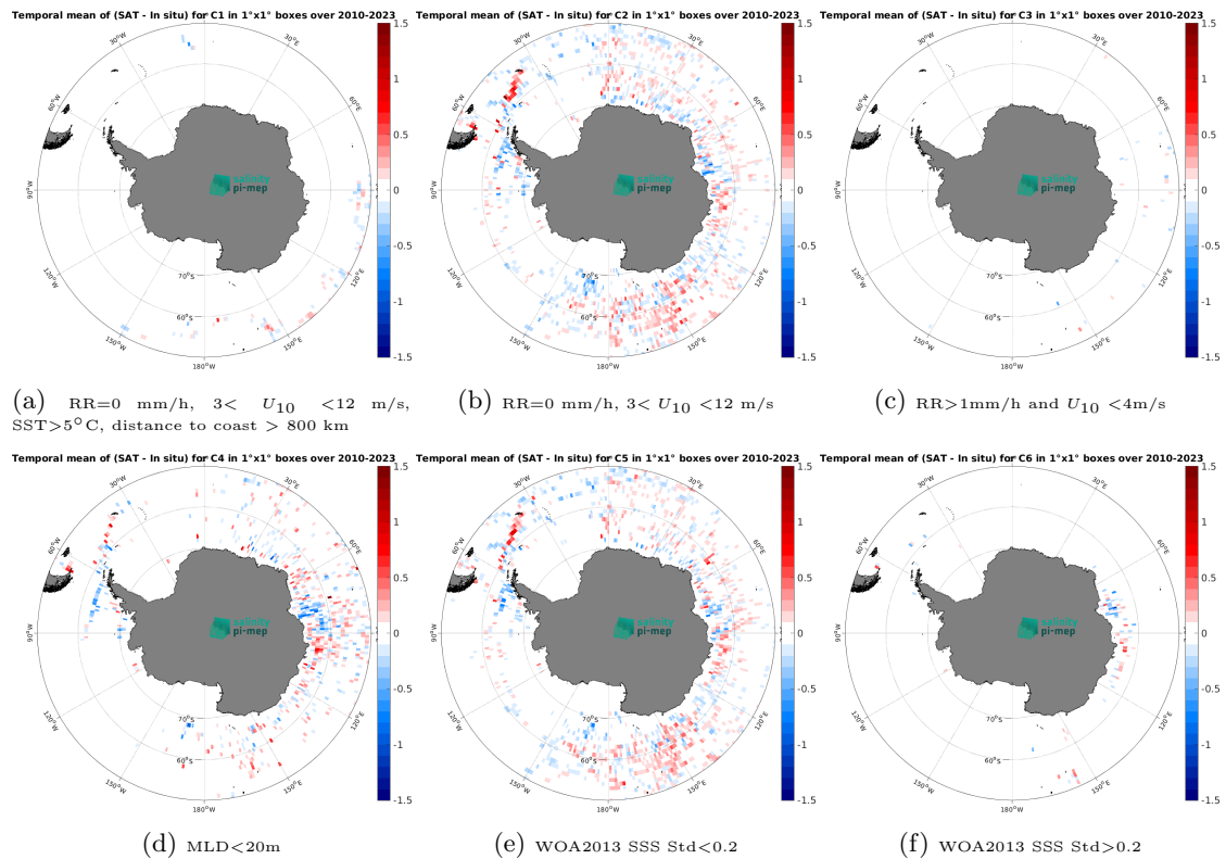
Figure 14: Temporal mean gridded over spatial boxes of size 1^\circ \times 1^\circ of \Delta\text{SSS} (CCI SSS L4 Merged-OI v5.5 - 7-day running (ESA) - Marine mammals) for 6 different subdatasets corresponding to:RR=0 mm/h, 3 < U_{10} < 12 m/s, SST>5°C, distance to coast > 800 km (a), RR=0 mm/h, 3 < U_{10} < 12 m/s (b), RR>1mm/h and U_{10} < 4 m/s (c),MLD<20m (d),WOA2013 SSS Std<0.2 (e),WOA2013 SSS Std>0.2 (f).
