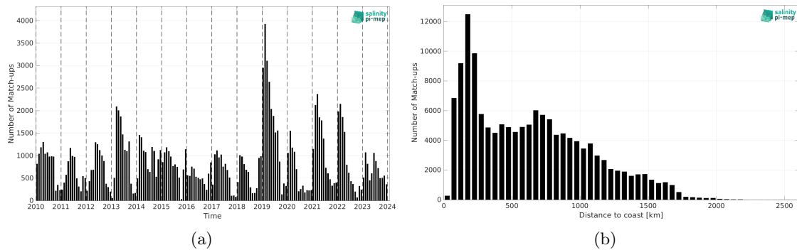
Figure 2: Number of match-ups between Marine mammals and CCI SSS L4 Merged-OI v5.5 - 7-day running (ESA) SSS as a function of time (a) and as function of the distance to coast (b) over the Southern Ocean Pi-MEP region and for the full satellite product period.
