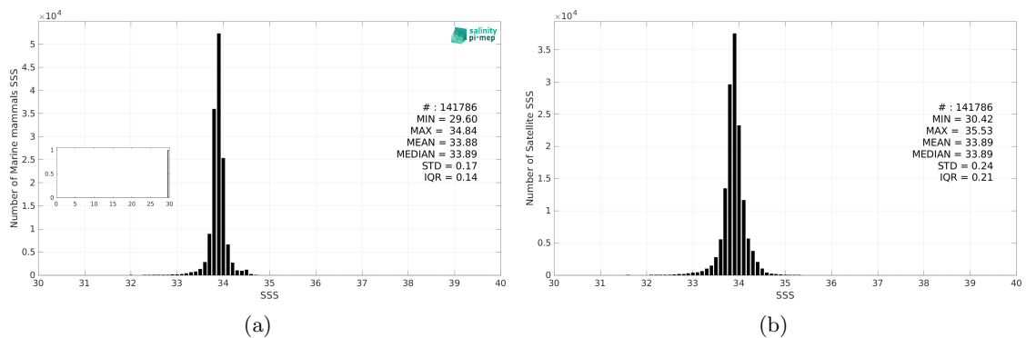
Figure 3: Histograms of SSS from Marine mammals (a) and CCI SSS L4 Merged-OI v5.5 - 7-day running (ESA) (b) considering all match-up pairs per bins of 0.1 over the Southern Ocean Pi-MEP region and for the full satellite product period.
