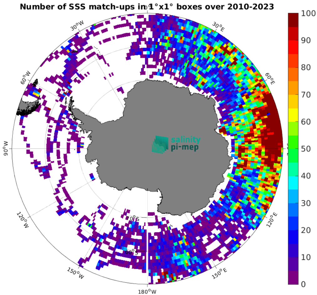
Figure 5: Number of SSS match-ups between Marine mammals SSS and the CCI SSS L4 Merged-OI v5.5 - 7-day running (ESA) SSS product for the Southern Ocean Pi-MEP region over 1^{\circ} \times 1^{\circ} boxes and for the full satellite product period.
