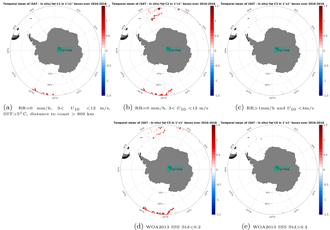
Figure 13: Temporal mean gridded over spatial boxes of size 1^\circ \times 1^\circ of \Delta\text{SSS} (CCI SSS L4 Merged-OI v5.5 - 7-day running (ESA) - Surface drifters) for 5 different subdatasets corresponding to:RR=0 mm/h, 3 < U_{10} < 12 m/s, SST >5^\circ\text{C} , distance to coast > 800 km (a), RR=0 mm/h, 3 < U_{10} < 12 m/s (b), RR >1 mm/h and U_{10} < 4 m/s (c), WOA2013 SSS Std <0.2 (d), WOA2013 SSS Std >0.2 (e).
