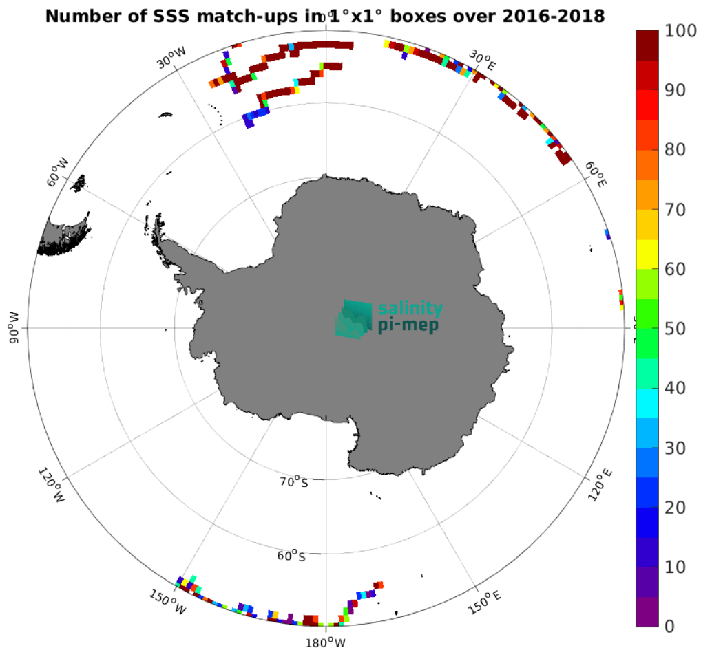
Figure 4: Number of SSS match-ups between Surface drifters SSS and the CCI SSS L4 Merged-OI v5.5 - 7-day running (ESA) SSS product for the Southern Ocean Pi-MEP region over 1^\circ \times 1^\circ boxes and for the full satellite product period.
