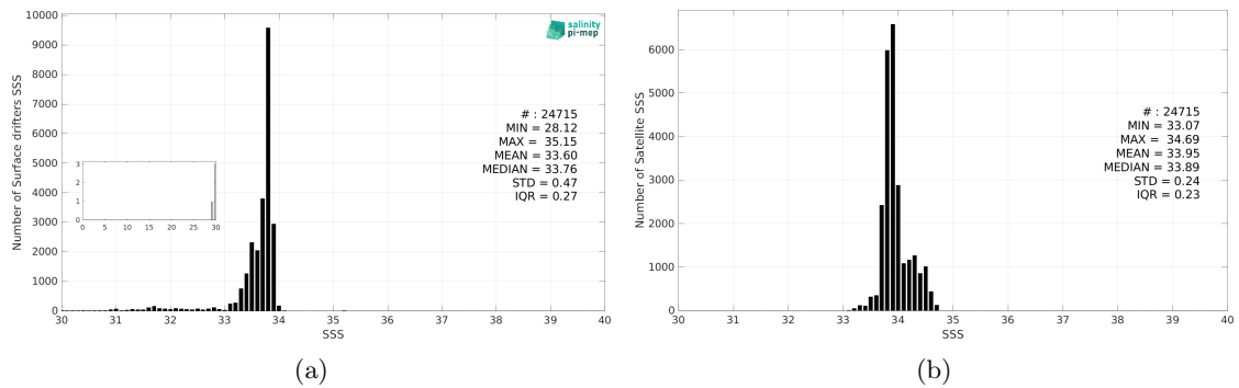
Figure 3: Histograms of SSS from Surface drifters (a) and CCI SSS L4 Merged-OI v5.5 - 7-day running (ESA) (b) considering all match-up pairs per bins of 0.1 over the Southern Ocean Pi-MEP region and for the full satellite product period.
