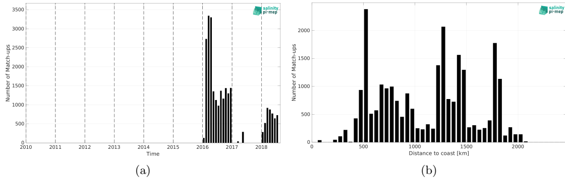
Figure 2: Number of match-ups between Surface drifters and CCI SSS L4 Merged-OI v5.5 - 7-day running (ESA) SSS as a function of time (a) and as function of the distance to coast (b) over the Southern Ocean Pi-MEP region and for the full satellite product period.
