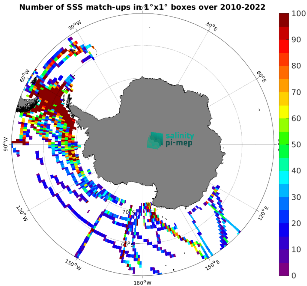
Figure 5: Number of SSS match-ups between TSG (SAMOS) SSS and the CCI SSS L4 Merged-OI v5.5 - 30-day running (ESA) SSS product for the Southern Ocean Pi-MEP region over 1^\circ \times 1^\circ boxes and for the full satellite product period.
