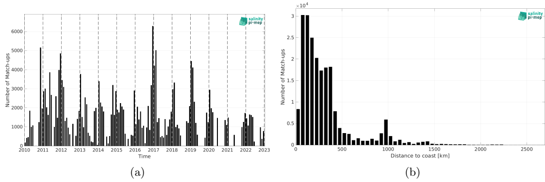
Figure 2: Number of match-ups between TSG (SAMOS) and CCI SSS L4 Merged-OI v5.5 - 30-day running (ESA) SSS as a function of time (a) and as function of the distance to coast (b) over the Southern Ocean Pi-MEP region and for the full satellite product period.
