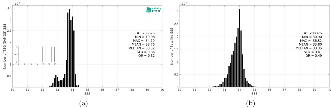
Figure 3: Histograms of SSS from TSG (SAMOS) (a) and CCI SSS L4 Merged-OI v5.5 - 30-day running (ESA) (b) considering all match-up pairs per bins of 0.1 over the Southern Ocean Pi-MEP region and for the full satellite product period.
