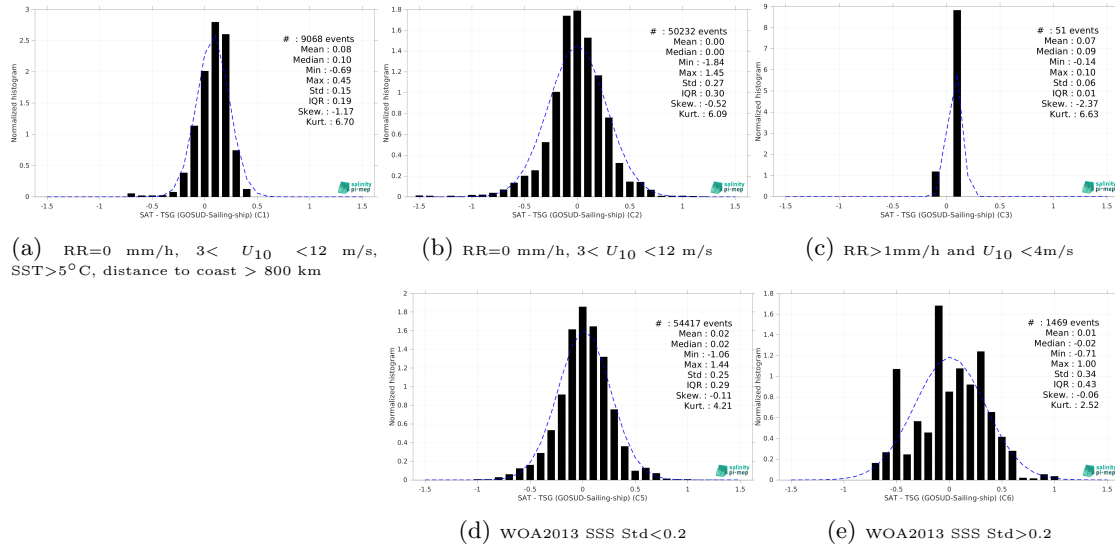
Figure 15: Normalized histogram of \Delta\text{SSS} (CCI SSS L4 Merged-OI v5.5 - 30-day running (ESA) - TSG (GOSUD-Sailing-ship)) for 5 different subdatasets corresponding to: RR=0 mm/h, 3 < U_{10} < 12 m/s, SST>5°C, distance to coast > 800 km (a), RR=0 mm/h, 3 < U_{10} < 12 m/s (b), RR>1mm/h and U_{10} < 4 m/s (c), WOA2013 SSS Std<0.2 (d), WOA2013 SSS Std>0.2 (e).
