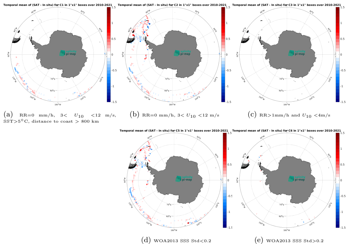
Figure 14: Temporal mean gridded over spatial boxes of size 1^\circ \times 1^\circ of \Delta SSS (CCI SSS L4 Merged-OI v5.5 - 30-day running (ESA) - TSG (GOSUD-Sailing-ship)) for 5 different subdatasets corresponding to:RR=0 mm/h, 3 < U_{10} < 12 m/s, SST >5^\circ\text{C} , distance to coast > 800 km (a), RR=0 mm/h, 3 < U_{10} < 12 m/s (b), RR >1 mm/h and U_{10} < 4 m/s (c), WOA2013 SSS Std <0.2 (d), WOA2013 SSS Std >0.2 (e).
