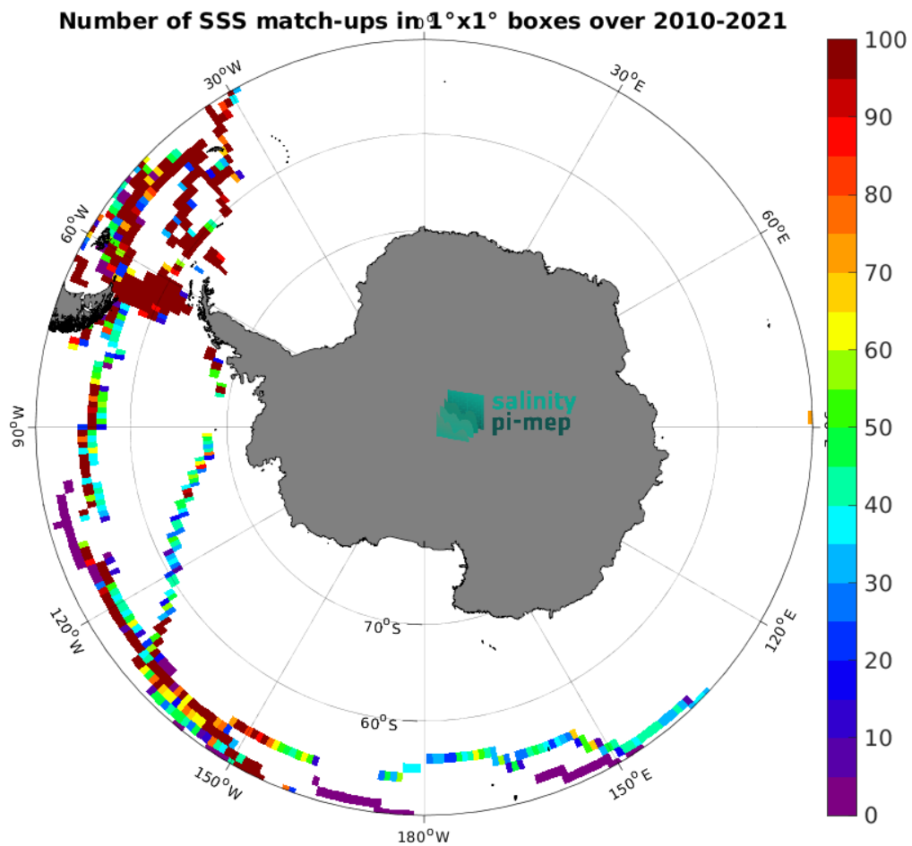
Figure 5: Number of SSS match-ups between TSG (GOSUD-Sailing-ship) SSS and the CCI SSS L4 Merged-OI v5.5 - 30-day running (ESA) SSS product for the Southern Ocean Pi-MEP region over 1^\circ \times 1^\circ boxes and for the full satellite product period.
