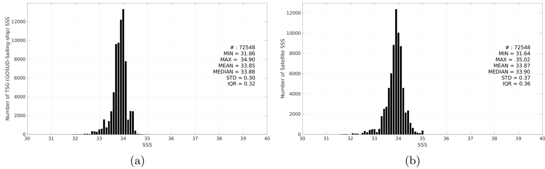
Figure 3: Histograms of SSS from TSG (GOSUD-Sailing-ship) (a) and CCI SSS L4 Merged-OI v5.5 - 30-day running (ESA) (b) considering all match-up pairs per bins of 0.1 over the Southern Ocean Pi-MEP region and for the full satellite product period.
