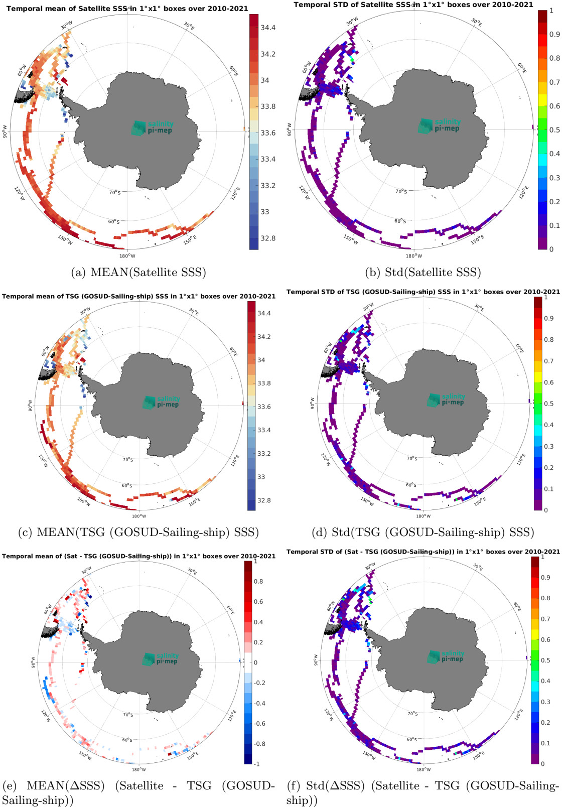
Figure 7: Temporal mean (left) and Std (right) of SSS from CCI SSS L4 Merged-OI v5.5 - 30-day running (ESA) (top), TSG (GOSUD-Sailing-ship) (middle), and of \Delta SSS (Satellite - TSG (GOSUD-Sailing-ship)). Only match-up pairs are used to generate these maps.
