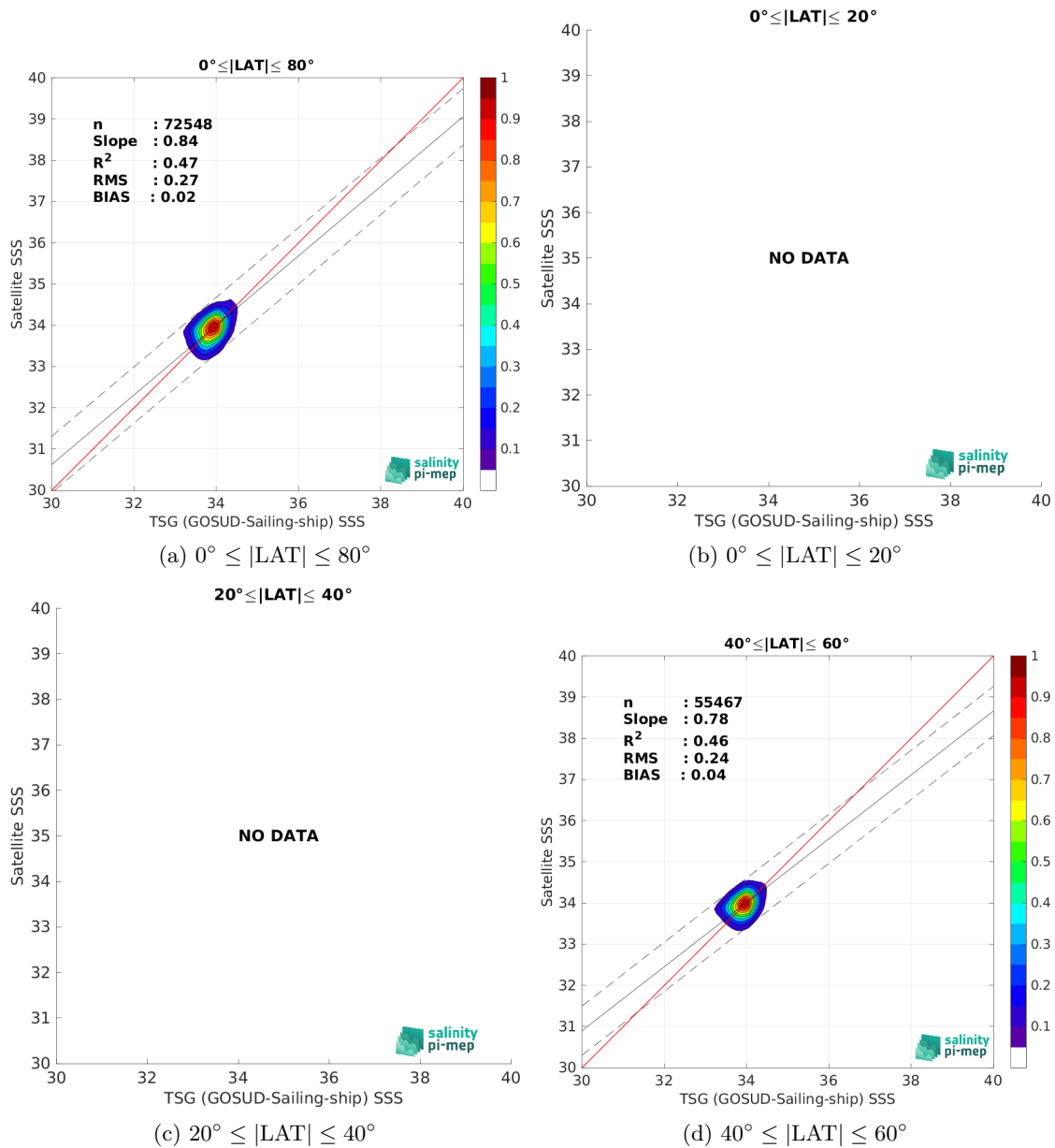
Figure 10: Contour maps of the concentration of CCI SSS L4 Merged-OI v5.5 - 30-day running (ESA) SSS (y-axis) versus TSG (GOSUD-Sailing-ship) SSS (x-axis) at match-up pairs for different latitude bands. For each plot, the red line shows x=y . The black thin and dashed lines indicate a linear fit through the data cloud and the \pm 95\% confidence levels, respectively. The number match-up pairs n , the slope and R^2 coefficient of the linear fit, the root mean square (RMS) and the mean bias between satellite and in situ data are indicated for each latitude band in each plots.
