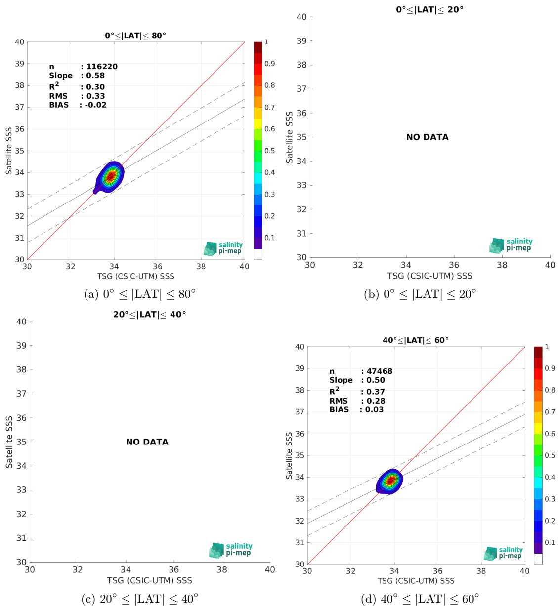
Figure 10: Contour maps of the concentration of CCI SSS L4 Merged-OI v5.5 - 30-day running (ESA) SSS (y-axis) versus TSG (CSIC-UTM) SSS (x-axis) at match-up pairs for different latitude bands. For each plot, the red line shows x=y . The black thin and dashed lines indicate a linear fit through the data cloud and the \pm 95\% confidence levels, respectively. The number match-up pairs n , the slope and R^2 coefficient of the linear fit, the root mean square (RMS) and the mean bias between satellite and in situ data are indicated for each latitude band in each plots.
