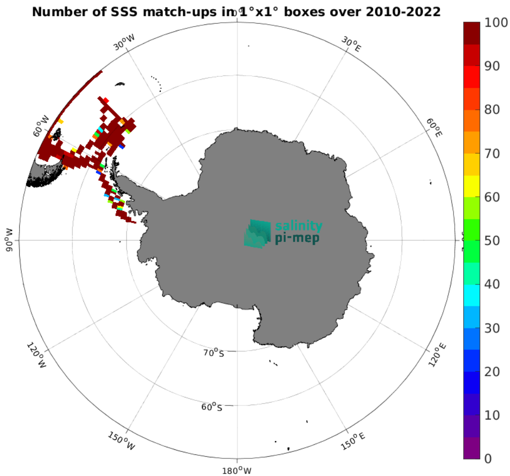
Figure 5: Number of SSS match-ups between TSG (CSIC-UTM) SSS and the CCI SSS L4 Merged-OI v5.5 - 30-day running (ESA) SSS product for the Southern Ocean Pi-MEP region over 1^{\circ} \times 1^{\circ} boxes and for the full satellite product period.
