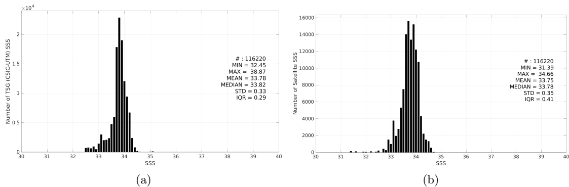
Figure 3: Histograms of SSS from TSG (CSIC-UTM) (a) and CCI SSS L4 Merged-OI v5.5 - 30-day running (ESA) (b) considering all match-up pairs per bins of 0.1 over the Southern Ocean Pi-MEP region and for the full satellite product period.
