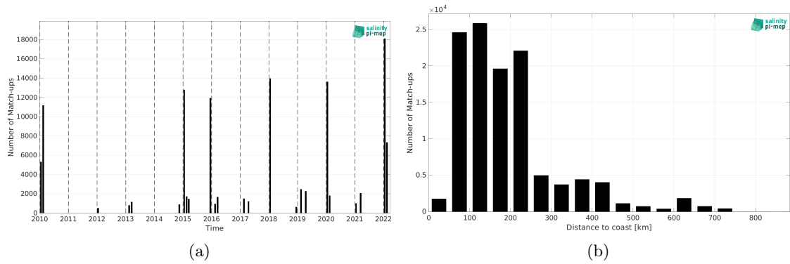
Figure 2: Number of match-ups between TSG (CSIC-UTM) and CCI SSS L4 Merged-OI v5.5 - 30-day running (ESA) SSS as a function of time (a) and as function of the distance to coast (b) over the Southern Ocean Pi-MEP region and for the full satellite product period.
