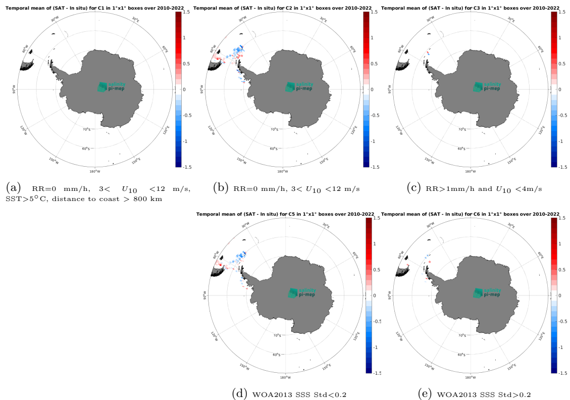
Figure 14: Temporal mean gridded over spatial boxes of size 1^\circ \times 1^\circ of \Delta\text{SSS} (CCI SSS L4 Merged-OI v5.5 - 30-day running (ESA) - TSG (CSIC-UTM)) for 5 different subdatasets corresponding to:RR=0 mm/h, 3 < U_{10} < 12 m/s, SST>5°C, distance to coast > 800 km (a), RR=0 mm/h, 3 < U_{10} < 12 m/s (b), RR>1mm/h and U_{10} < 4 m/s (c), WOA2013 SSS Std<0.2 (d), WOA2013 SSS Std>0.2 (e).
