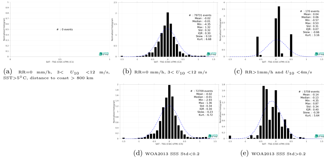
Figure 15: Normalized histogram of \Delta SSS (CCI SSS L4 Merged-OI v5.5 - 30-day running (ESA) - TSG (CSIC-UTM)) for 5 different subdatasets corresponding to: RR=0 mm/h, 3 < U_{10} < 12 m/s, SST > 5°C, distance to coast > 800 km (a), RR=0 mm/h, 3 < U_{10} < 12 m/s (b), RR > 1mm/h and U_{10} < 4 m/s (c), WOA2013 SSS Std < 0.2 (d), WOA2013 SSS Std > 0.2 (e).
