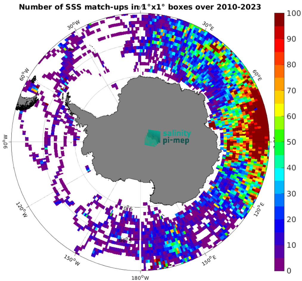
Figure 5: Number of SSS match-ups between Marine mammals SSS and the CCI SSS L4 Merged-OI v5.5 - 30-day running (ESA) SSS product for the Southern Ocean Pi-MEP region over 1^\circ \times 1^\circ boxes and for the full satellite product period.
