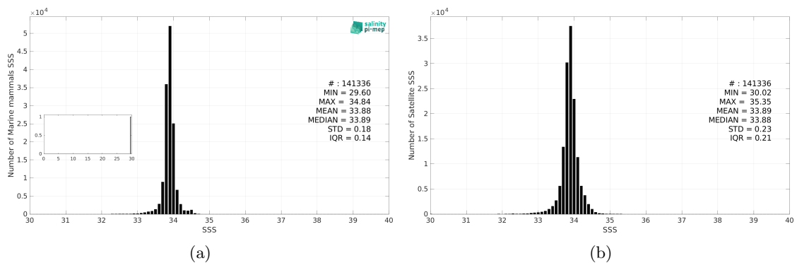
Figure 3: Histograms of SSS from Marine mammals (a) and CCI SSS L4 Merged-OI v5.5 - 30-day running (ESA) (b) considering all match-up pairs per bins of 0.1 over the Southern Ocean Pi-MEP region and for the full satellite product period.
