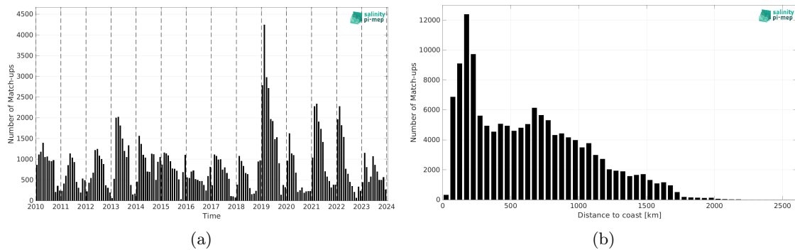
Figure 2: Number of match-ups between Marine mammals and CCI SSS L4 Merged-OI v5.5 - 30-day running (ESA) SSS as a function of time (a) and as function of the distance to coast (b) over the Southern Ocean Pi-MEP region and for the full satellite product period.
