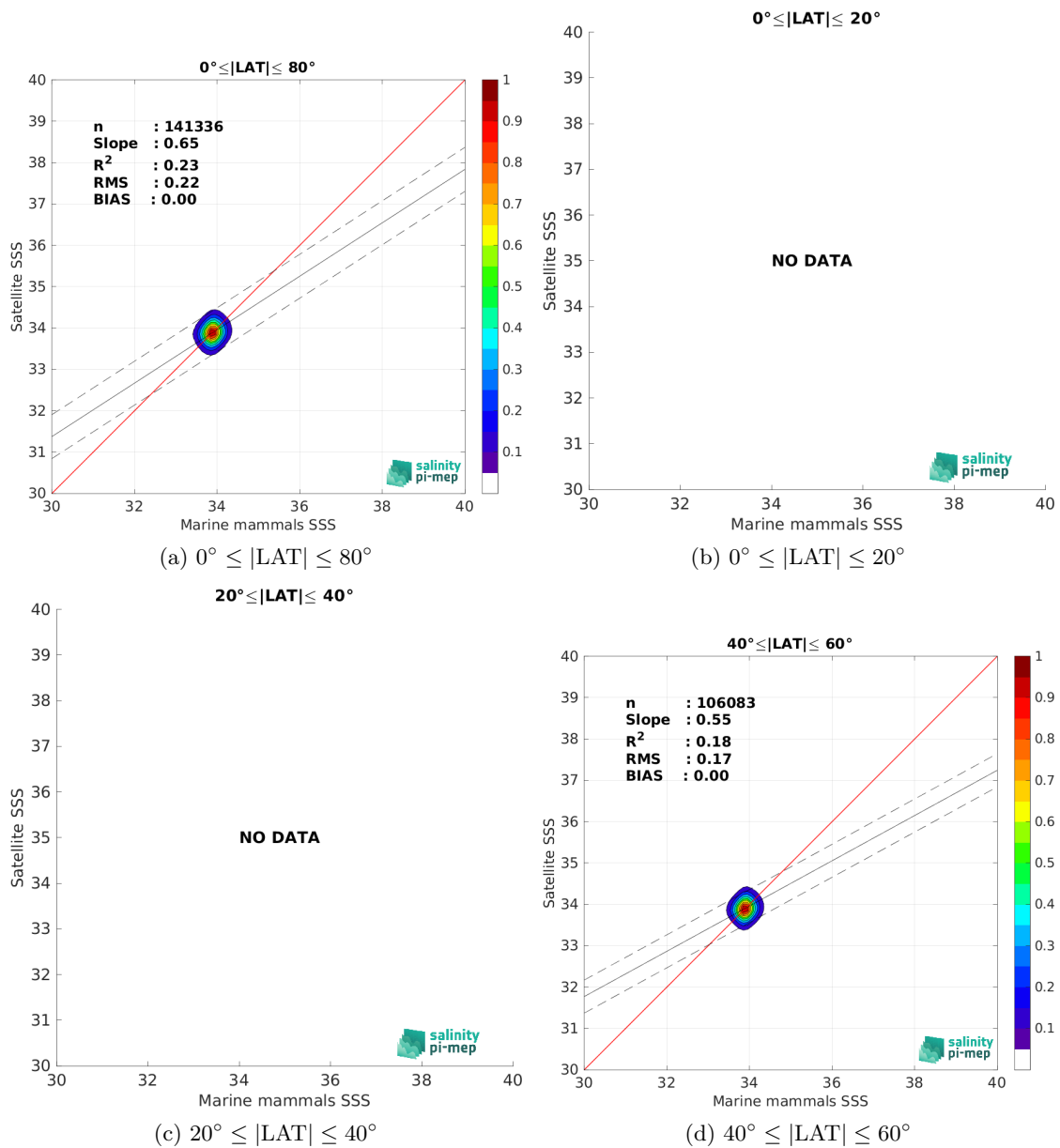
Figure 10: Contour maps of the concentration of CCI SSS L4 Merged-OI v5.5 - 30-day running (ESA) SSS (y-axis) versus Marine mammals SSS (x-axis) at match-up pairs for different latitude bands. For each plot, the red line shows x=y . The black thin and dashed lines indicate a linear fit through the data cloud and the \pm 95\% confidence levels, respectively. The number match-up pairs n , the slope and R^2 coefficient of the linear fit, the root mean square (RMS) and the mean bias between satellite and in situ data are indicated for each latitude band in each plots.
