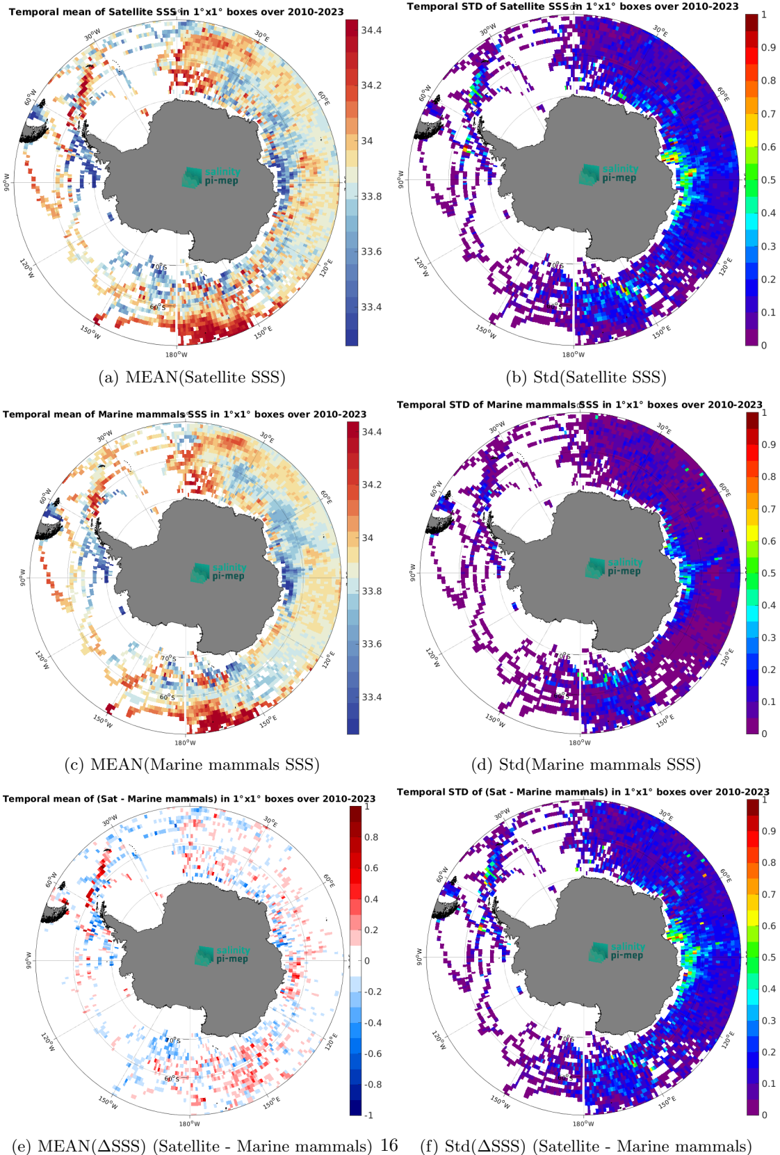
Figure 7: Temporal mean (left) and Std (right) of SSS from CCI SSS L4 Merged-OI v5.5 - 30-day running (ESA) (top), Marine mammals (middle), and of \Delta SSS (Satellite - Marine mammals). Only match-up pairs are used to generate these maps.
