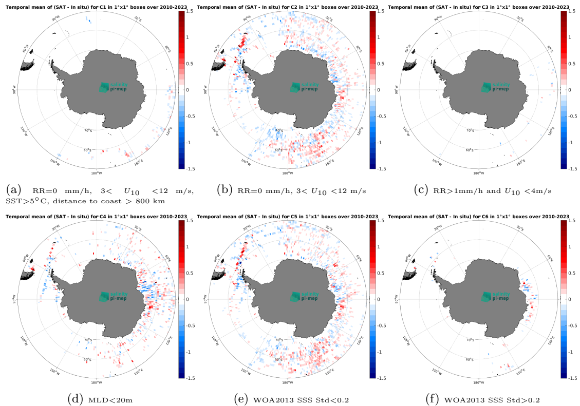
Figure 14: Temporal mean gridded over spatial boxes of size 1^\circ \times 1^\circ of \Delta\text{SSS} (CCI SSS L4 Merged-OI v5.5 - 30-day running (ESA) - Marine mammals) for 6 different subdatasets corresponding to:RR=0 mm/h, 3 < U_{10} < 12 m/s, SST>5°C, distance to coast > 800 km (a), RR=0 mm/h, 3 < U_{10} < 12 m/s (b), RR>1mm/h and U_{10} < 4 m/s (c),MLD<20m (d),WOA2013 SSS Std<0.2 (e),WOA2013 SSS Std>0.2 (f).
