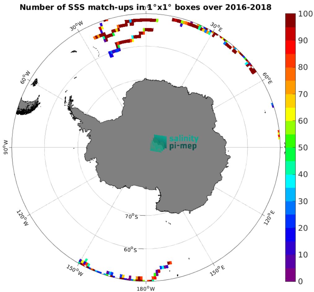
Figure 4: Number of SSS match-ups between Surface drifters SSS and the CCI SSS L4 Merged-OI v5.5 - 30-day running (ESA) SSS product for the Southern Ocean Pi-MEP region over 1^\circ \times 1^\circ boxes and for the full satellite product period.
