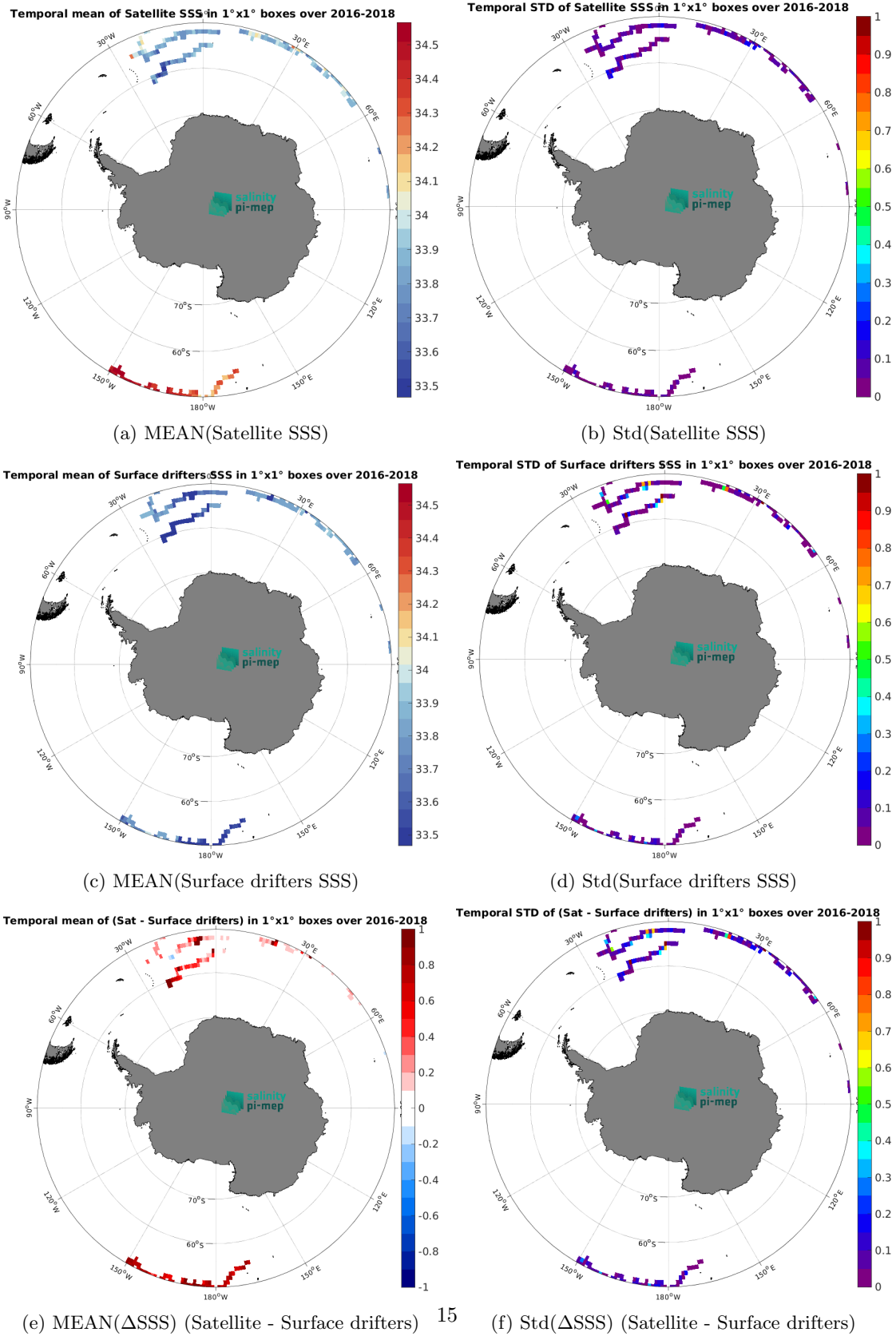
Figure 6: Temporal mean (left) and Std (right) of SSS from CCI SSS L4 Merged-OI v5.5 - 30-day running (ESA) (top), Surface drifters (middle), and of \Delta SSS (Satellite - Surface drifters). Only match-up pairs are used to generate these maps.
