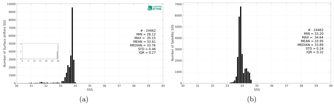
Figure 3: Histograms of SSS from Surface drifters (a) and CCI SSS L4 Merged-OI v5.5 - 30-day running (ESA) (b) considering all match-up pairs per bins of 0.1 over the Southern Ocean Pi-MEP region and for the full satellite product period.
