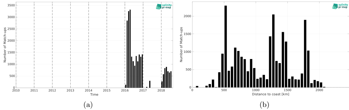
Figure 2: Number of match-ups between Surface drifters and CCI SSS L4 Merged-OI v5.5 - 30-day running (ESA) SSS as a function of time (a) and as function of the distance to coast (b) over the Southern Ocean Pi-MEP region and for the full satellite product period.
