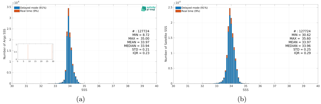
Figure 3: Histograms of SSS from Argo (a) and CCI SSS L4 Merged-OI v5.5 - 30-day running (ESA) (b) considering all match-up pairs per bins of 0.1 over the Southern Ocean Pi-MEP region and for the full satellite product period.
