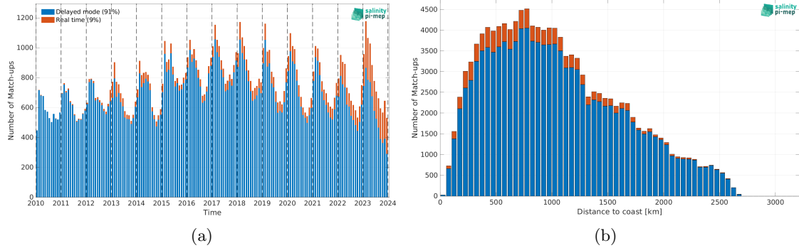
Figure 2: Number of match-ups between Argo and CCI SSS L4 Merged-OI v5.5 - 30-day running (ESA) SSS as a function of time (a) and as function of the distance to coast (b) over the Southern Ocean Pi-MEP region and for the full satellite product period.
