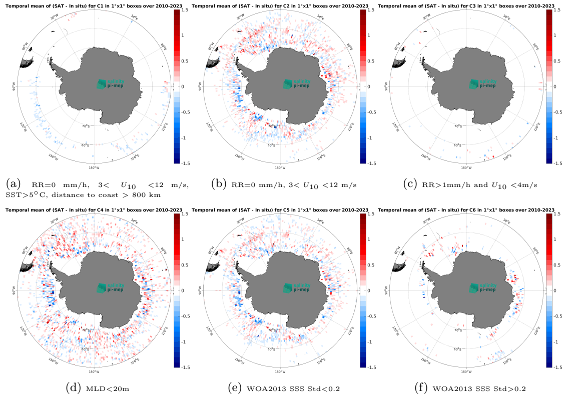
Figure 14: Temporal mean gridded over spatial boxes of size 1^\circ \times 1^\circ of \Delta\text{SSS} (CCI SSS L4 Merged-OI v5.5 - 30-day running (ESA) - Argo) for 6 different subdatasets corresponding to:RR=0 mm/h, 3 < U_{10} < 12 m/s, SST>5°C, distance to coast > 800 km (a), RR=0 mm/h, 3 < U_{10} < 12 m/s (b), RR>1mm/h and U_{10} < 4 m/s (c),MLD<20m (d),WOA2013 SSS Std<0.2 (e),WOA2013 SSS Std>0.2 (f).
