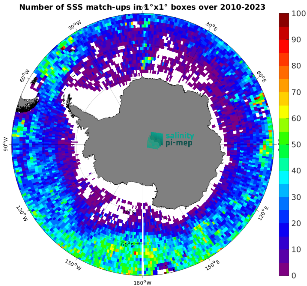
Figure 5: Number of SSS match-ups between Argo SSS and the CCI SSS L4 Merged-OI v5.5 - 30-day running (ESA) SSS product for the Southern Ocean Pi-MEP region over 1^\circ \times 1^\circ boxes and for the full satellite product period.
