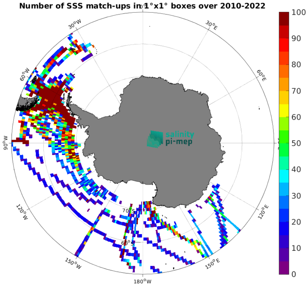
Figure 5: Number of SSS match-ups between TSG (SAMOS) SSS and the CCI SSS L4 Merged-OI v4.41 - 7-day running (ESA) SSS product for the Southern Ocean Pi-MEP region over 1^\circ \times 1^\circ boxes and for the full satellite product period.
