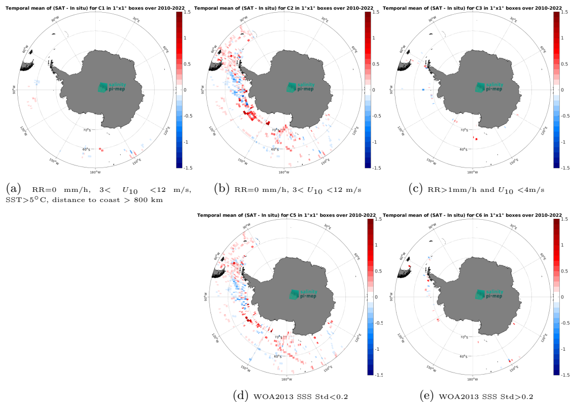
Figure 14: Temporal mean gridded over spatial boxes of size 1^\circ \times 1^\circ of \Delta SSS (CCI SSS L4 Merged-OI v4.41 - 7-day running (ESA) - TSG (SAMOS)) for 5 different subdatasets corresponding to:RR=0 mm/h, 3 < U_{10} < 12 m/s, SST > 5^\circ\text{C} , distance to coast > 800 km (a), RR=0 mm/h, 3 < U_{10} < 12 m/s (b), RR > 1 mm/h and U_{10} < 4 m/s (c), WOA2013 SSS Std < 0.2 (d), WOA2013 SSS Std > 0.2 (e).
