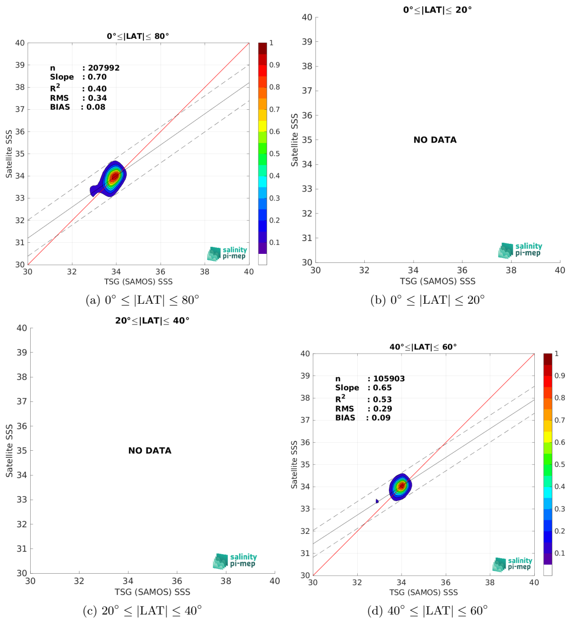
Figure 10: Contour maps of the concentration of CCI SSS L4 Merged-OI v4.41 - 7-day running (ESA) SSS (y-axis) versus TSG (SAMOS) SSS (x-axis) at match-up pairs for different latitude bands. For each plot, the red line shows x=y . The black thin and dashed lines indicate a linear fit through the data cloud and the \pm 95\% confidence levels, respectively. The number match-up pairs n , the slope and R^2 coefficient of the linear fit, the root mean square (RMS) and the mean bias between satellite and in situ data are indicated for each latitude band in each plots.
