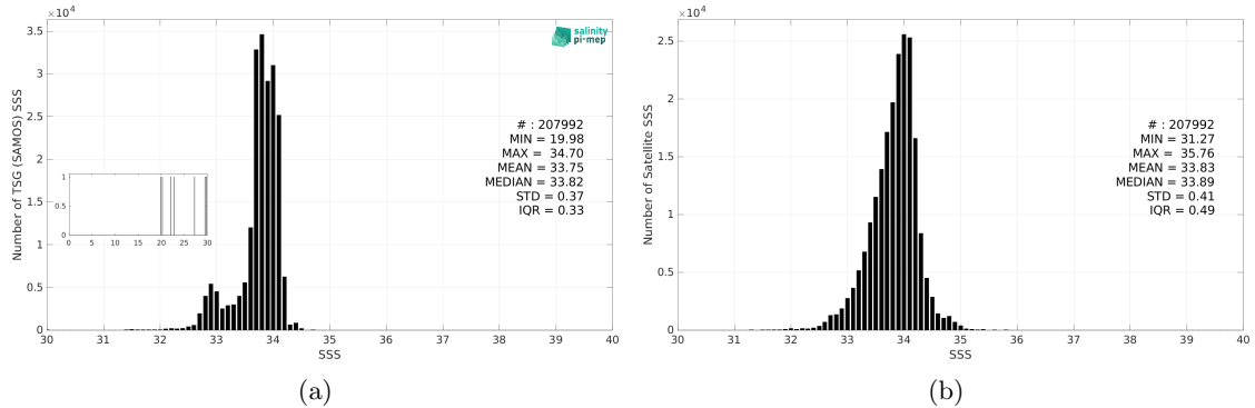
Figure 3: Histograms of SSS from TSG (SAMOS) (a) and CCI SSS L4 Merged-OI v4.41 - 7-day running (ESA) (b) considering all match-up pairs per bins of 0.1 over the Southern Ocean Pi-MEP region and for the full satellite product period.
