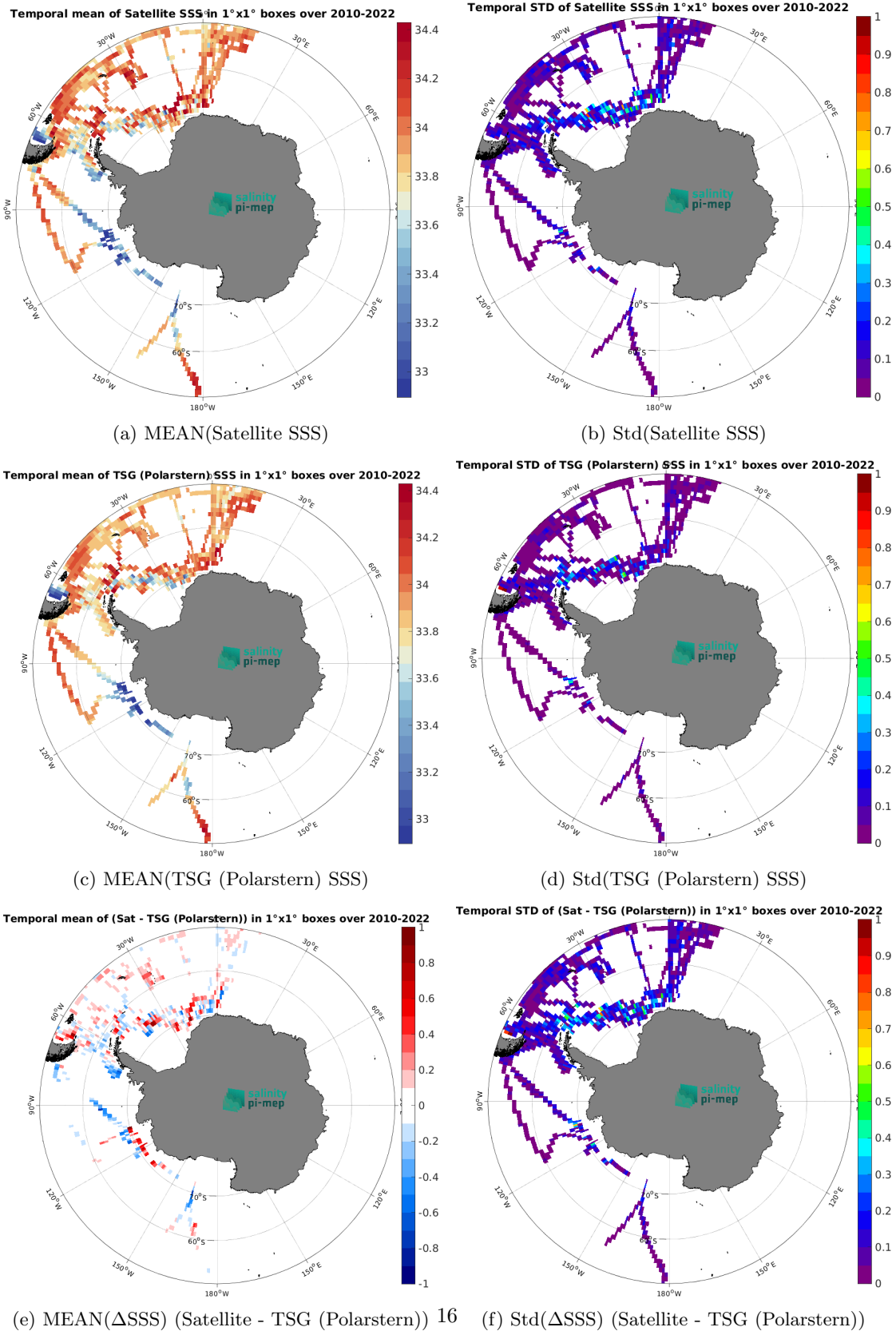
Figure 7: Temporal mean (left) and Std (right) of SSS from CCI SSS L4 Merged-OI v4.41 - 7-day running (ESA) (top), TSG (Polarstern) (middle), and of \Delta SSS (Satellite - TSG (Polarstern)). Only match-up pairs are used to generate these maps.
