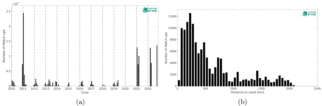
Figure 2: Number of match-ups between TSG (Polarstern) and CCI SSS L4 Merged-OI v4.41 - 7-day running (ESA) SSS as a function of time (a) and as function of the distance to coast (b) over the Southern Ocean Pi-MEP region and for the full satellite product period.
