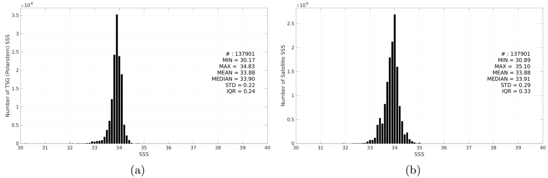
Figure 3: Histograms of SSS from TSG (Polarstern) (a) and CCI SSS L4 Merged-OI v4.41 - 7-day running (ESA) (b) considering all match-up pairs per bins of 0.1 over the Southern Ocean Pi-MEP region and for the full satellite product period.
