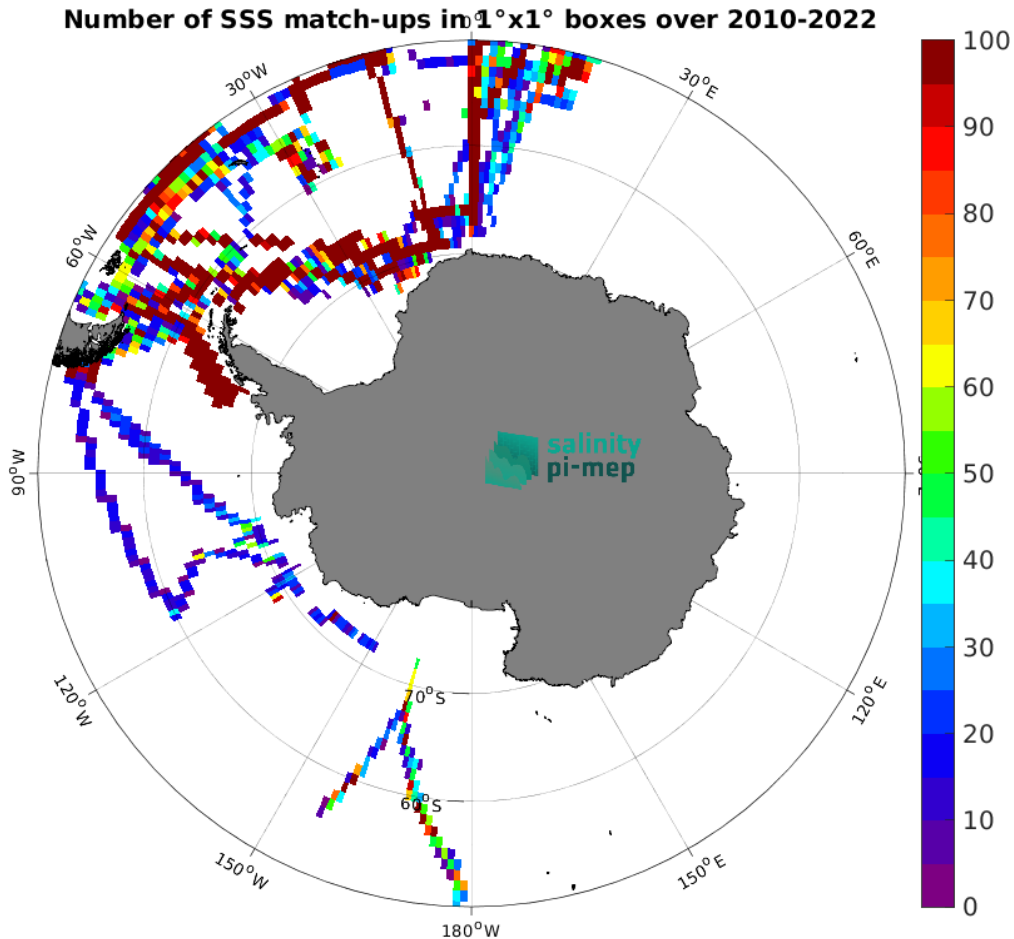
Figure 5: Number of SSS match-ups between TSG (Polarstern) SSS and the CCI SSS L4 Merged-OI v4.41 - 7-day running (ESA) SSS product for the Southern Ocean Pi-MEP region over 1^\circ \times 1^\circ boxes and for the full satellite product period.
