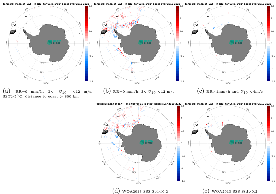
Figure 14: Temporal mean gridded over spatial boxes of size 1^\circ \times 1^\circ of \Delta\text{SSS} (CCI SSS L4 Merged-OI v4.41 - 7-day running (ESA) - TSG (Polarstern)) for 5 different subdatasets corresponding to:RR=0 mm/h, 3 < U_{10} < 12 m/s, SST>5°C, distance to coast > 800 km (a), RR=0 mm/h, 3 < U_{10} < 12 m/s (b), RR>1mm/h and U_{10} < 4 m/s (c), WOA2013 SSS Std<0.2 (d), WOA2013 SSS Std>0.2 (e).
