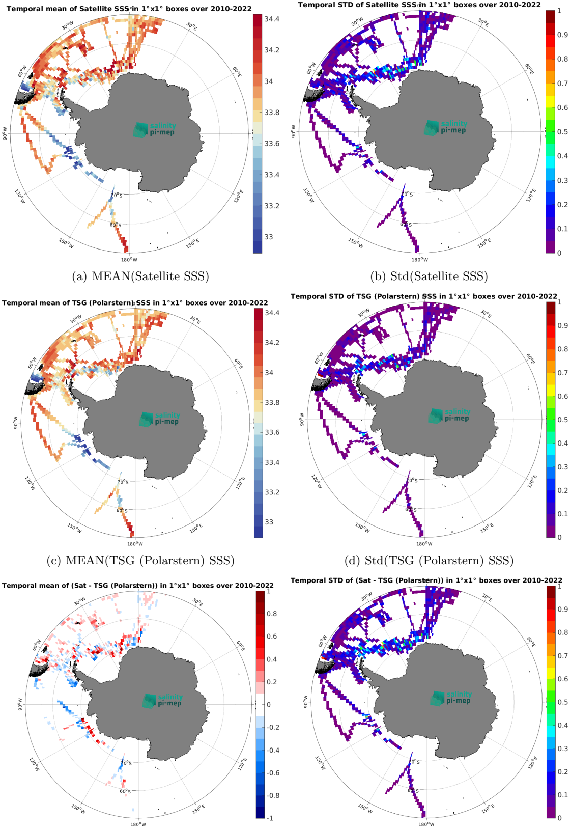
Figure 7: Temporal mean (left) and Std (right) of SSS from CCI SSS L4 Merged-OI v4.41 - 7-day running (ESA) (top), TSG (Polarstern) (middle), and of \Delta SSS (Satellite - TSG (Polarstern)). Only match-up pairs are used to generate these maps.
