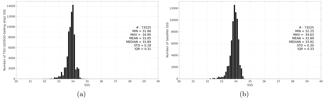
Figure 3: Histograms of SSS from TSG (GOSUD-Sailing-ship) (a) and CCI SSS L4 Merged-OI v4.41 - 7-day running (ESA) (b) considering all match-up pairs per bins of 0.1 over the Southern Ocean Pi-MEP region and for the full satellite product period.
