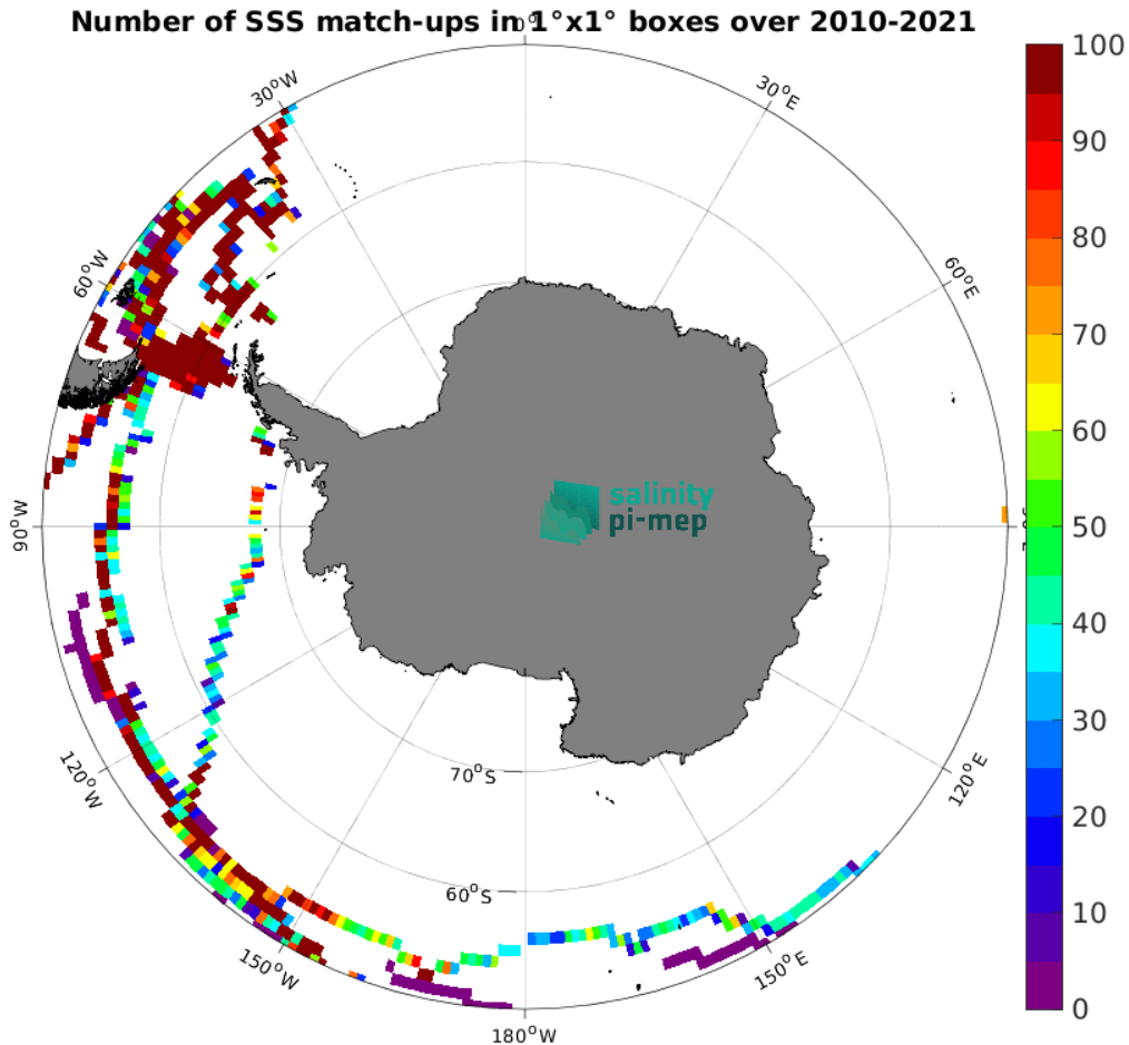
Figure 5: Number of SSS match-ups between TSG (GOSUD-Sailing-ship) SSS and the CCI SSS L4 Merged-OI v4.41 - 7-day running (ESA) SSS product for the Southern Ocean Pi-MEP region over 1^\circ \times 1^\circ boxes and for the full satellite product period.
