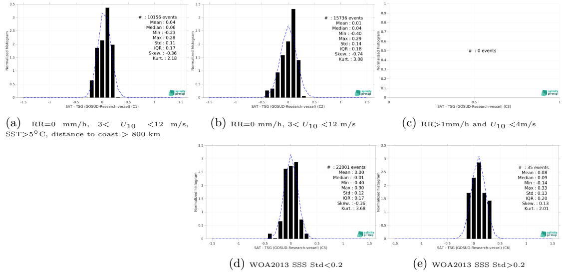
Figure 15: Normalized histogram of \Delta SSS (CCI SSS L4 Merged-OI v4.41 - 7-day running (ESA) - TSG (GOSUD-Research-vessel)) for 5 different subdatasets corresponding to: RR=0 mm/h, 3 < U_{10} < 12 m/s, SST > 5°C, distance to coast > 800 km (a), RR=0 mm/h, 3 < U_{10} < 12 m/s (b), RR > 1mm/h and U_{10} < 4 m/s (c), WOA2013 SSS Std < 0.2 (d), WOA2013 SSS Std > 0.2 (e).
