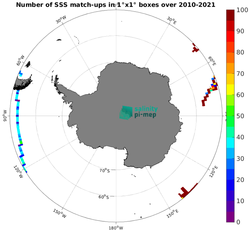
Figure 5: Number of SSS match-ups between TSG (GOSUD-Research-vessel) SSS and the CCI SSS L4 Merged-OI v4.41 - 7-day running (ESA) SSS product for the Southern Ocean Pi-MEP region over 1^\circ \times 1^\circ boxes and for the full satellite product period.
