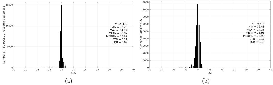
Figure 3: Histograms of SSS from TSG (GOSUD-Research-vessel) (a) and CCI SSS L4 Merged-OI v4.41 - 7-day running (ESA) (b) considering all match-up pairs per bins of 0.1 over the Southern Ocean Pi-MEP region and for the full satellite product period.
