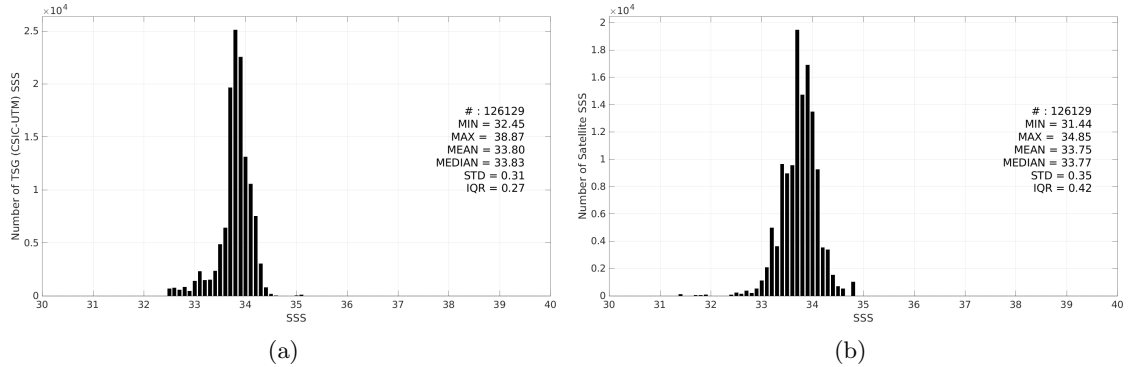
Figure 3: Histograms of SSS from TSG (CSIC-UTM) (a) and CCI SSS L4 Merged-OI v4.41 - 7-day running (ESA) (b) considering all match-up pairs per bins of 0.1 over the Southern Ocean Pi-MEP region and for the full satellite product period.
