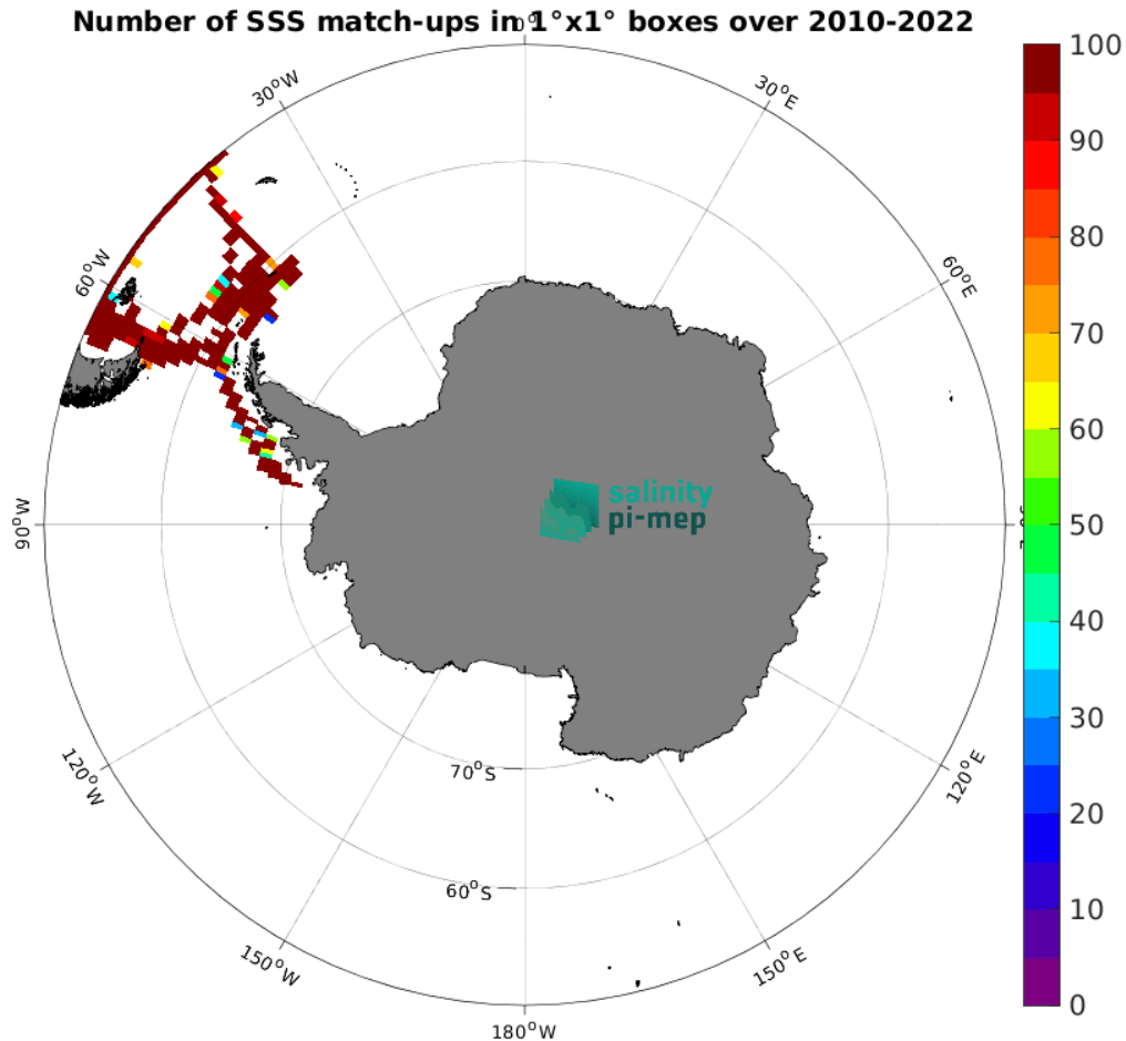
Figure 5: Number of SSS match-ups between TSG (CSIC-UTM) SSS and the CCI SSS L4 Merged-OI v4.41 - 7-day running (ESA) SSS product for the Southern Ocean Pi-MEP region over 1^\circ \times 1^\circ boxes and for the full satellite product period.
