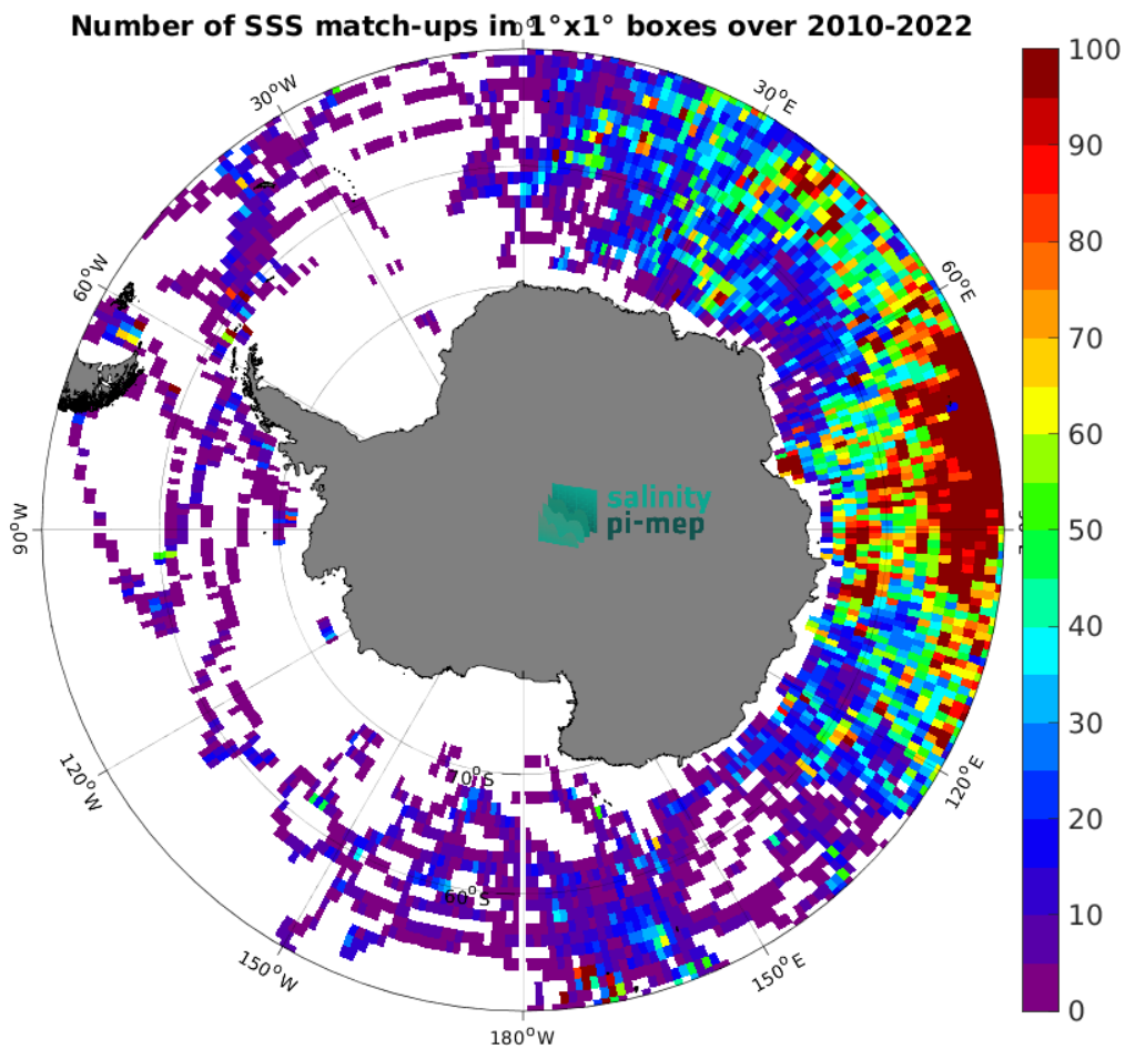
Figure 5: Number of SSS match-ups between Marine mammals SSS and the CCI SSS L4 Merged-OI v4.41 - 7-day running (ESA) SSS product for the Southern Ocean Pi-MEP region over 1^\circ \times 1^\circ boxes and for the full satellite product period.
