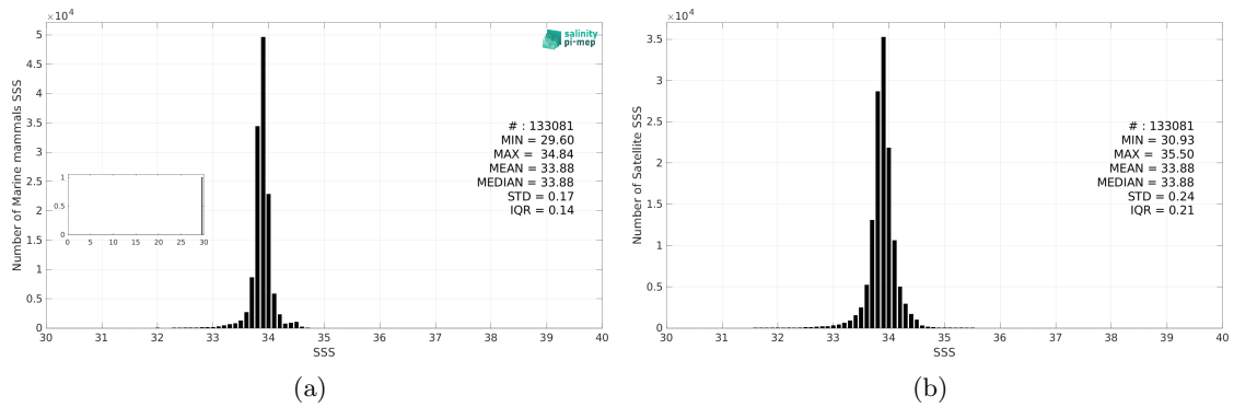
Figure 3: Histograms of SSS from Marine mammals (a) and CCI SSS L4 Merged-OI v4.41 - 7-day running (ESA) (b) considering all match-up pairs per bins of 0.1 over the Southern Ocean Pi-MEP region and for the full satellite product period.
