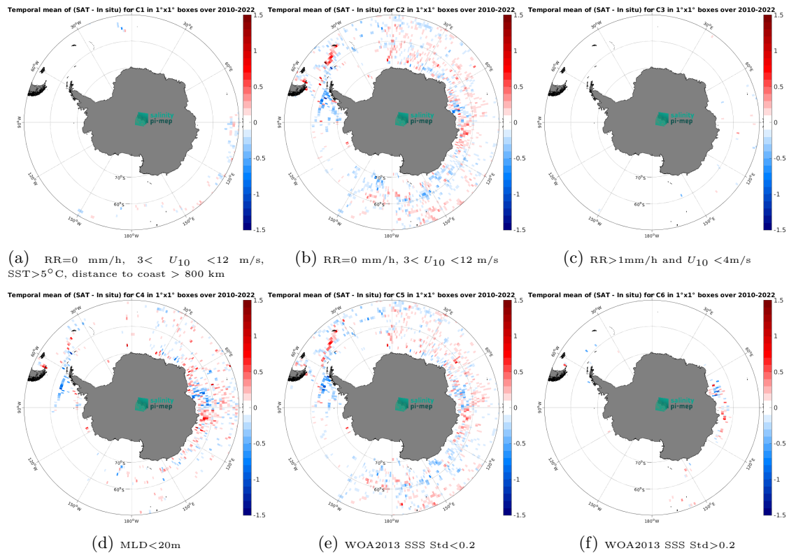
Figure 14: Temporal mean gridded over spatial boxes of size 1^\circ \times 1^\circ of \Delta\text{SSS} (CCI SSS L4 Merged-OI v4.41 - 7-day running (ESA) - Marine mammals) for 6 different subdatasets corresponding to:RR=0 mm/h, 3 < U_{10} < 12 m/s, SST>5°C, distance to coast > 800 km (a), RR=0 mm/h, 3 < U_{10} < 12 m/s (b), RR>1mm/h and U_{10} < 4 m/s (c),MLD<20m (d),WOA2013 SSS Std<0.2 (e),WOA2013 SSS Std>0.2 (f).
