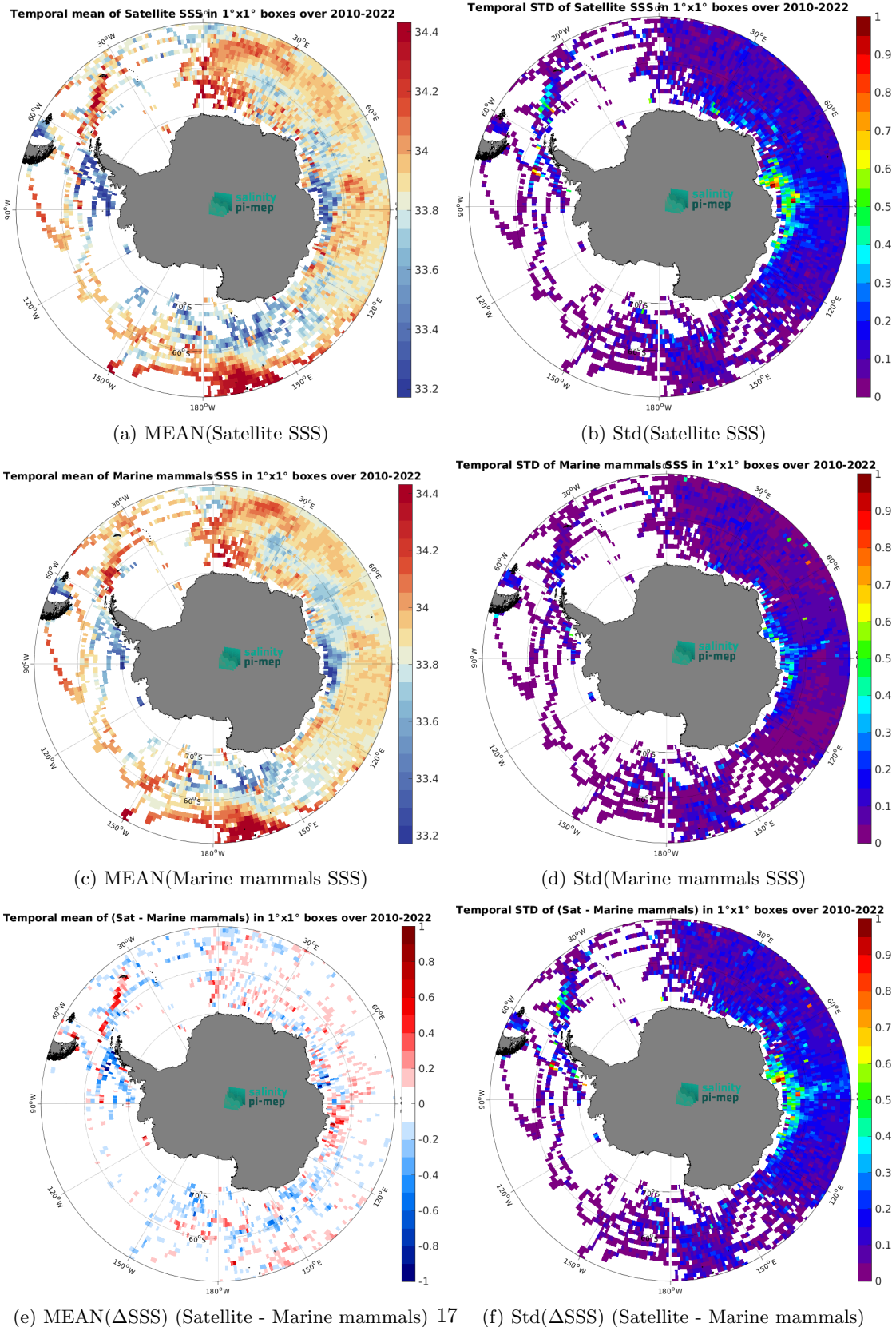
Figure 7: Temporal mean (left) and Std (right) of SSS from CCI SSS L4 Merged-OI v4.41 - 7-day running (ESA) (top), Marine mammals (middle), and of \Delta SSS (Satellite - Marine mammals). Only match-up pairs are used to generate these maps.
