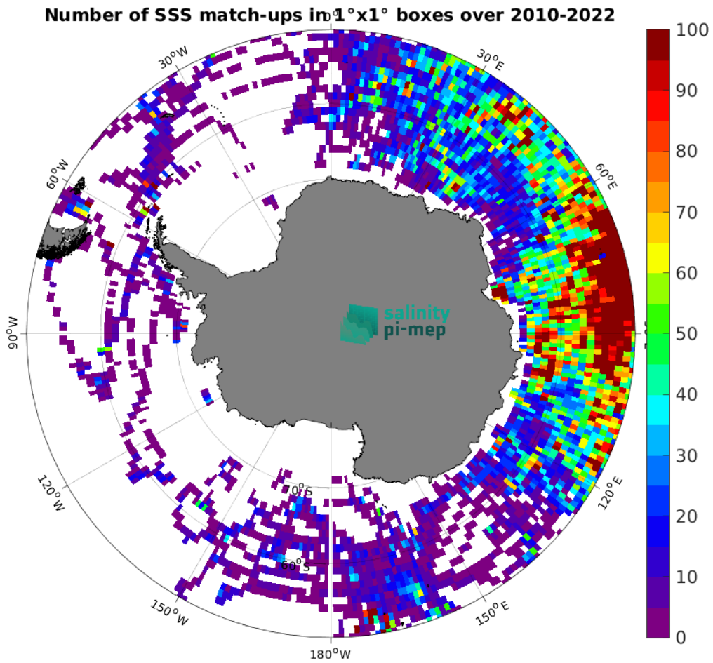
Figure 5: Number of SSS match-ups between Marine mammals SSS and the CCI SSS L4 Merged-OI v4.41 - 7-day running (ESA) SSS product for the Southern Ocean Pi-MEP region over 1^{\circ} \times 1^{\circ} boxes and for the full satellite product period.
