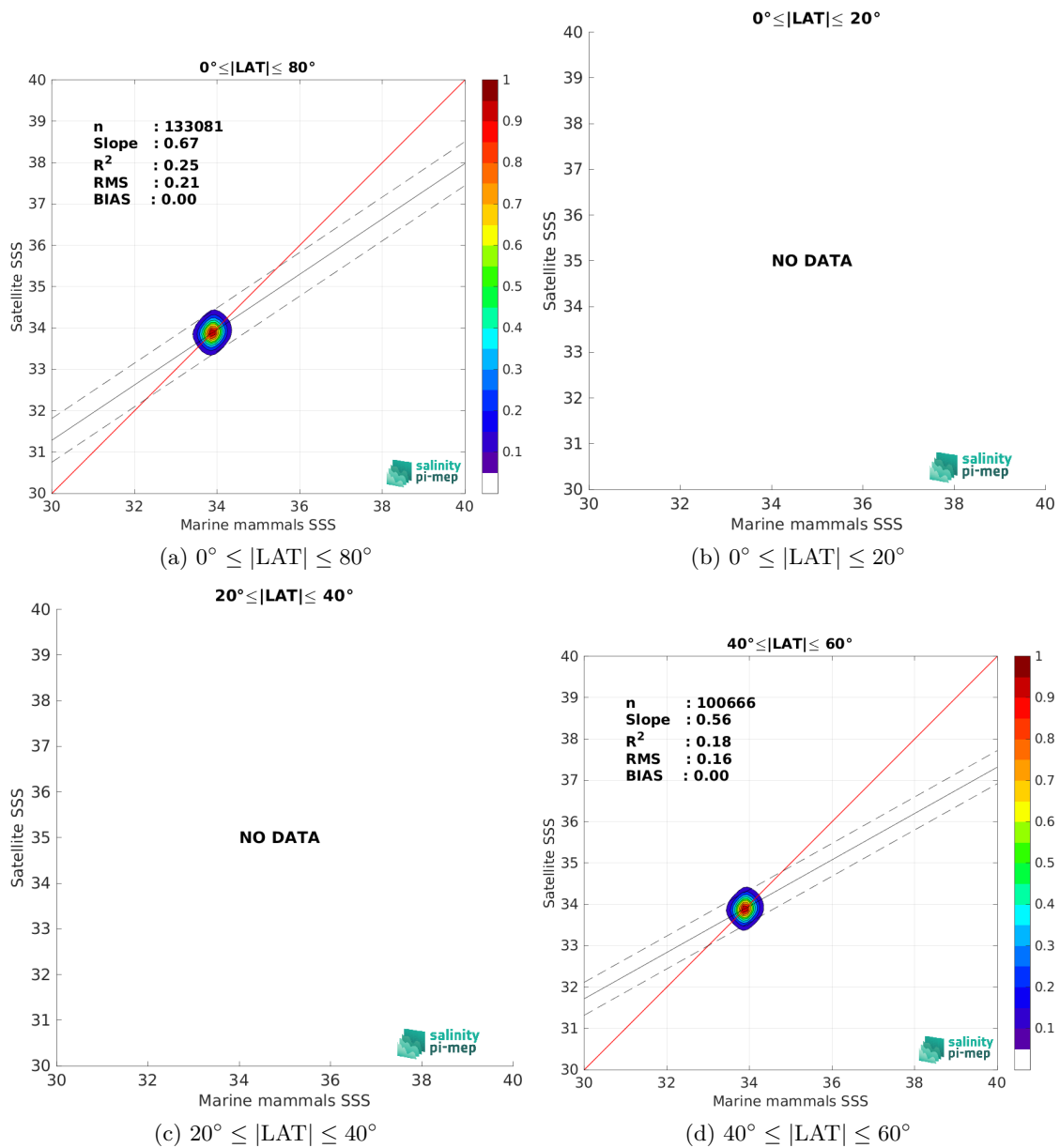
Figure 10: Contour maps of the concentration of CCI SSS L4 Merged-OI v4.41 - 7-day running (ESA) SSS (y-axis) versus Marine mammals SSS (x-axis) at match-up pairs for different latitude bands. For each plot, the red line shows x=y . The black thin and dashed lines indicate a linear fit through the data cloud and the \pm 95\% confidence levels, respectively. The number match-up pairs n , the slope and R^2 coefficient of the linear fit, the root mean square (RMS) and the mean bias between satellite and in situ data are indicated for each latitude band in each plots.
