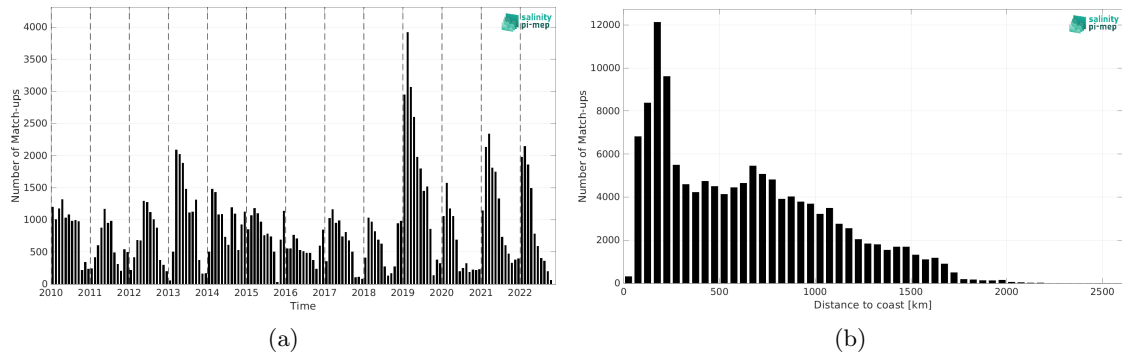
Figure 2: Number of match-ups between Marine mammals and CCI SSS L4 Merged-OI v4.41 - 7-day running (ESA) SSS as a function of time (a) and as function of the distance to coast (b) over the Southern Ocean Pi-MEP region and for the full satellite product period.
