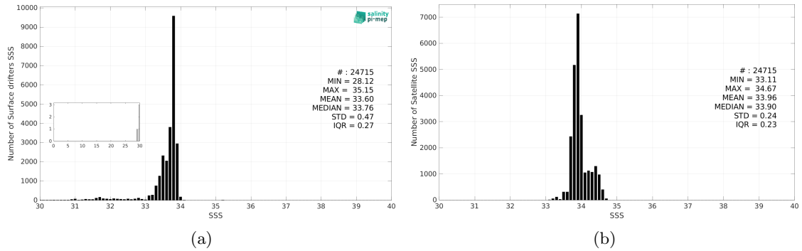
Figure 3: Histograms of SSS from Surface drifters (a) and CCI SSS L4 Merged-OI v4.41 - 7-day running (ESA) (b) considering all match-up pairs per bins of 0.1 over the Southern Ocean Pi-MEP region and for the full satellite product period.
