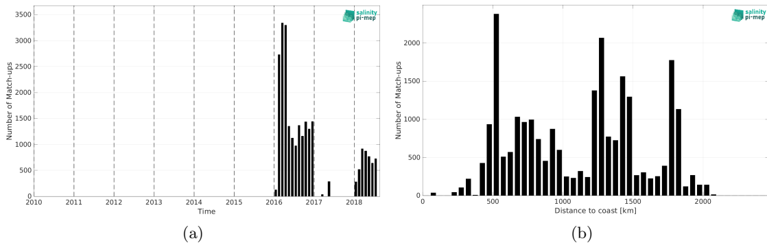
Figure 2: Number of match-ups between Surface drifters and CCI SSS L4 Merged-OI v4.41 - 7-day running (ESA) SSS as a function of time (a) and as function of the distance to coast (b) over the Southern Ocean Pi-MEP region and for the full satellite product period.
