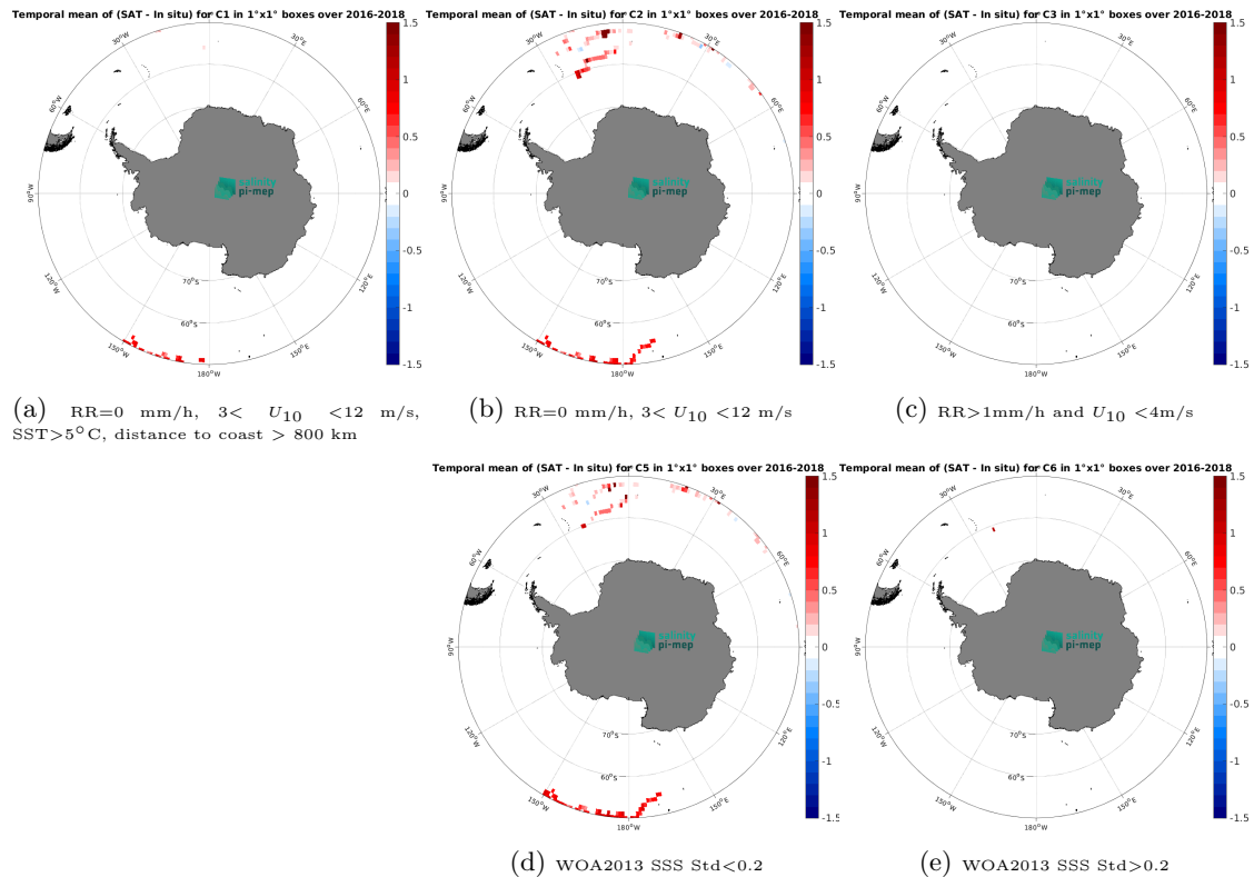
Figure 13: Temporal mean gridded over spatial boxes of size 1^\circ \times 1^\circ of \Delta\text{SSS} (CCI SSS L4 Merged-OI v4.41 - 7-day running (ESA) - Surface drifters) for 5 different subdatasets corresponding to:RR=0 mm/h, 3 < U_{10} < 12 m/s, SST >5^\circ\text{C} , distance to coast > 800 km (a), RR=0 mm/h, 3 < U_{10} < 12 m/s (b), RR >1 mm/h and U_{10} < 4 m/s (c), WOA2013 SSS Std <0.2 (d), WOA2013 SSS Std >0.2 (e).
