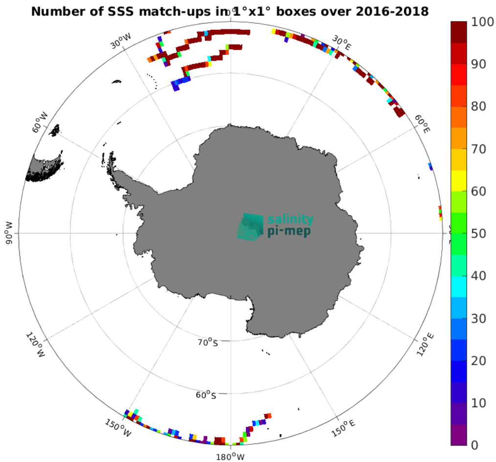
Figure 4: Number of SSS match-ups between Surface drifters SSS and the CCI SSS L4 Merged-OI v4.41 - 7-day running (ESA) SSS product for the Southern Ocean Pi-MEP region over 1^\circ \times 1^\circ boxes and for the full satellite product period.
