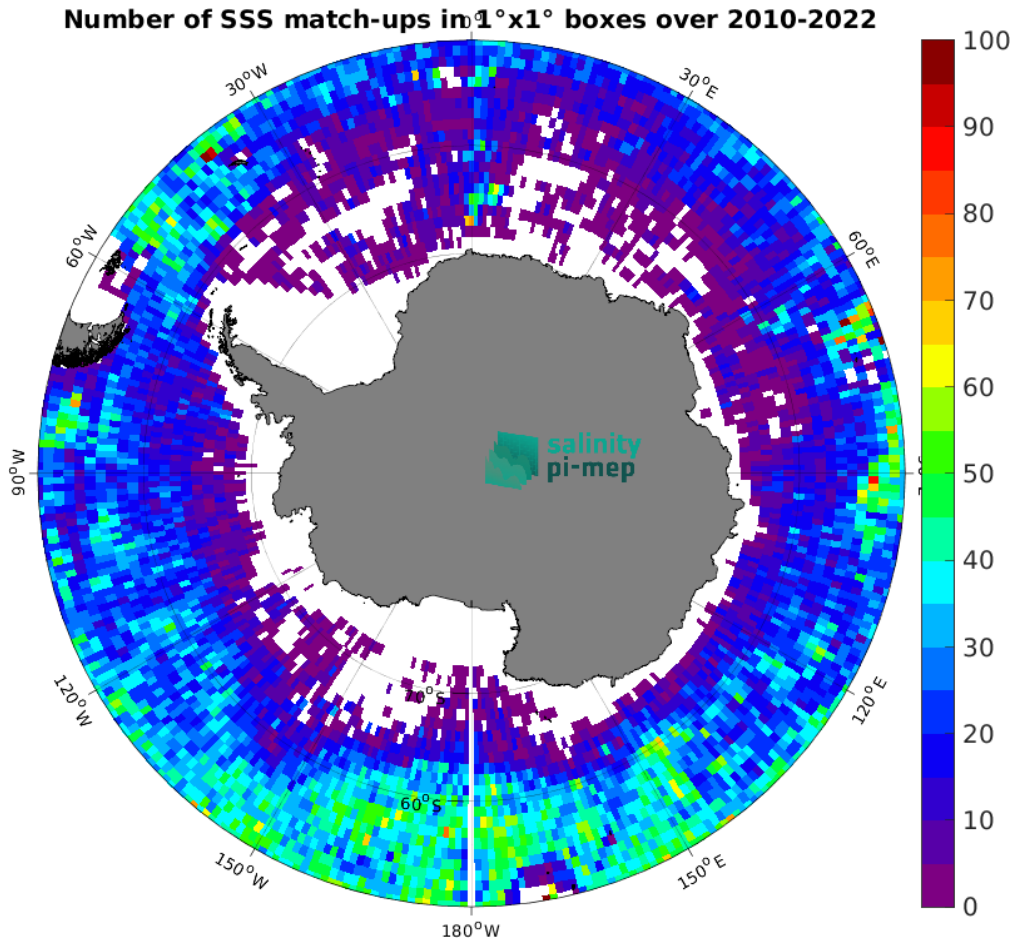
Figure 5: Number of SSS match-ups between Argo SSS and the CCI SSS L4 Merged-OI v4.41 - 7-day running (ESA) SSS product for the Southern Ocean Pi-MEP region over 1^\circ \times 1^\circ boxes and for the full satellite product period.
