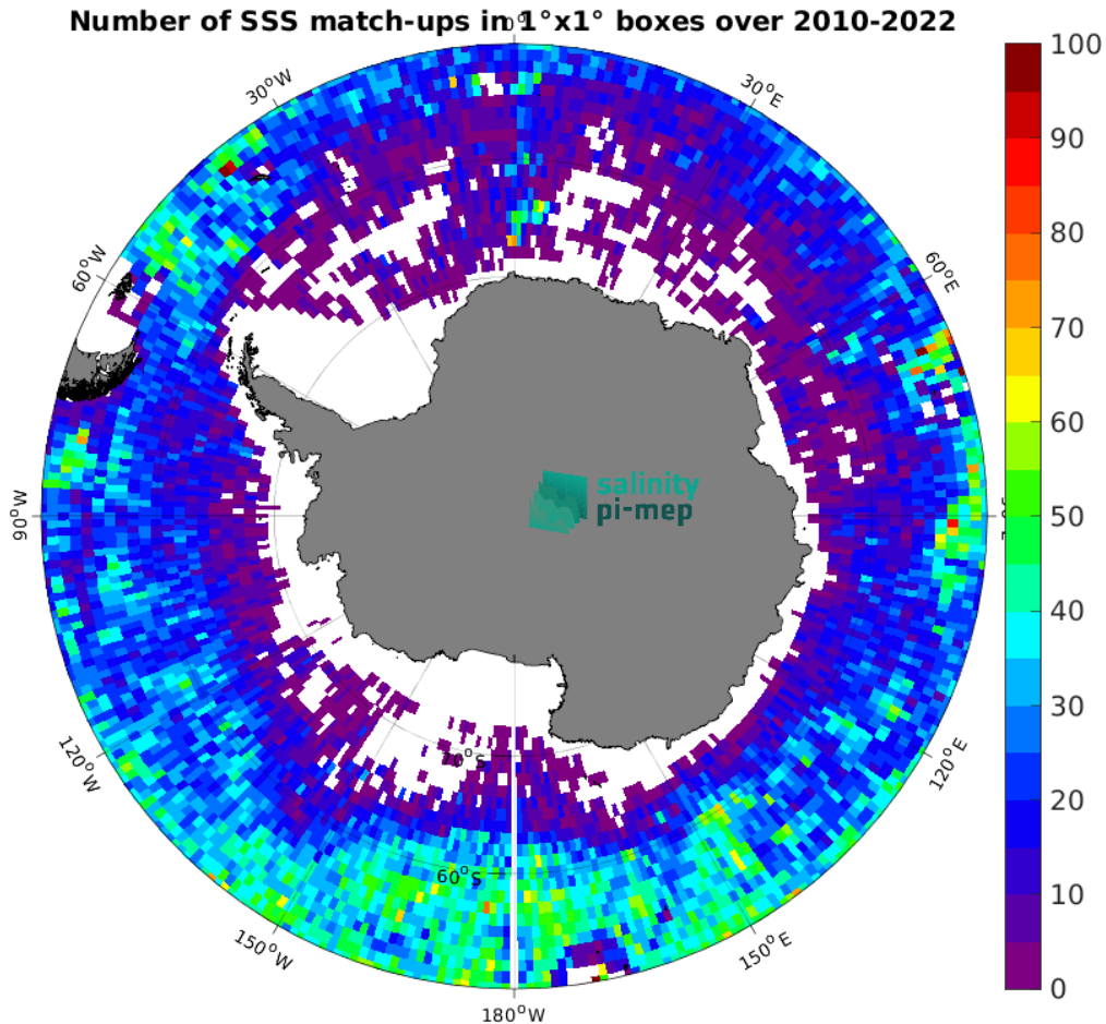
Figure 5: Number of SSS match-ups between Argo SSS and the CCI SSS L4 Merged-OI v4.41 - 7-day running (ESA) SSS product for the Southern Ocean Pi-MEP region over 1^\circ \times 1^\circ boxes and for the full satellite product period.
