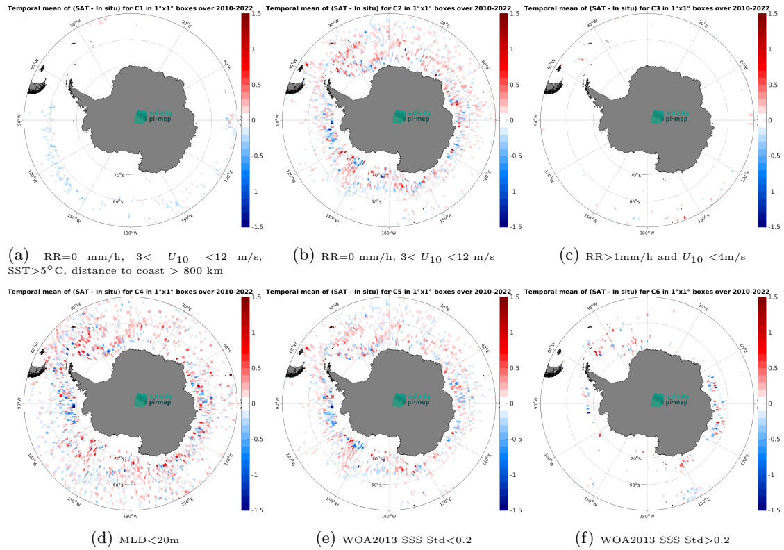
Figure 14: Temporal mean gridded over spatial boxes of size 1^\circ \times 1^\circ of \Delta\text{SSS} (CCI SSS L4 Merged-OI v4.41 - 7-day running (ESA) - Argo) for 6 different subdatasets corresponding to:RR=0 mm/h, 3 < U_{10} < 12 m/s, SST>5°C, distance to coast > 800 km (a), RR=0 mm/h, 3 < U_{10} < 12 m/s (b), RR>1mm/h and U_{10} < 4 m/s (c),MLD<20m (d),WOA2013 SSS Std<0.2 (e),WOA2013 SSS Std>0.2 (f).
