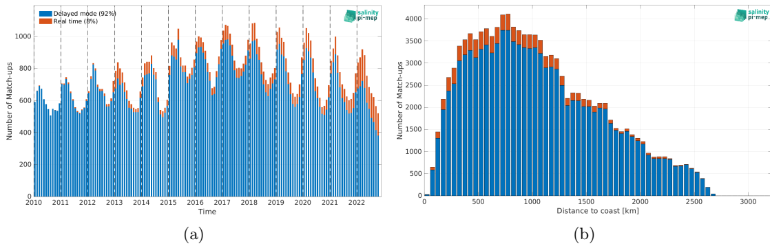
Figure 2: Number of match-ups between Argo and CCI SSS L4 Merged-OI v4.41 - 7-day running (ESA) SSS as a function of time (a) and as function of the distance to coast (b) over the Southern Ocean Pi-MEP region and for the full satellite product period.
