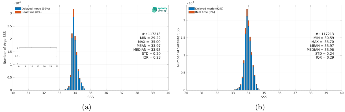
Figure 3: Histograms of SSS from Argo (a) and CCI SSS L4 Merged-OI v4.41 - 7-day running (ESA) (b) considering all match-up pairs per bins of 0.1 over the Southern Ocean Pi-MEP region and for the full satellite product period.
