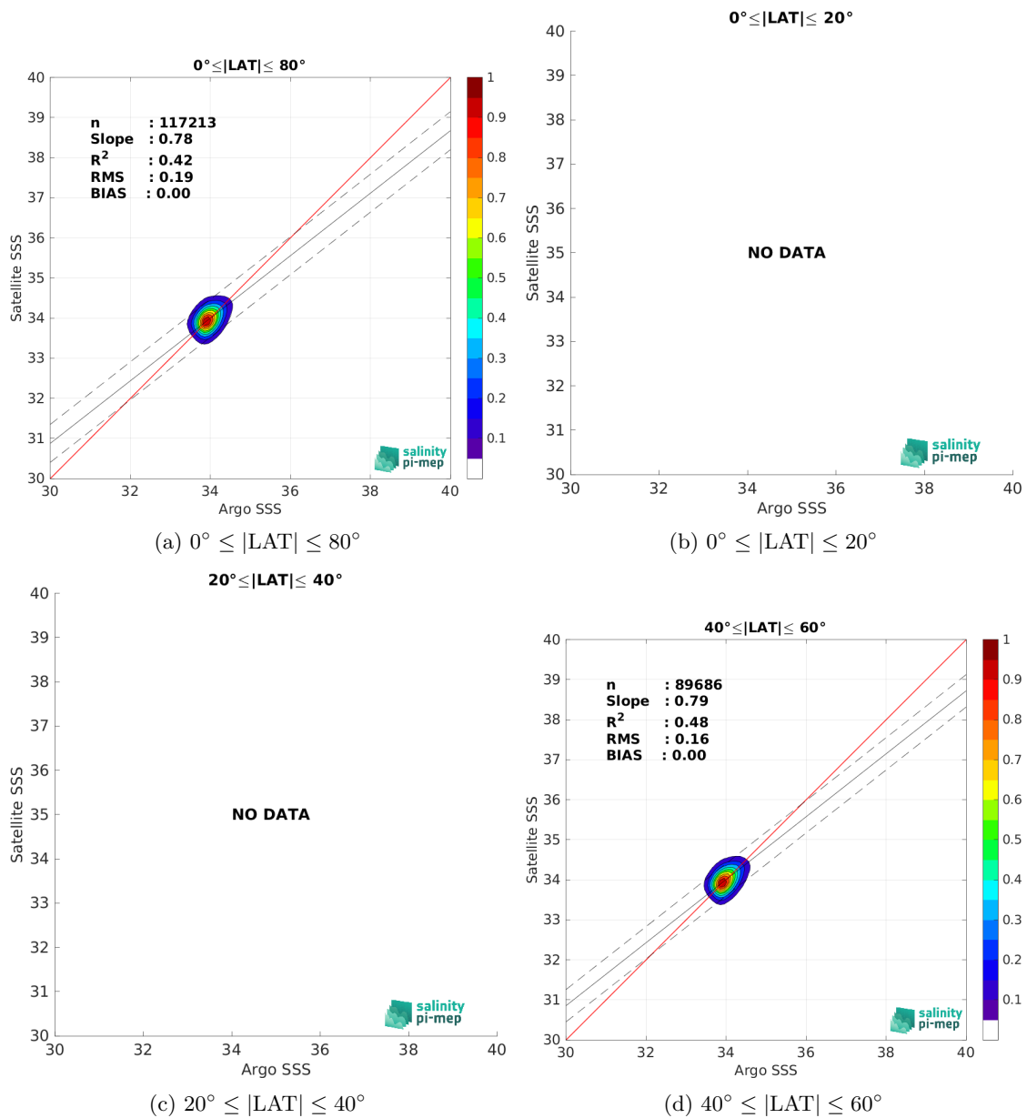
Figure 10: Contour maps of the concentration of CCI SSS L4 Merged-OI v4.41 - 7-day running (ESA) SSS (y-axis) versus Argo SSS (x-axis) at match-up pairs for different latitude bands. For each plot, the red line shows x=y . The black thin and dashed lines indicate a linear fit through the data cloud and the \pm 95\% confidence levels, respectively. The number match-up pairs n , the slope and R^2 coefficient of the linear fit, the root mean square (RMS) and the mean bias between satellite and in situ data are indicated for each latitude band in each plots.
