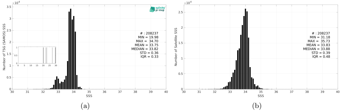
Figure 3: Histograms of SSS from TSG (SAMOS) (a) and CCI SSS L4 Merged-OI v4.41 - 30-day running (ESA) (b) considering all match-up pairs per bins of 0.1 over the Southern Ocean Pi-MEP region and for the full satellite product period.
