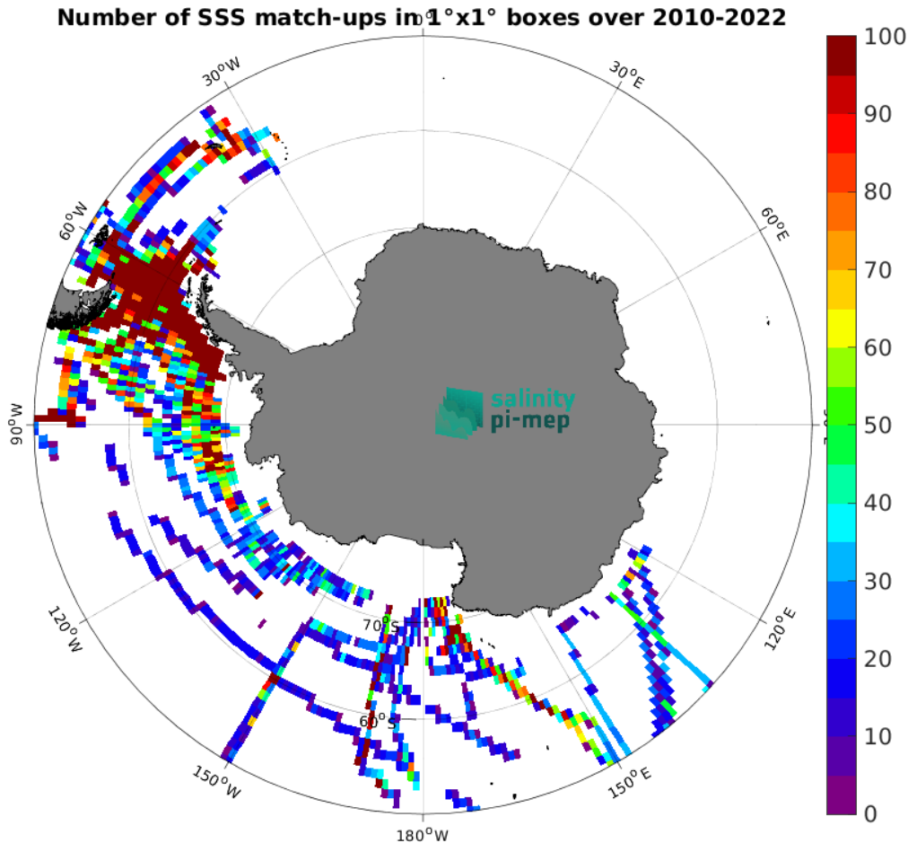
Figure 5: Number of SSS match-ups between TSG (SAMOS) SSS and the CCI SSS L4 Merged-OI v4.41 - 30-day running (ESA) SSS product for the Southern Ocean Pi-MEP region over 1^\circ \times 1^\circ boxes and for the full satellite product period.
