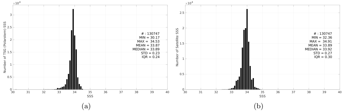
Figure 3: Histograms of SSS from TSG (Polarstern) (a) and CCI SSS L4 Merged-OI v4.41 - 30-day running (ESA) (b) considering all match-up pairs per bins of 0.1 over the Southern Ocean Pi-MEP region and for the full satellite product period.
