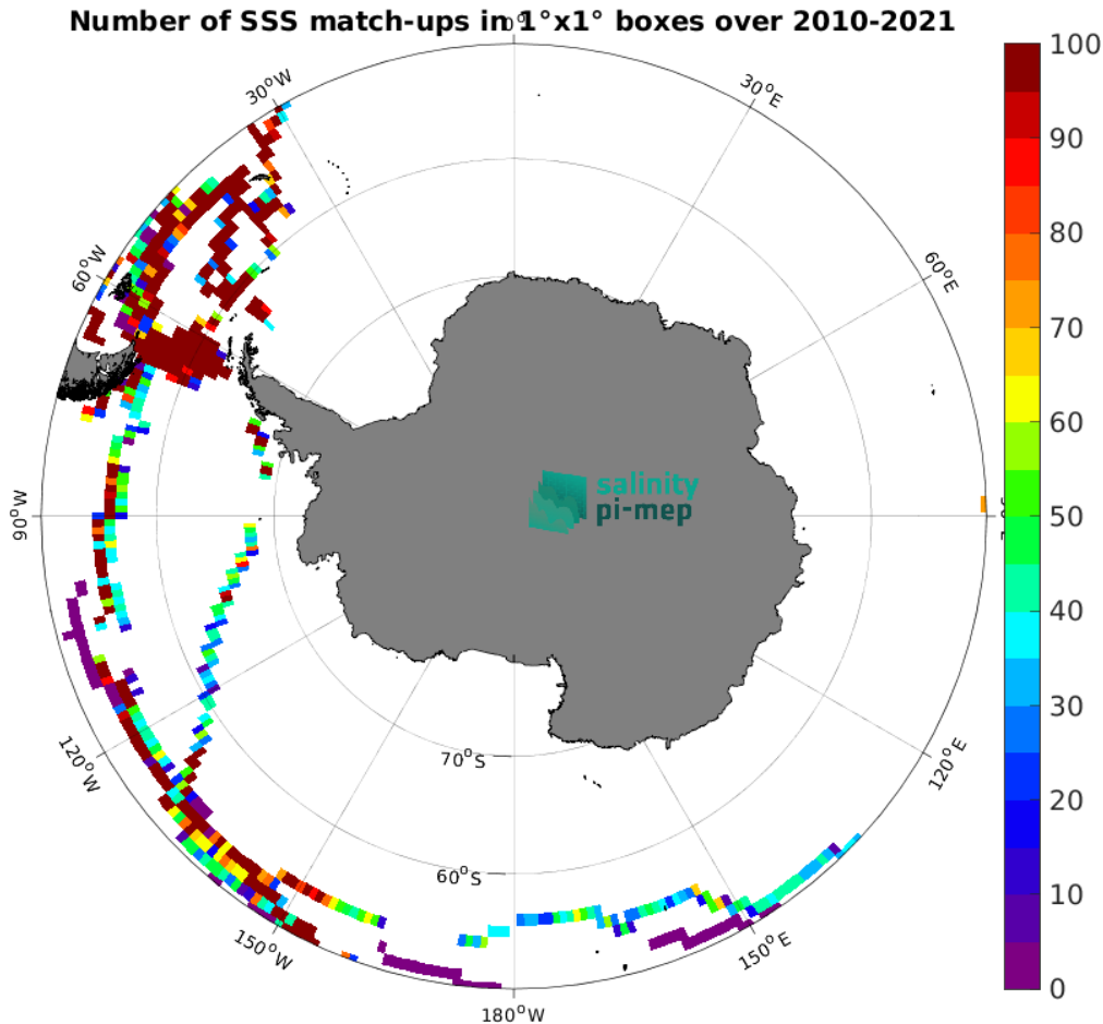
Figure 5: Number of SSS match-ups between TSG (GOSUD-Sailing-ship) SSS and the CCI SSS L4 Merged-OI v4.41 - 30-day running (ESA) SSS product for the Southern Ocean Pi-MEP region over 1^\circ \times 1^\circ boxes and for the full satellite product period.
