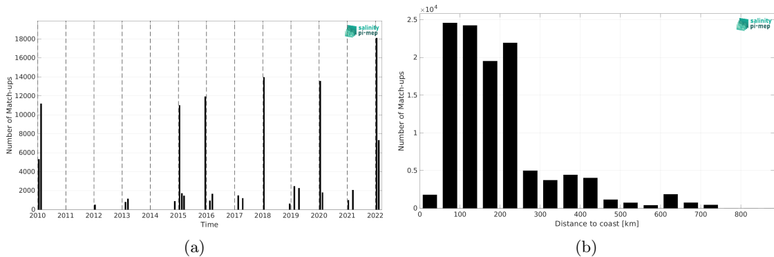
Figure 2: Number of match-ups between TSG (CSIC-UTM) and CCI SSS L4 Merged-OI v4.41 - 30-day running (ESA) SSS as a function of time (a) and as function of the distance to coast (b) over the Southern Ocean Pi-MEP region and for the full satellite product period.
