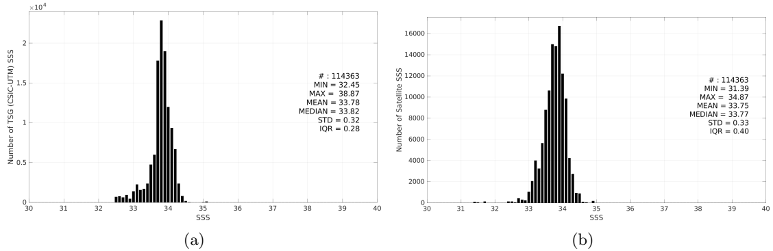
Figure 3: Histograms of SSS from TSG (CSIC-UTM) (a) and CCI SSS L4 Merged-OI v4.41 - 30-day running (ESA) (b) considering all match-up pairs per bins of 0.1 over the Southern Ocean Pi-MEP region and for the full satellite product period.
