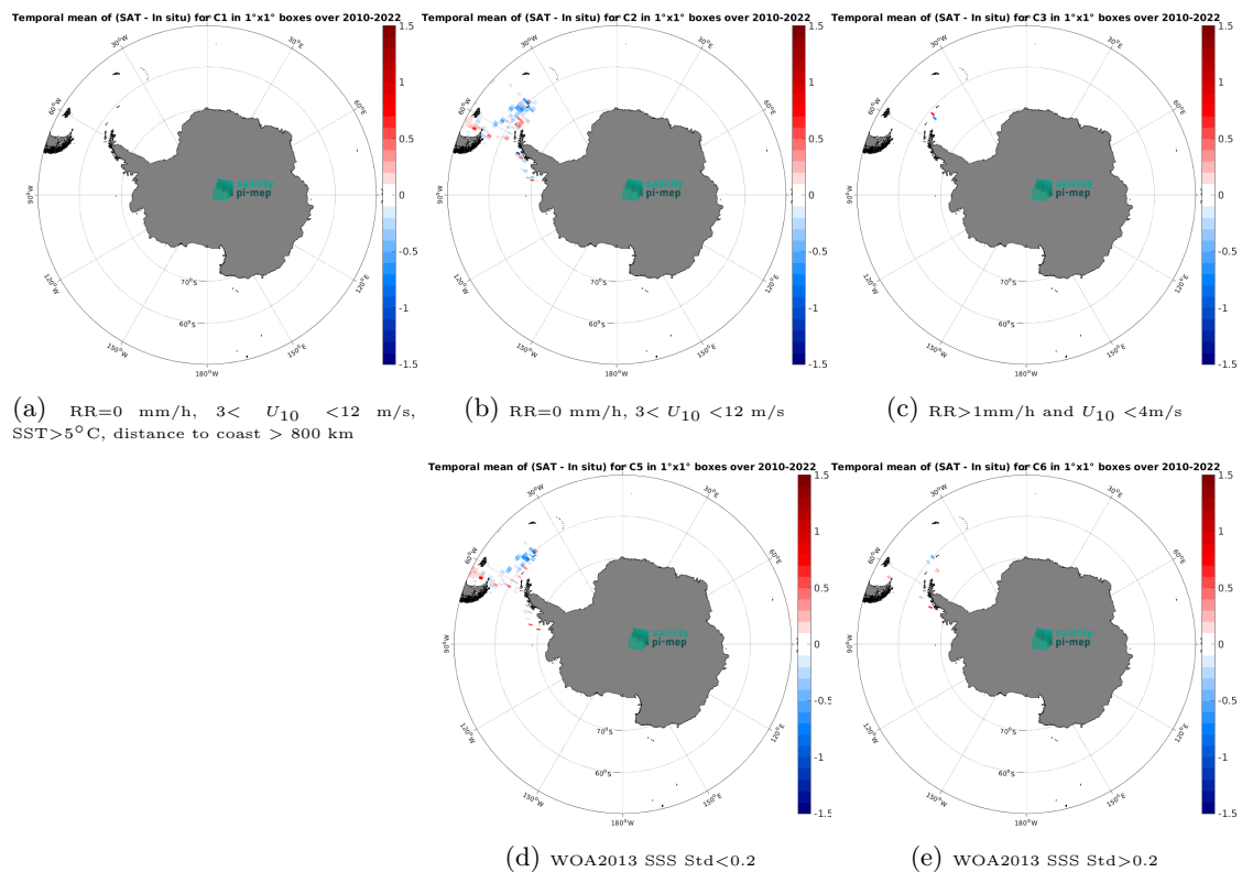
Figure 14: Temporal mean gridded over spatial boxes of size 1^\circ \times 1^\circ of \Delta SSS (CCI SSS L4 Merged-OI v4.41 - 30-day running (ESA) - TSG (CSIC-UTM)) for 5 different subdatasets corresponding to: RR=0 mm/h, 3 < U_{10} < 12 m/s, SST > 5^\circ\text{C} , distance to coast > 800 km (a), RR=0 mm/h, 3 < U_{10} < 12 m/s (b), RR > 1 mm/h and U_{10} < 4 m/s (c), WOA2013 SSS Std < 0.2 (d), WOA2013 SSS Std > 0.2 (e).
