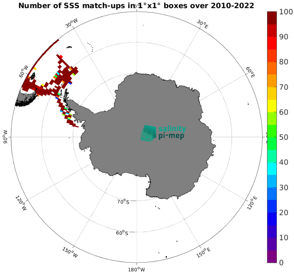
Figure 5: Number of SSS match-ups between TSG (CSIC-UTM) SSS and the CCI SSS L4 Merged-OI v4.41 - 30-day running (ESA) SSS product for the Southern Ocean Pi-MEP region over 1^\circ \times 1^\circ boxes and for the full satellite product period.
