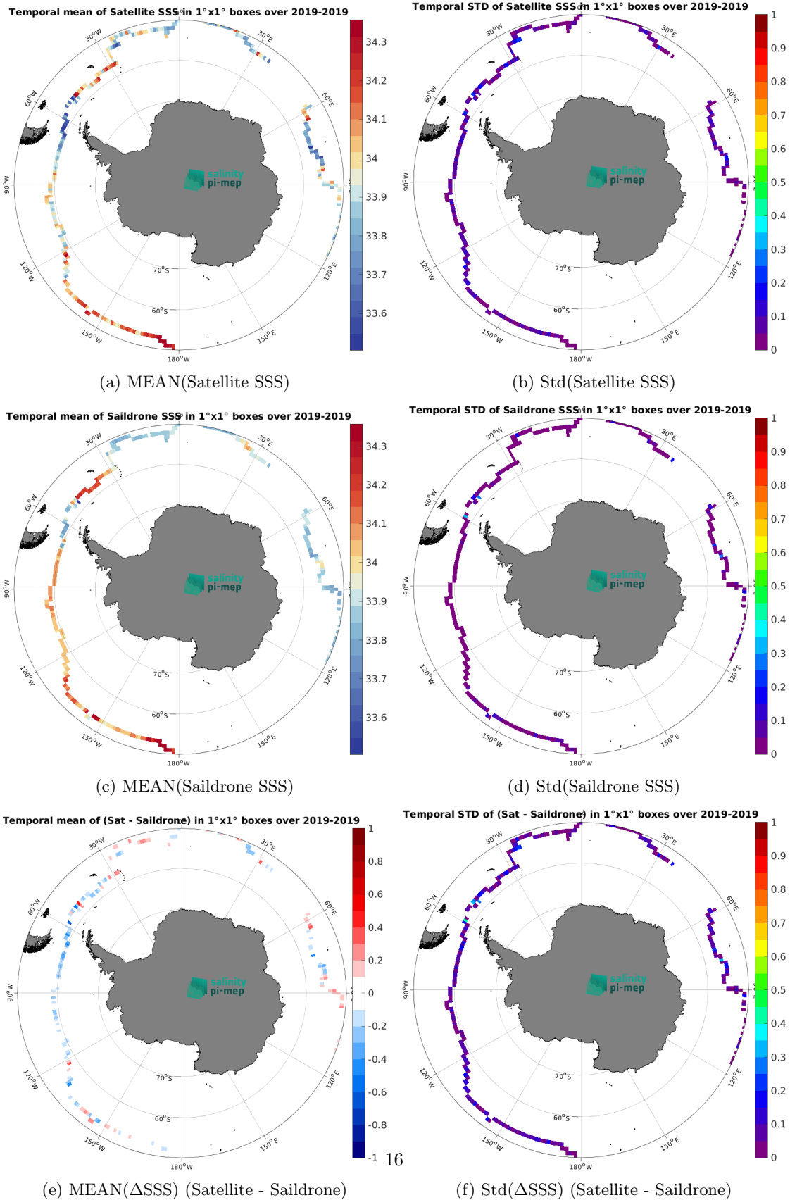
Figure 7: Temporal mean (left) and Std (right) of SSS from CCI SSS L4 Merged-OI v4.41 - 30-day running (ESA) (top), Saildrone (middle), and of \Delta SSS (Satellite - Saildrone). Only match-up pairs are used to generate these maps.
