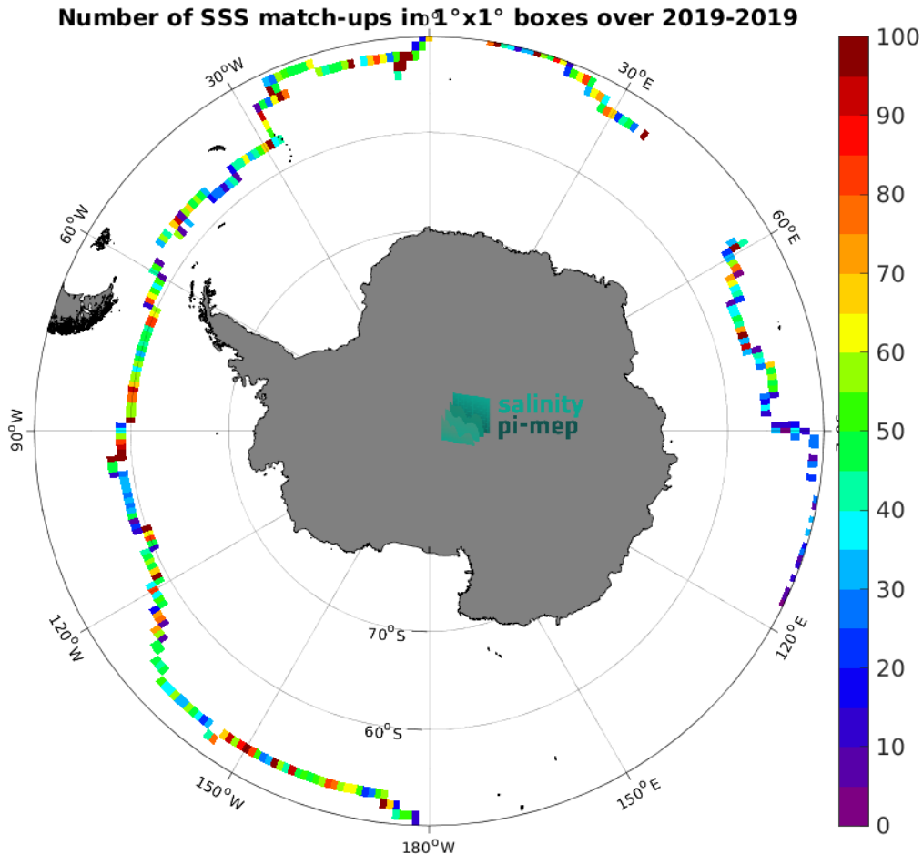
Figure 5: Number of SSS match-ups between Saildrone SSS and the CCI SSS L4 Merged-OI v4.41 - 30-day running (ESA) SSS product for the Southern Ocean Pi-MEP region over 1^\circ \times 1^\circ boxes and for the full satellite product period.
