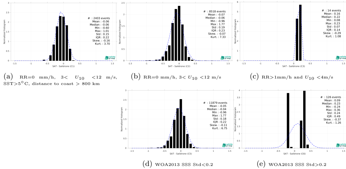
Figure 15: Normalized histogram of \Delta\text{SSS} (CCI SSS L4 Merged-OI v4.41 - 30-day running (ESA) - Saldrone) for 5 different subdatasets corresponding to: RR=0 mm/h, 3 < U_{10} < 12 m/s, SST > 5^{\circ}\text{C} , distance to coast > 800 km (a), RR=0 mm/h, 3 < U_{10} < 12 m/s (b), RR > 1\text{mm/h} and U_{10} < 4\text{m/s} (c), WOA2013 SSS Std < 0.2 (d), WOA2013 SSS Std > 0.2 (e).
