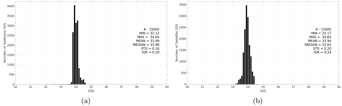
Figure 3: Histograms of SSS from Saildrone (a) and CCI SSS L4 Merged-OI v4.41 - 30-day running (ESA) (b) considering all match-up pairs per bins of 0.1 over the Southern Ocean Pi-MEP region and for the full satellite product period.
