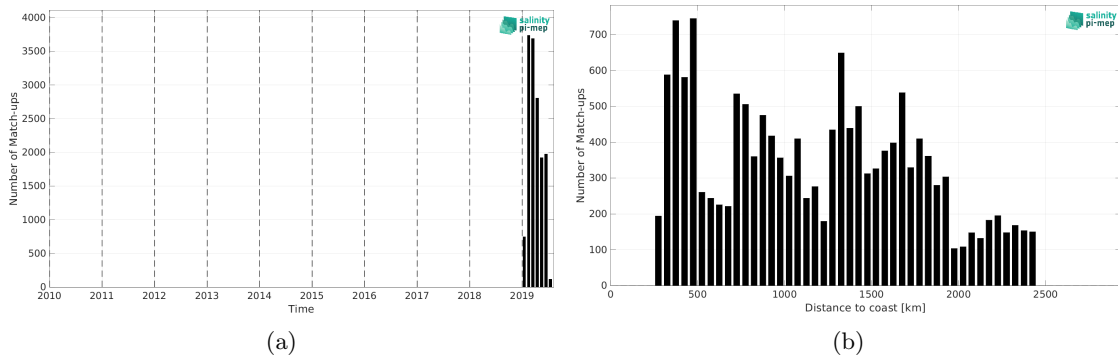
Figure 2: Number of match-ups between Saildrone and CCI SSS L4 Merged-OI v4.41 - 30-day running (ESA) SSS as a function of time (a) and as function of the distance to coast (b) over the Southern Ocean Pi-MEP region and for the full satellite product period.
