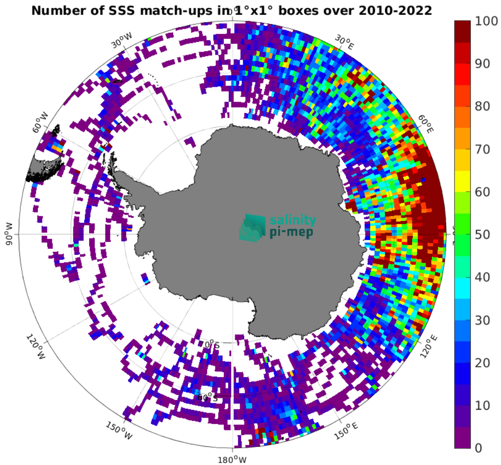
Figure 5: Number of SSS match-ups between Marine mammals SSS and the CCI SSS L4 Merged-OI v4.41 - 30-day running (ESA) SSS product for the Southern Ocean Pi-MEP region over 1^\circ \times 1^\circ boxes and for the full satellite product period.
