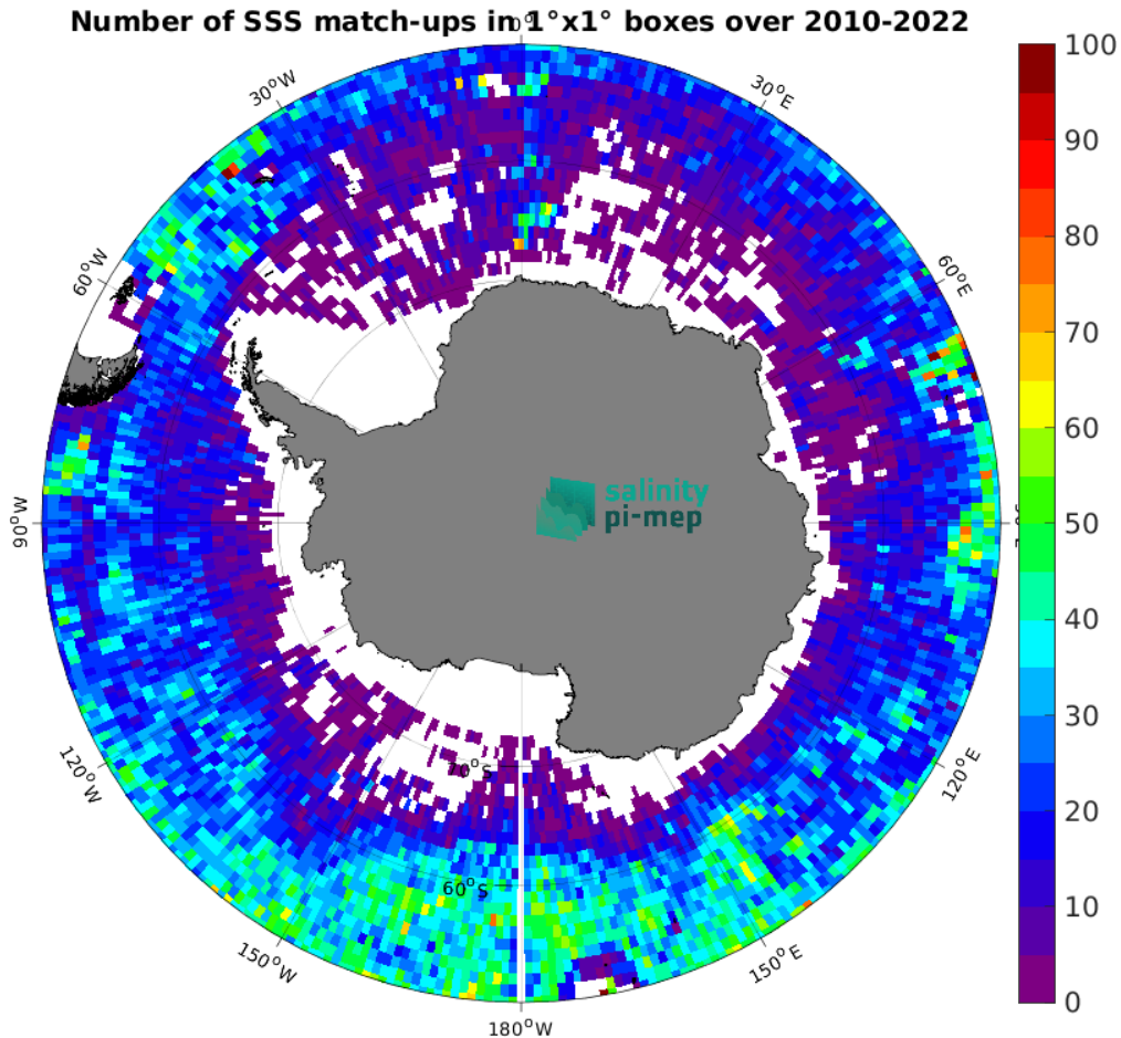
Figure 5: Number of SSS match-ups between Argo SSS and the CCI SSS L4 Merged-OI v4.41 - 30-day running (ESA) SSS product for the Southern Ocean Pi-MEP region over 1^\circ \times 1^\circ boxes and for the full satellite product period.
