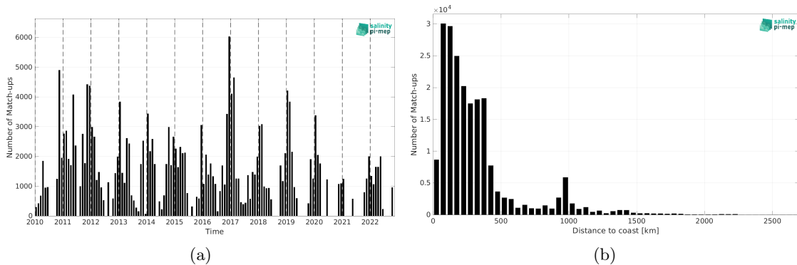
Figure 1: Number of match-ups between TSG (SAMOS) and CCI SSS L4 Merged-OI v4.4 - 7-day running (ESA) SSS as a function of time (a) and as function of the distance to coast (b) over the Southern Ocean Pi-MEP region and for the full satellite product period.
