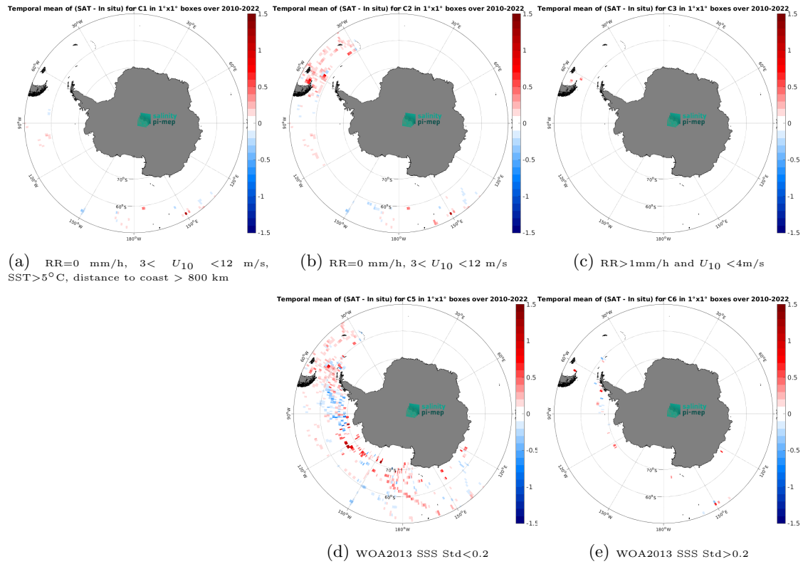
Figure 12: Temporal mean gridded over spatial boxes of size 1^{\circ}\times 1^{\circ} of \Delta\text{SSS} (CCI SSS L4 Merged-OI v4.4 - 7-day running (ESA) - TSG (SAMOS)) for 5 different subdatasets corresponding to:RR=0 mm/h, 3 < U_{10} < 12 m/s, SST >5^{\circ}\text{C} , distance to coast > 800 km (a), RR=0 mm/h, 3 < U_{10} < 12 m/s (b), RR >1 mm/h and U_{10} < 4 m/s (c), WOA2013 SSS Std <0.2 (d), WOA2013 SSS Std >0.2 (e).
