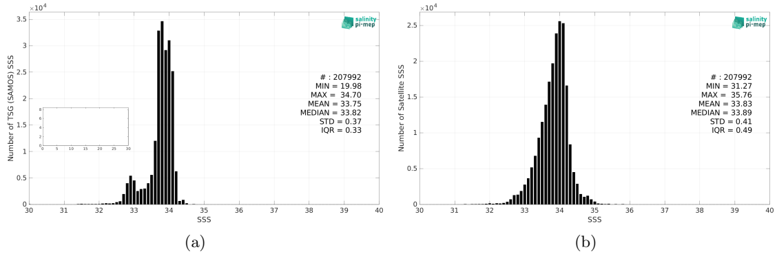
Figure 2: Histograms of SSS from TSG (SAMOS) (a) and CCI SSS L4 Merged-OI v4.4 - 7-day running (ESA) (b) considering all match-up pairs per bins of 0.1 over the Southern Ocean Pi-MEP region and for the full satellite product period.
