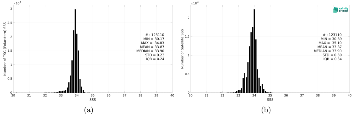
Figure 2: Histograms of SSS from TSG (Polarstern) (a) and CCI SSS L4 Merged-OI v4.4 - 7-day running (ESA) (b) considering all match-up pairs per bins of 0.1 over the Southern Ocean Pi-MEP region and for the full satellite product period.
