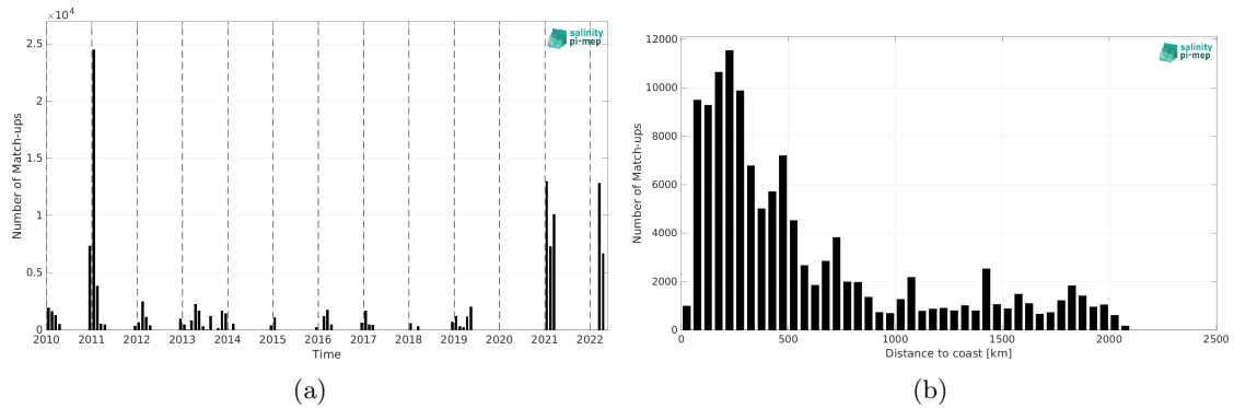
Figure 1: Number of match-ups between TSG (Polarstern) and CCI SSS L4 Merged-OI v4.4 - 7-day running (ESA) SSS as a function of time (a) and as function of the distance to coast (b) over the Southern Ocean Pi-MEP region and for the full satellite product period.
