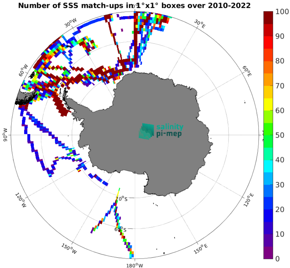
Figure 4: Number of SSS match-ups between TSG (Polarstern) SSS and the CCI SSS L4 Merged-OI v4.4 - 7-day running (ESA) SSS product for the Southern Ocean Pi-MEP region over 1^\circ \times 1^\circ boxes and for the full satellite product period.
