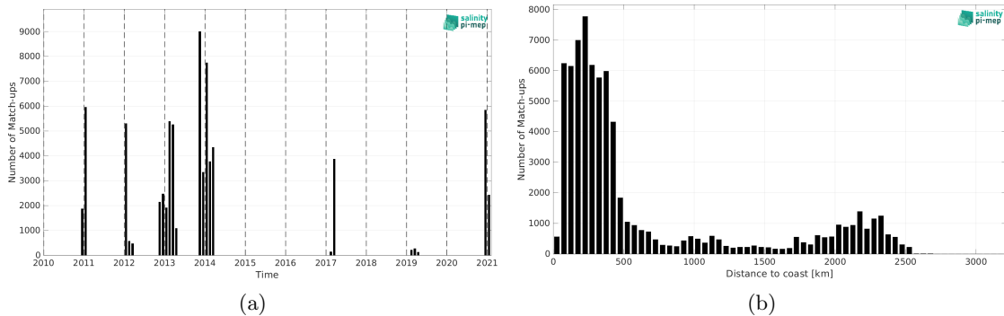
Figure 1: Number of match-ups between TSG (GOSUD-Sailing-ship) and CCI SSS L4 Merged-OI v4.4 - 7-day running (ESA) SSS as a function of time (a) and as function of the distance to coast (b) over the Southern Ocean Pi-MEP region and for the full satellite product period.
