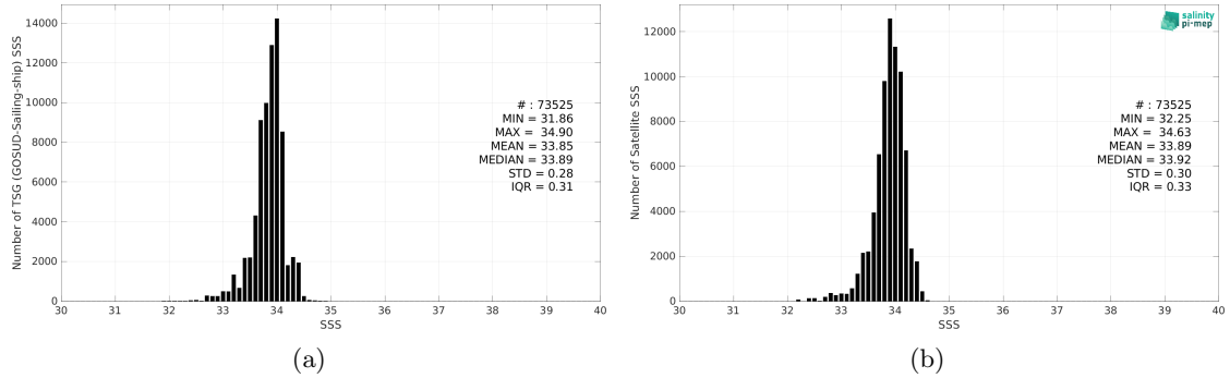
Figure 2: Histograms of SSS from TSG (GOSUD-Sailing-ship) (a) and CCI SSS L4 Merged-OI v4.4 - 7-day running (ESA) (b) considering all match-up pairs per bins of 0.1 over the Southern Ocean Pi-MEP region and for the full satellite product period.
