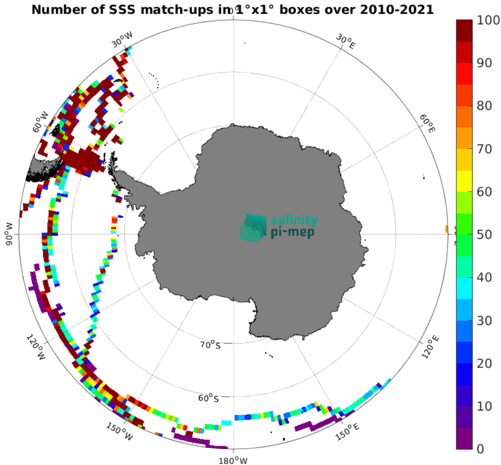
Figure 4: Number of SSS match-ups between TSG (GOSUD-Sailing-ship) SSS and the CCI SSS L4 Merged-OI v4.4 - 7-day running (ESA) SSS product for the Southern Ocean Pi-MEP region over 1^\circ \times 1^\circ boxes and for the full satellite product period.
