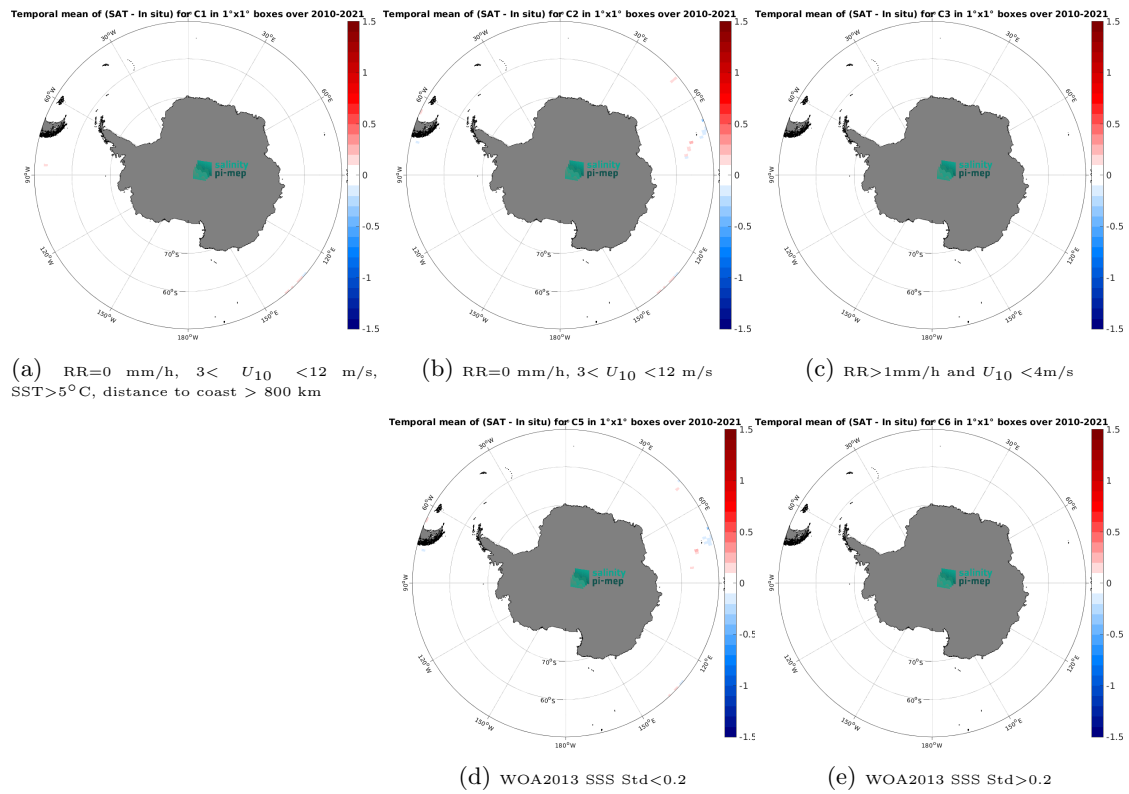
Figure 12: Temporal mean gridded over spatial boxes of size 1^\circ \times 1^\circ of \Delta SSS (CCI SSS L4 Merged-OI v4.4 - 7-day running (ESA) - TSG (GOSUD-Research-vessel)) for 5 different subdatasets corresponding to:RR=0 mm/h, 3 < U_{10} < 12 m/s, SST>5°C, distance to coast > 800 km (a), RR=0 mm/h, 3 < U_{10} < 12 m/s (b), RR>1mm/h and U_{10} < 4 m/s (c), WOA2013 SSS Std<0.2 (d), WOA2013 SSS Std>0.2 (e).
