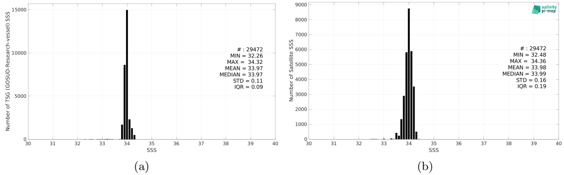
Figure 2: Histograms of SSS from TSG (GOSUD-Research-vessel) (a) and CCI SSS L4 Merged-OI v4.4 - 7-day running (ESA) (b) considering all match-up pairs per bins of 0.1 over the Southern Ocean Pi-MEP region and for the full satellite product period.
