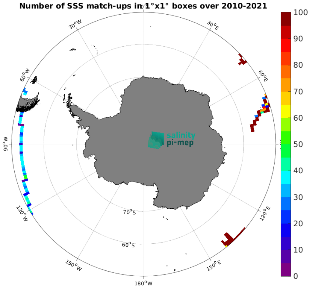
Figure 4: Number of SSS match-ups between TSG (GOSUD-Research-vessel) SSS and the CCI SSS L4 Merged-OI v4.4 - 7-day running (ESA) SSS product for the Southern Ocean Pi-MEP region over 1^\circ \times 1^\circ boxes and for the full satellite product period.
