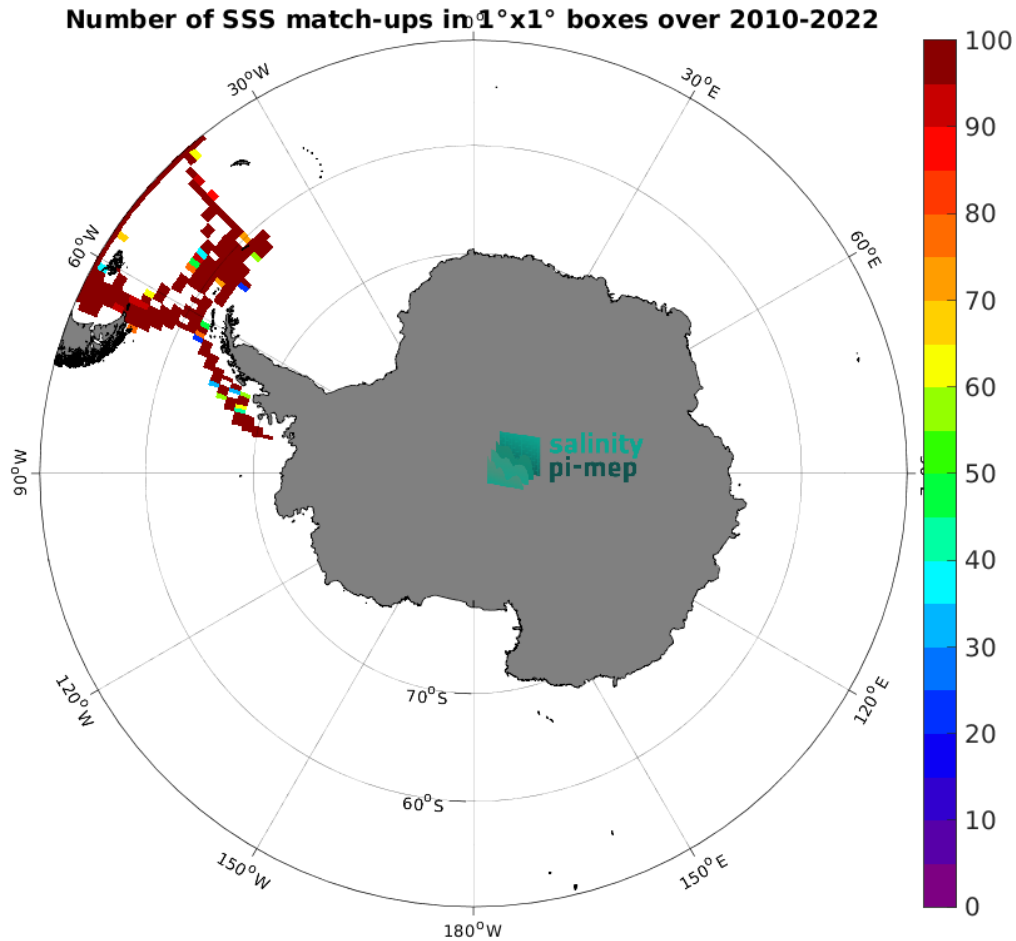
Figure 4: Number of SSS match-ups between TSG (CSIC-UTM) SSS and the CCI SSS L4 Merged-OI v4.4 - 7-day running (ESA) SSS product for the Southern Ocean Pi-MEP region over 1^\circ \times 1^\circ boxes and for the full satellite product period.
