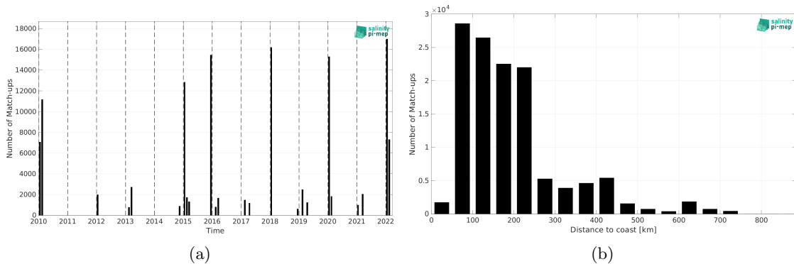
Figure 1: Number of match-ups between TSG (CSIC-UTM) and CCI SSS L4 Merged-OI v4.4 - 7-day running (ESA) SSS as a function of time (a) and as function of the distance to coast (b) over the Southern Ocean Pi-MEP region and for the full satellite product period.
