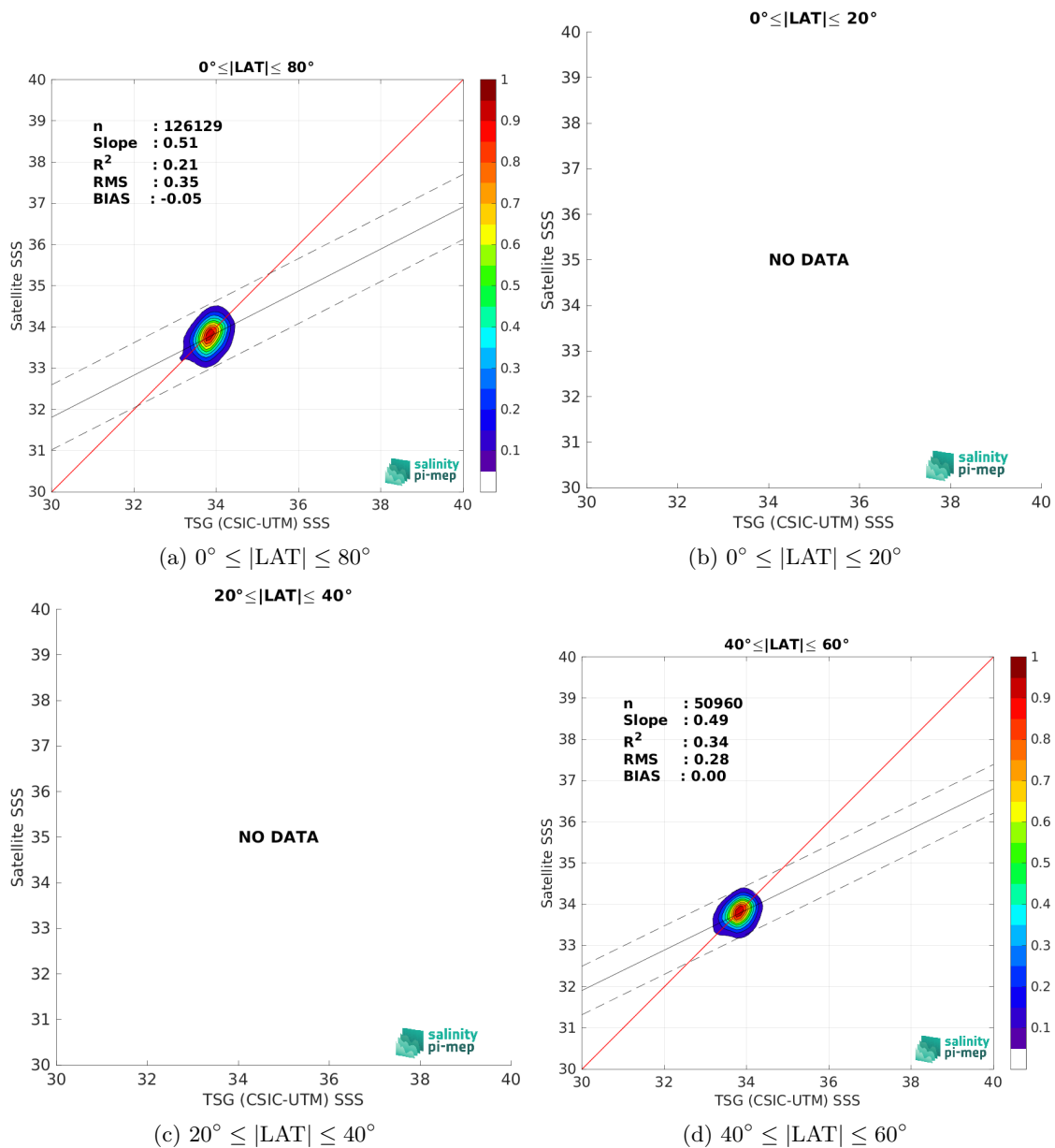
Figure 9: Contour maps of the concentration of CCI SSS L4 Merged-OI v4.4 - 7-day running (ESA) SSS (y-axis) versus TSG (CSIC-UTM) SSS (x-axis) at match-up pairs for different latitude bands. For each plot, the red line shows x=y . The black thin and dashed lines indicate a linear fit through the data cloud and the \pm 95\% confidence levels, respectively. The number match-up pairs n , the slope and R^2 coefficient of the linear fit, the root mean square (RMS) and the mean bias between satellite and in situ data are indicated for each latitude band in each plots.
