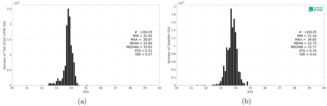
Figure 2: Histograms of SSS from TSG (CSIC-UTM) (a) and CCI SSS L4 Merged-OI v4.4 - 7-day running (ESA) (b) considering all match-up pairs per bins of 0.1 over the Southern Ocean Pi-MEP region and for the full satellite product period.
