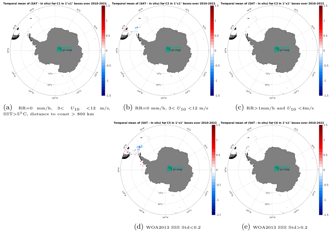
Figure 12: Temporal mean gridded over spatial boxes of size 1^{\circ}\times 1^{\circ} of \Delta\text{SSS} (CCI SSS L4 Merged-OI v4.4 - 7-day running (ESA) - TSG (CSIC-UTM)) for 5 different subdatasets corresponding to:RR=0 mm/h, 3 < U_{10} < 12 m/s, SST >5^{\circ}\text{C} , distance to coast > 800 km (a), RR=0 mm/h, 3 < U_{10} < 12 m/s (b), RR >1 mm/h and U_{10} < 4 m/s (c), WOA2013 SSS Std <0.2 (d), WOA2013 SSS Std >0.2 (e).
