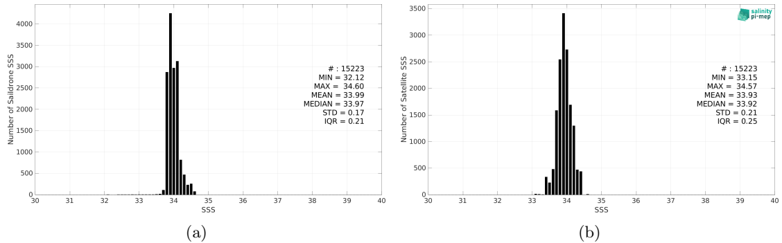
Figure 2: Histograms of SSS from Saildrone (a) and CCI SSS L4 Merged-OI v4.4 - 7-day running (ESA) (b) considering all match-up pairs per bins of 0.1 over the Southern Ocean Pi-MEP region and for the full satellite product period.
