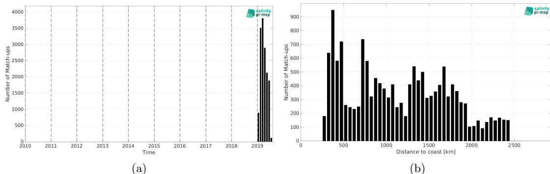
Figure 1: Number of match-ups between Saildrone and CCI SSS L4 Merged-OI v4.4 - 7-day running (ESA) SSS as a function of time (a) and as function of the distance to coast (b) over the Southern Ocean Pi-MEP region and for the full satellite product period.
