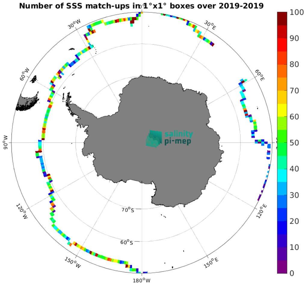
Figure 4: Number of SSS match-ups between Saildrone SSS and the CCI SSS L4 Merged-OI v4.4 - 7-day running (ESA) SSS product for the Southern Ocean Pi-MEP region over 1^\circ \times 1^\circ boxes and for the full satellite product period.
