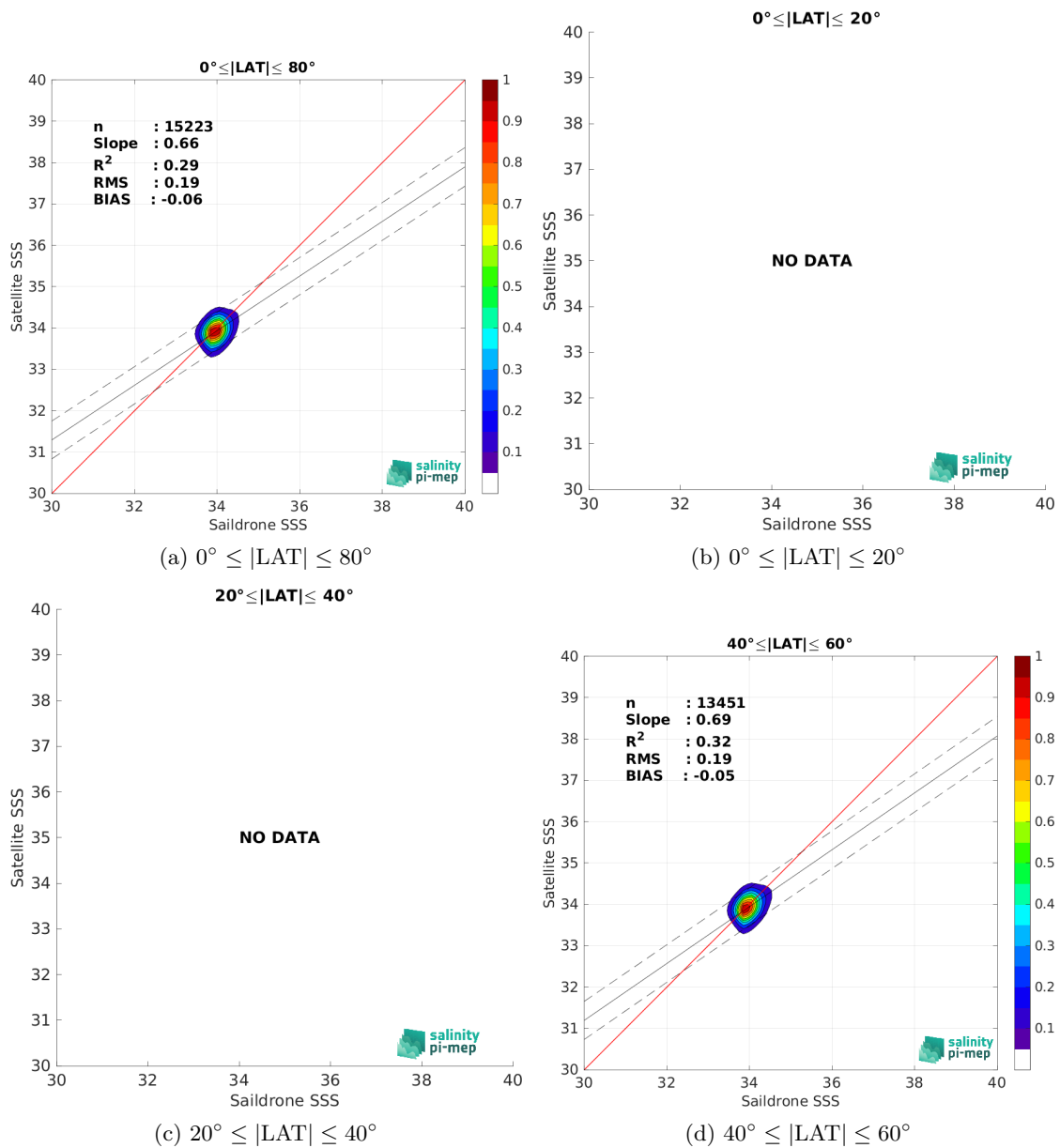
Figure 9: Contour maps of the concentration of CCI SSS L4 Merged-OI v4.4 - 7-day running (ESA) SSS (y-axis) versus Sailldrone SSS (x-axis) at match-up pairs for different latitude bands. For each plot, the red line shows x=y . The black thin and dashed lines indicate a linear fit through the data cloud and the \pm 95\% confidence levels, respectively. The number match-up pairs n , the slope and R^2 coefficient of the linear fit, the root mean square (RMS) and the mean bias between satellite and in situ data are indicated for each latitude band in each plots.
