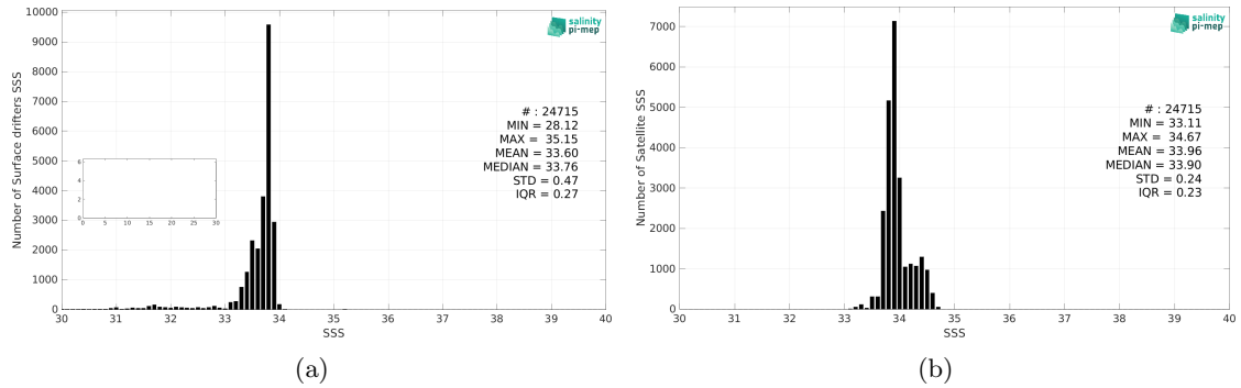
Figure 2: Histograms of SSS from Surface drifters (a) and CCI SSS L4 Merged-OI v4.4 - 7-day running (ESA) (b) considering all match-up pairs per bins of 0.1 over the Southern Ocean Pi-MEP region and for the full satellite product period.
