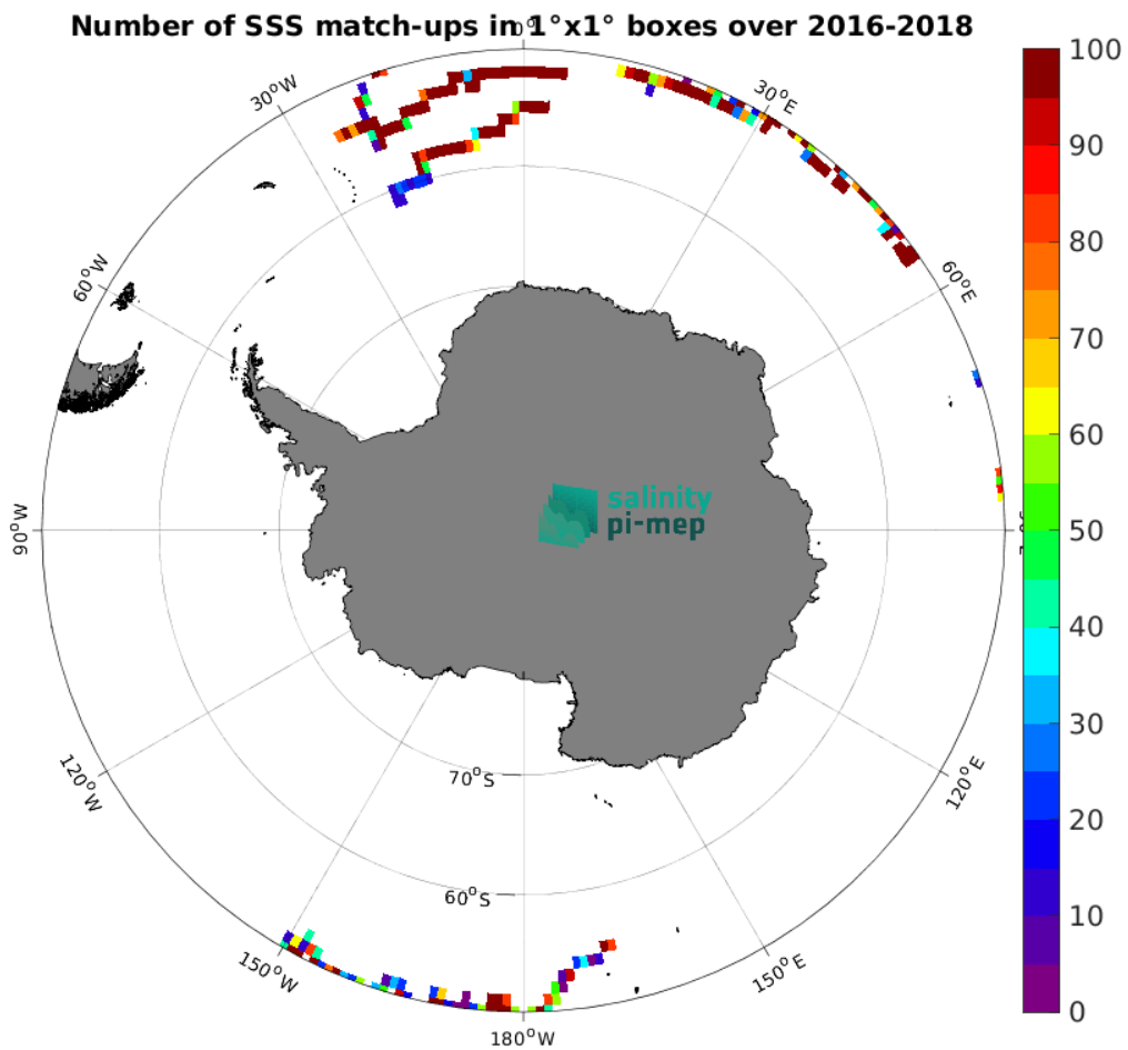
Figure 3: Number of SSS match-ups between Surface drifters SSS and the CCI SSS L4 Merged-OI v4.4 - 7-day running (ESA) SSS product for the Southern Ocean Pi-MEP region over 1^\circ \times 1^\circ boxes and for the full satellite product period.
