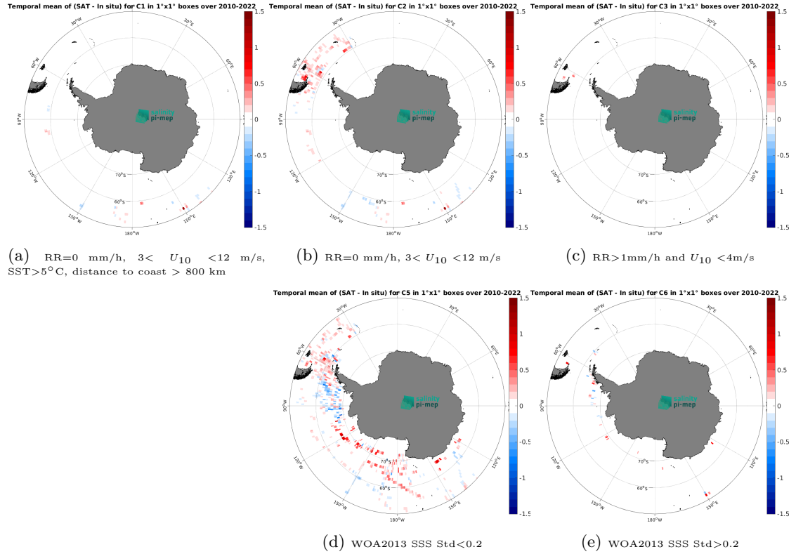
Figure 12: Temporal mean gridded over spatial boxes of size 1^{\circ}\times 1^{\circ} of \Delta\text{SSS} (CCI SSS L4 Merged-OI v4.4 - 30-day running (ESA) - TSG (SAMOS)) for 5 different subdatasets corresponding to:RR=0 mm/h, 3 < U_{10} < 12 m/s, SST >5^{\circ}\text{C} , distance to coast > 800 km (a), RR=0 mm/h, 3 < U_{10} < 12 m/s (b), RR >1 mm/h and U_{10} < 4 m/s (c), WOA2013 SSS Std <0.2 (d), WOA2013 SSS Std >0.2 (e).
