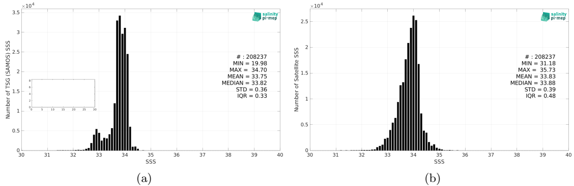
Figure 2: Histograms of SSS from TSG (SAMOS) (a) and CCI SSS L4 Merged-OI v4.4 - 30-day running (ESA) (b) considering all match-up pairs per bins of 0.1 over the Southern Ocean Pi-MEP region and for the full satellite product period.
