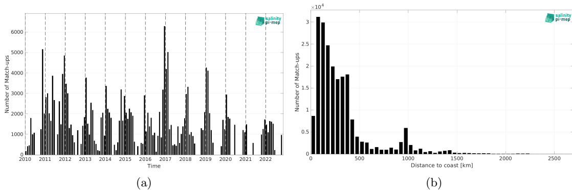
Figure 1: Number of match-ups between TSG (SAMOS) and CCI SSS L4 Merged-OI v4.4 - 30-day running (ESA) SSS as a function of time (a) and as function of the distance to coast (b) over the Southern Ocean Pi-MEP region and for the full satellite product period.
