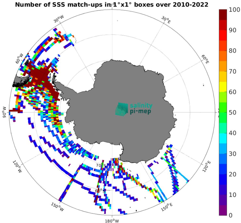
Figure 4: Number of SSS match-ups between TSG (SAMOS) SSS and the CCI SSS L4 Merged-OI v4.4 - 30-day running (ESA) SSS product for the Southern Ocean Pi-MEP region over 1^\circ \times 1^\circ boxes and for the full satellite product period.
