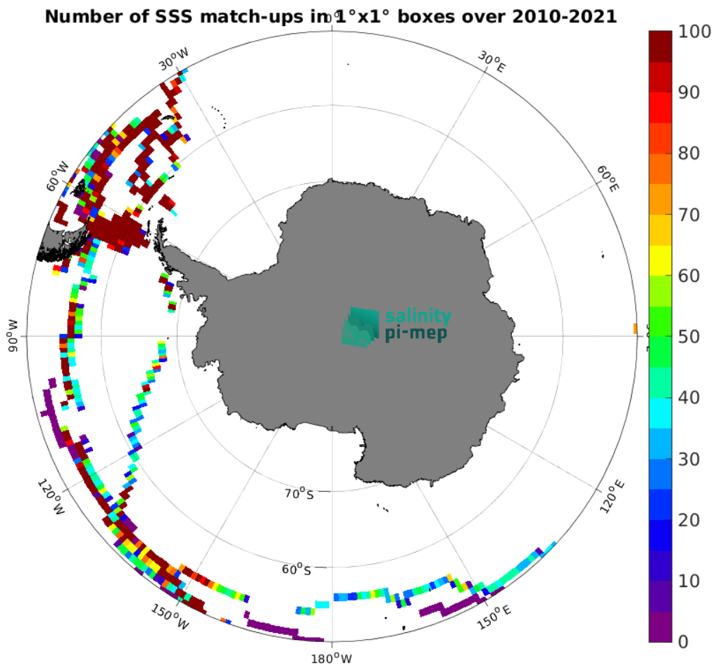
Figure 4: Number of SSS match-ups between TSG (GOSUD-Sailing-ship) SSS and the CCI SSS L4 Merged-OI v4.4 - 30-day running (ESA) SSS product for the Southern Ocean Pi-MEP region over 1^\circ \times 1^\circ boxes and for the full satellite product period.
