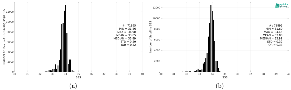
Figure 2: Histograms of SSS from TSG (GOSUD-Sailing-ship) (a) and CCI SSS L4 Merged-OI v4.4 - 30-day running (ESA) (b) considering all match-up pairs per bins of 0.1 over the Southern Ocean Pi-MEP region and for the full satellite product period.
