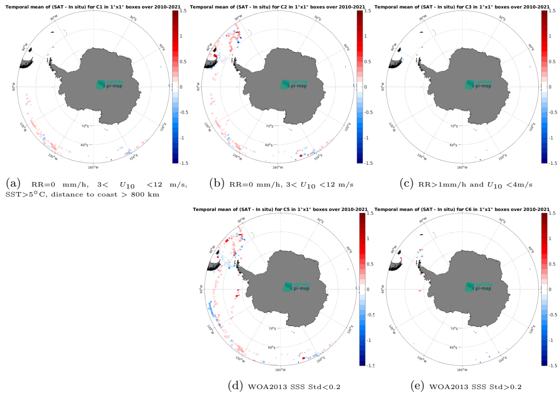
Figure 12: Temporal mean gridded over spatial boxes of size 1^\circ \times 1^\circ of \Delta\text{SSS} (CCI SSS L4 Merged-OI v4.4 - 30-day running (ESA) - TSG (GOSUD-Sailing-ship)) for 5 different subdatasets corresponding to: RR=0 mm/h, 3 < U_{10} < 12 m/s, SST > 5^\circ\text{C} , distance to coast > 800 km (a), RR=0 mm/h, 3 < U_{10} < 12 m/s (b), RR > 1 mm/h and U_{10} < 4 m/s (c), WOA2013 SSS Std < 0.2 (d), WOA2013 SSS Std > 0.2 (e).
