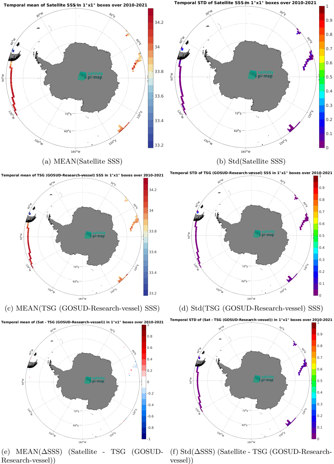
Figure 6: Temporal mean (left) and Std (right) of SSS from CCI SSS L4 Merged-OI v4.4 - 30-day running (ESA) (top), TSG (GOSUD-Research-vessel) (middle), and of \Delta SSS (Satellite - TSG (GOSUD-Research-vessel)). Only match-up pairs are used to generate these maps.
