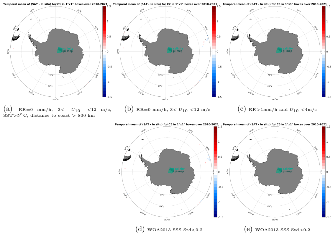
Figure 12: Temporal mean gridded over spatial boxes of size 1^\circ \times 1^\circ of \Delta SSS (CCI SSS L4 Merged-OI v4.4 - 30-day running (ESA) - TSG (GOSUD-Research-vessel)) for 5 different subdatasets corresponding to:RR=0 mm/h, 3 < U_{10} < 12 m/s, SST>5°C, distance to coast > 800 km (a), RR=0 mm/h, 3 < U_{10} < 12 m/s (b), RR>1mm/h and U_{10} < 4 m/s (c), WOA2013 SSS Std<0.2 (d), WOA2013 SSS Std>0.2 (e).
