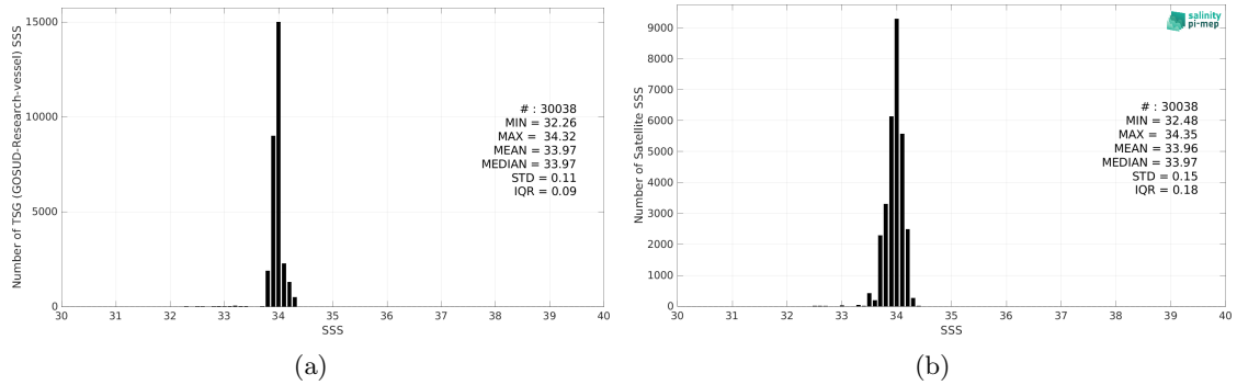
Figure 2: Histograms of SSS from TSG (GOSUD-Research-vessel) (a) and CCI SSS L4 Merged-OI v4.4 - 30-day running (ESA) (b) considering all match-up pairs per bins of 0.1 over the Southern Ocean Pi-MEP region and for the full satellite product period.
