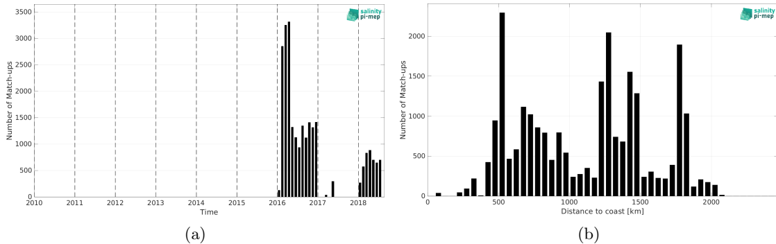
Figure 1: Number of match-ups between Surface drifters and CCI SSS L4 Merged-OI v4.4 - 30-day running (ESA) SSS as a function of time (a) and as function of the distance to coast (b) over the Southern Ocean Pi-MEP region and for the full satellite product period.
