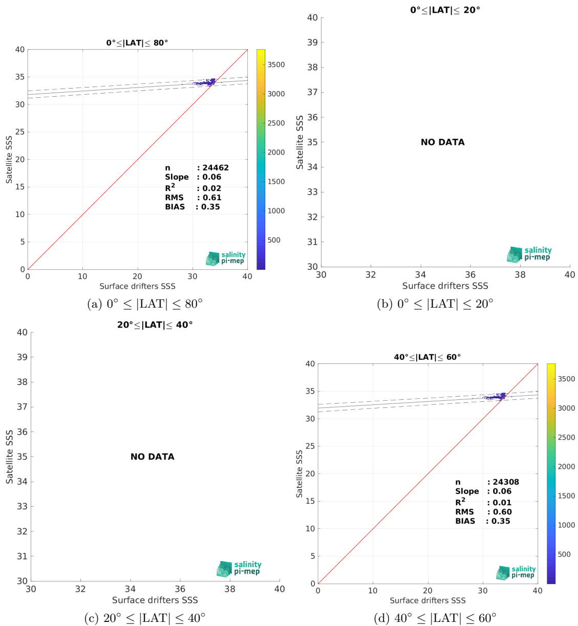
Figure 8: Contour maps of the concentration of CCI SSS L4 Merged-OI v4.4 - 30-day running (ESA) SSS (y-axis) versus Surface drifters SSS (x-axis) at match-up pairs for different latitude bands. For each plot, the red line shows x=y . The black thin and dashed lines indicate a linear fit through the data cloud and the \pm 95\% confidence levels, respectively. The number match-up pairs n , the slope and R^2 coefficient of the linear fit, the root mean square (RMS) and the mean bias between satellite and in situ data are indicated for each latitude band in each plots.
