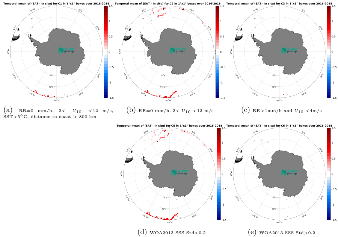
Figure 11: Temporal mean gridded over spatial boxes of size 1^{\circ}\times 1^{\circ} of \Delta\text{SSS} (CCI SSS L4 Merged-OI v4.4 - 30-day running (ESA) - Surface drifters) for 5 different subdatasets corresponding to:RR=0 mm/h, 3 < U_{10} < 12 m/s, SST >5^{\circ}\text{C} , distance to coast > 800 km (a), RR=0 mm/h, 3 < U_{10} < 12 m/s (b), RR >1 mm/h and U_{10} < 4 m/s (c), WOA2013 SSS Std <0.2 (d), WOA2013 SSS Std >0.2 (e).
