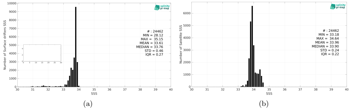
Figure 2: Histograms of SSS from Surface drifters (a) and CCI SSS L4 Merged-OI v4.4 - 30-day running (ESA) (b) considering all match-up pairs per bins of 0.1 over the Southern Ocean Pi-MEP region and for the full satellite product period.
