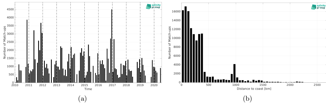
Figure 1: Number of match-ups between TSG (SAMOS) and CCI SSS L4 Merged-OI v3.2 - 7-day running (ESA) SSS as a function of time (a) and as function of the distance to coast (b) over the Southern Ocean Pi-MEP region and for the full satellite product period.
