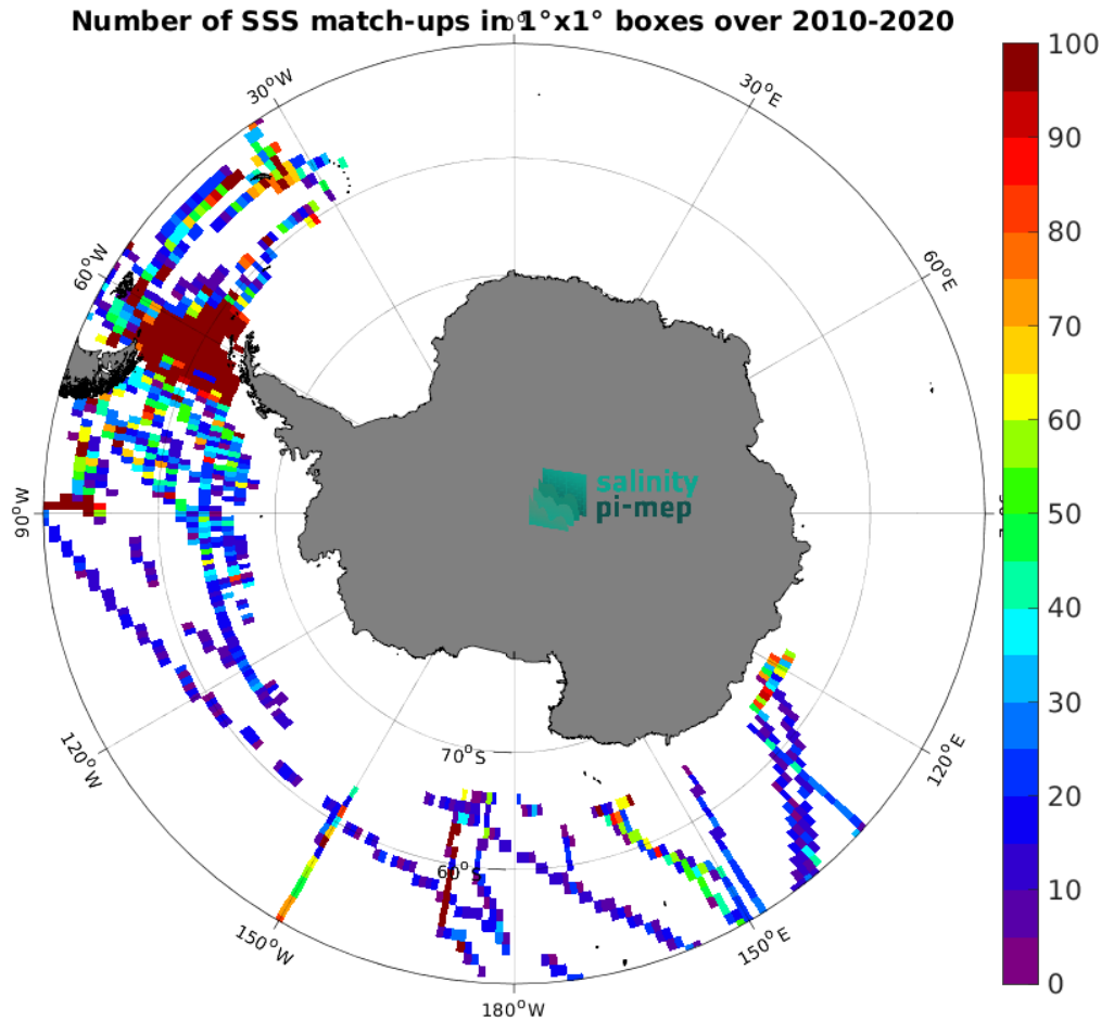
Figure 4: Number of SSS match-ups between TSG (SAMOS) SSS and the CCI SSS L4 Merged-OI v3.2 - 7-day running (ESA) SSS product for the Southern Ocean Pi-MEP region over 1^\circ \times 1^\circ boxes and for the full satellite product period.
