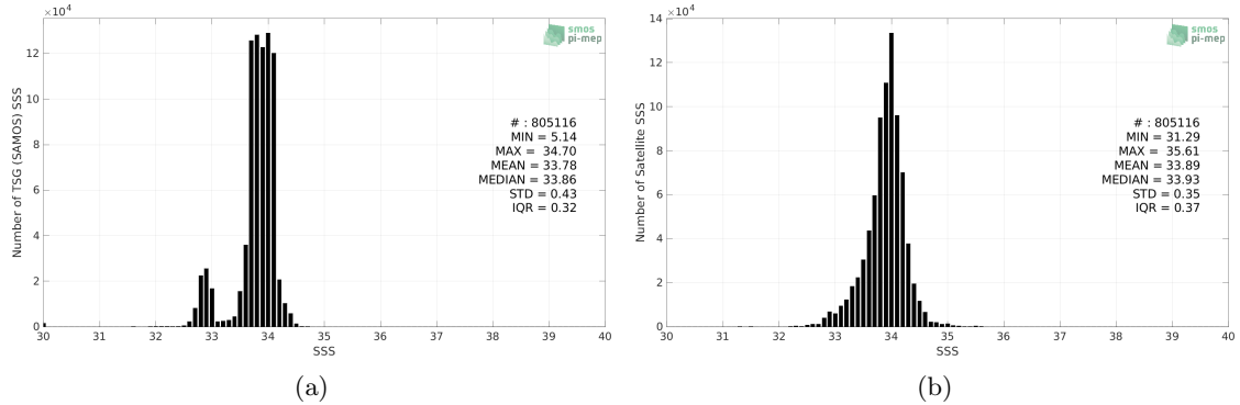
Figure 2: Histograms of SSS from TSG (SAMOS) (a) and CCI SSS L4 Merged-OI v3.2 - 7-day running (ESA) (b) considering all match-up pairs per bins of 0.1 over the Southern Ocean Pi-MEP region and for the full satellite product period.
