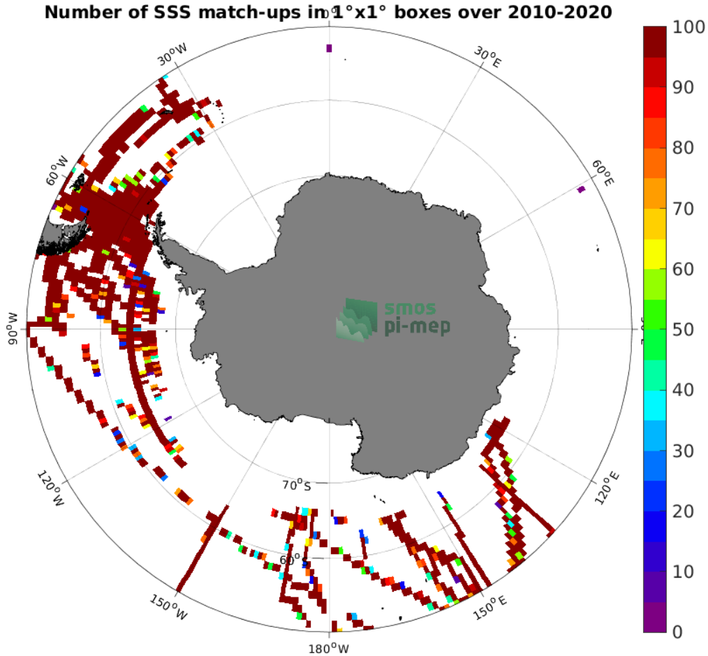
Figure 4: Number of SSS match-ups between TSG (SAMOS) SSS and the CCI SSS L4 Merged-OI v3.2 - 7-day running (ESA) SSS product for the Southern Ocean Pi-MEP region over 1^\circ \times 1^\circ boxes and for the full satellite product period.
