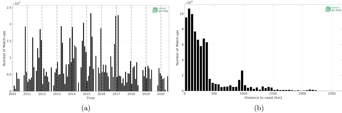
Figure 1: Number of match-ups between TSG (SAMOS) and CCI SSS L4 Merged-OI v3.2 - 7-day running (ESA) SSS as a function of time (a) and as function of the distance to coast (b) over the Southern Ocean Pi-MEP region and for the full satellite product period.
