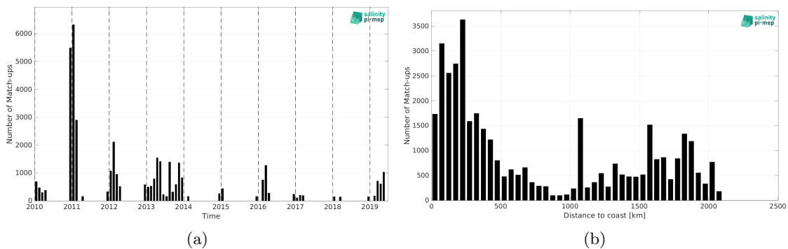
Figure 1: Number of match-ups between TSG (Polarstern) and CCI SSS L4 Merged-OI v3.2 - 7-day running (ESA) SSS as a function of time (a) and as function of the distance to coast (b) over the Southern Ocean Pi-MEP region and for the full satellite product period.
