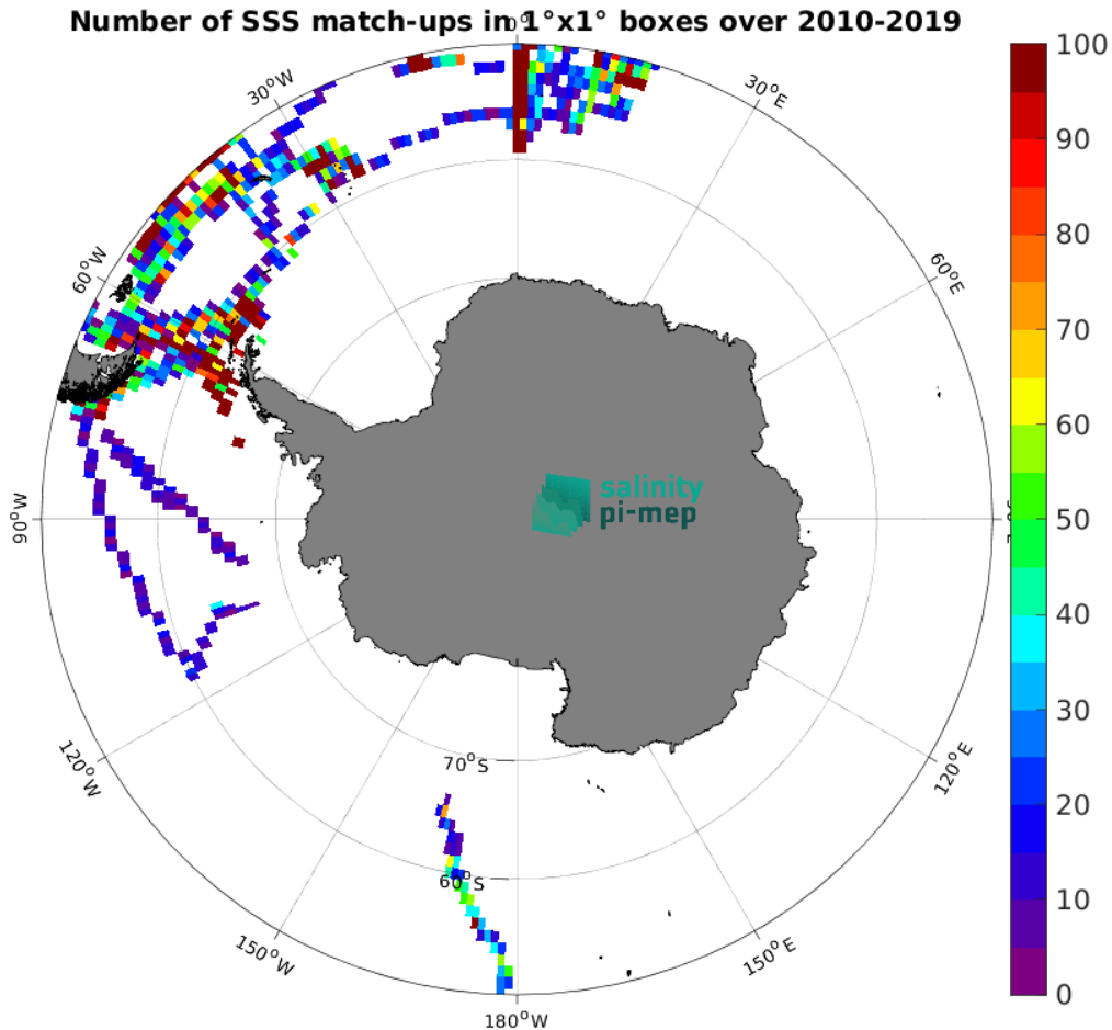
Figure 4: Number of SSS match-ups between TSG (Polarstern) SSS and the CCI SSS L4 Merged-OI v3.2 - 7-day running (ESA) SSS product for the Southern Ocean Pi-MEP region over 1^\circ \times 1^\circ boxes and for the full satellite product period.
