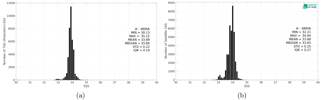
Figure 2: Histograms of SSS from TSG (Polarstern) (a) and CCI SSS L4 Merged-OI v3.2 - 7-day running (ESA) (b) considering all match-up pairs per bins of 0.1 over the Southern Ocean Pi-MEP region and for the full satellite product period.
