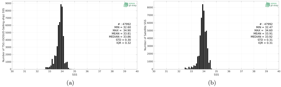
Figure 2: Histograms of SSS from TSG (GOSUD-Sailing-ship) (a) and CCI SSS L4 Merged-OI v3.2 - 7-day running (ESA) (b) considering all match-up pairs per bins of 0.1 over the Southern Ocean Pi-MEP region and for the full satellite product period.
