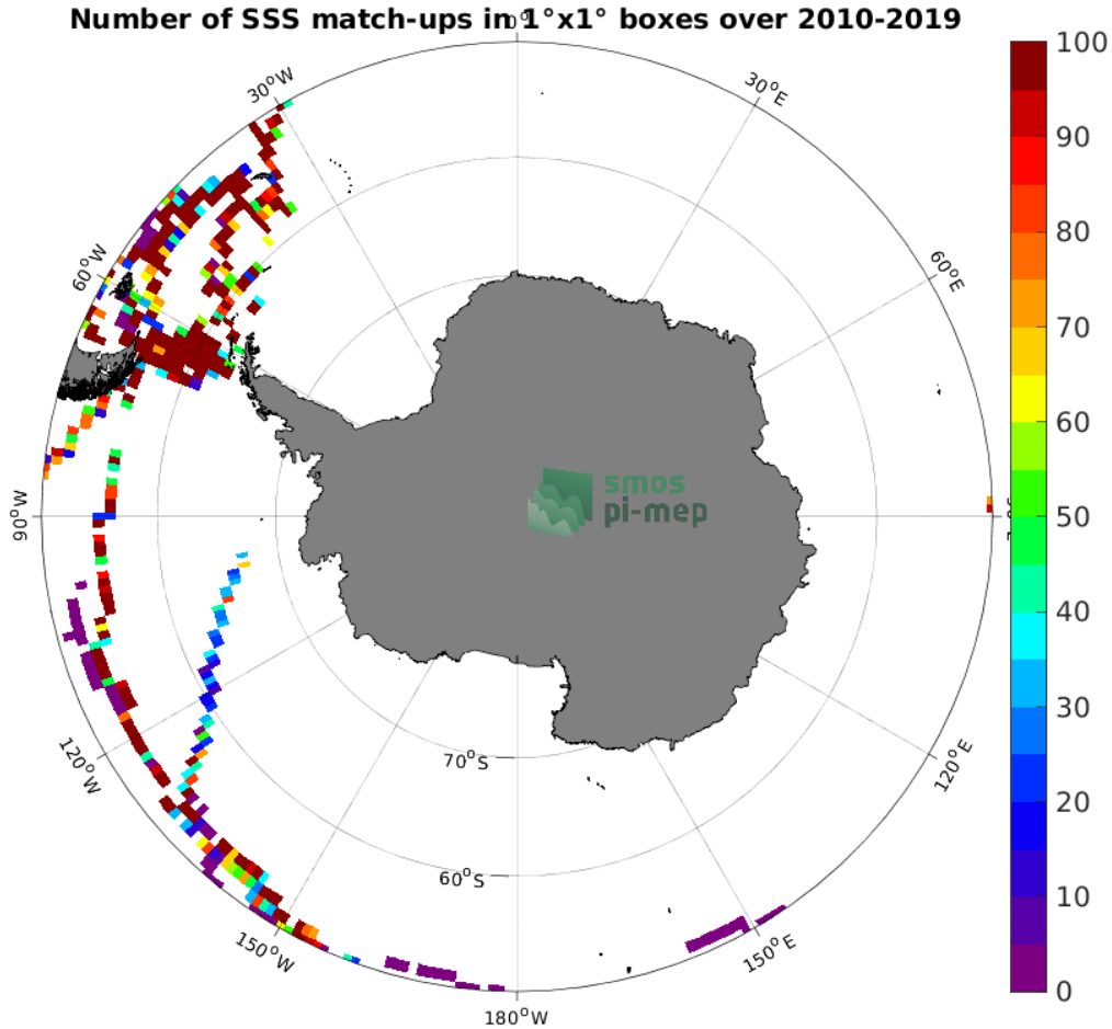
Figure 4: Number of SSS match-ups between TSG (GOSUD-Sailing-ship) SSS and the CCI SSS L4 Merged-OI v3.2 - 7-day running (ESA) SSS product for the Southern Ocean Pi-MEP region over 1^\circ \times 1^\circ boxes and for the full satellite product period.
