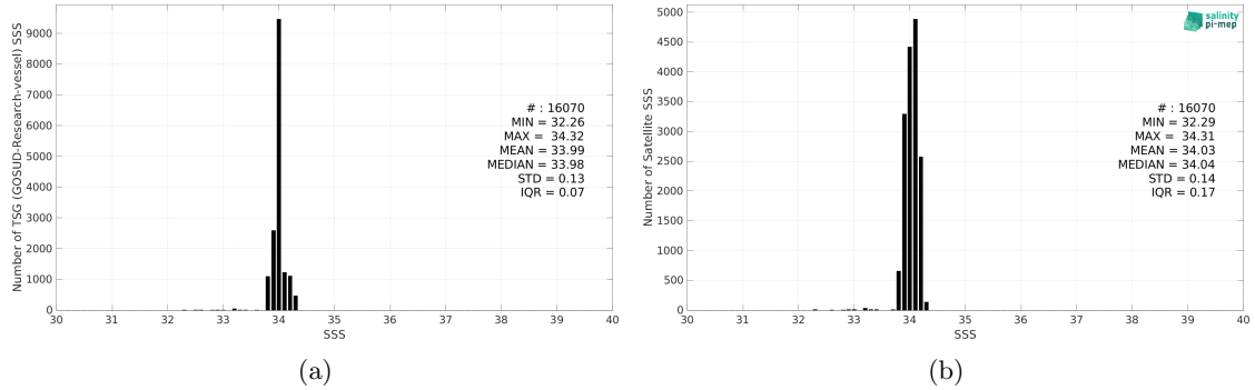
Figure 2: Histograms of SSS from TSG (GOSUD-Research-vessel) (a) and CCI SSS L4 Merged-OI v3.2 - 7-day running (ESA) (b) considering all match-up pairs per bins of 0.1 over the Southern Ocean Pi-MEP region and for the full satellite product period.
