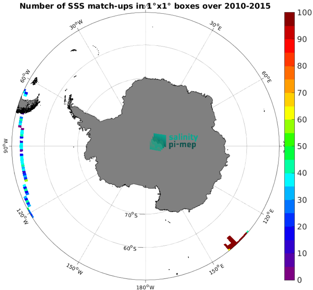
Figure 4: Number of SSS match-ups between TSG (GOSUD-Research-vessel) SSS and the CCI SSS L4 Merged-OI v3.2 - 7-day running (ESA) SSS product for the Southern Ocean Pi-MEP region over 1^\circ \times 1^\circ boxes and for the full satellite product period.
