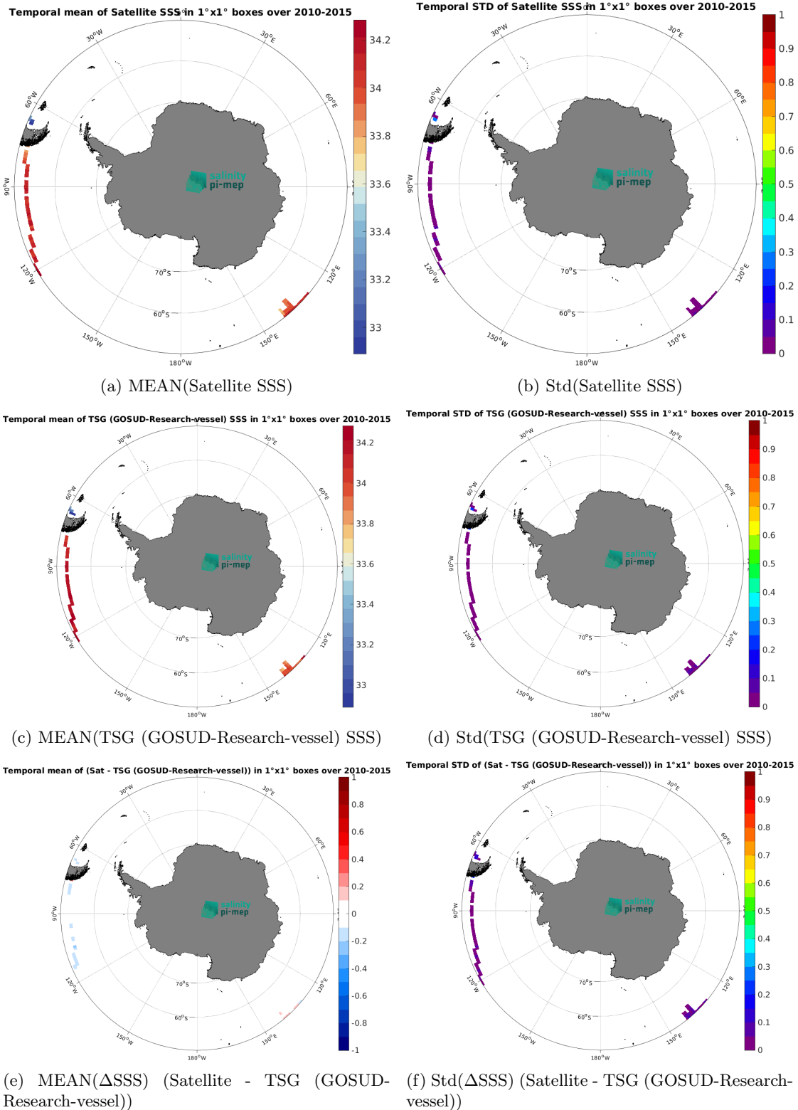
Figure 6: Temporal mean (left) and Std (right) of SSS from CCI SSS L4 Merged-OI v3.2 - 7-day running (ESA) (top), TSG (GOSUD-Research-vessel) (middle), and of \Delta SSS (Satellite - TSG (GOSUD-Research-vessel)). Only match-up pairs are used to generate these maps.
