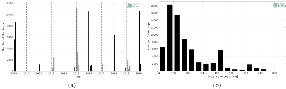
Figure 1: Number of match-ups between TSG (CSIC-UTM) and CCI SSS L4 Merged-OI v3.2 - 7-day running (ESA) SSS as a function of time (a) and as function of the distance to coast (b) over the Southern Ocean Pi-MEP region and for the full satellite product period.
