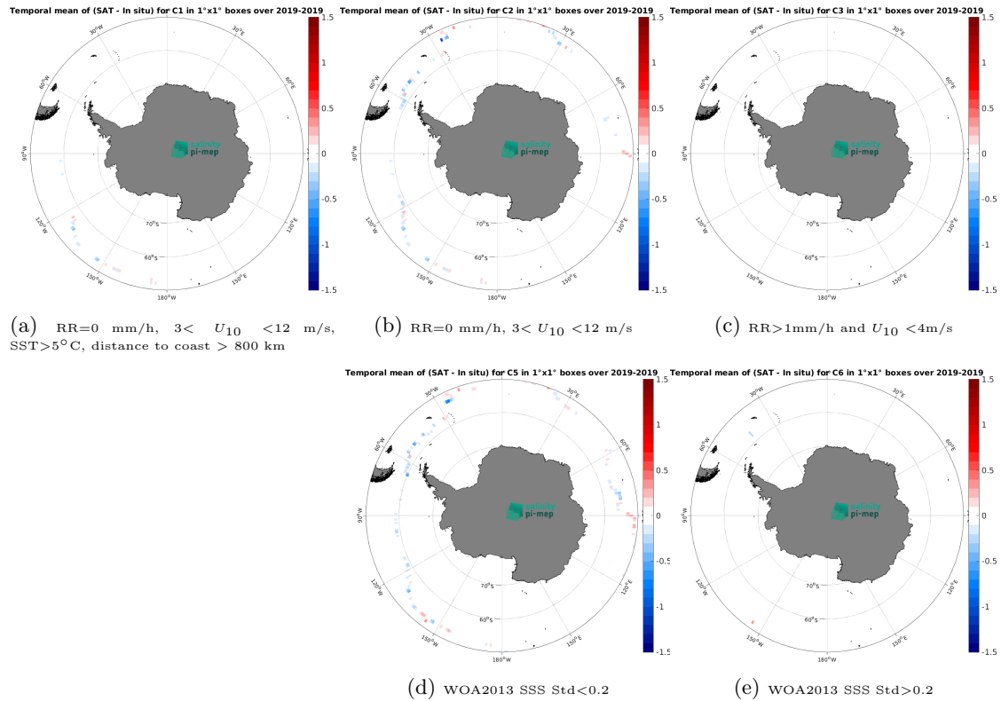
Figure 12: Temporal mean gridded over spatial boxes of size 1^{\circ}\times 1^{\circ} of \Delta\text{SSS} (CCI SSS L4 Merged-OI v3.2 - 7-day running (ESA) - Sailydrone) for 5 different subdatasets corresponding to:RR=0 mm/h, 3 < U_{10} < 12 m/s, SST >5^{\circ}\text{C} , distance to coast > 800 km (a), RR=0 mm/h, 3 < U_{10} < 12 m/s (b), RR >1 mm/h and U_{10} < 4 m/s (c), WOA2013 SSS Std <0.2 (d), WOA2013 SSS Std >0.2 (e).
