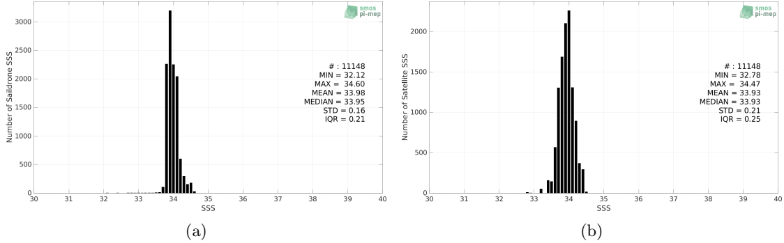
Figure 2: Histograms of SSS from Saildrone (a) and CCI SSS L4 Merged-OI v3.2 - 7-day running (ESA) (b) considering all match-up pairs per bins of 0.1 over the Southern Ocean Pi-MEP region and for the full satellite product period.
