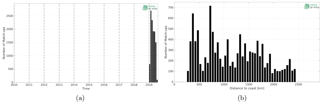
Figure 1: Number of match-ups between Saildrone and CCI SSS L4 Merged-OI v3.2 - 7-day running (ESA) SSS as a function of time (a) and as function of the distance to coast (b) over the Southern Ocean Pi-MEP region and for the full satellite product period.
