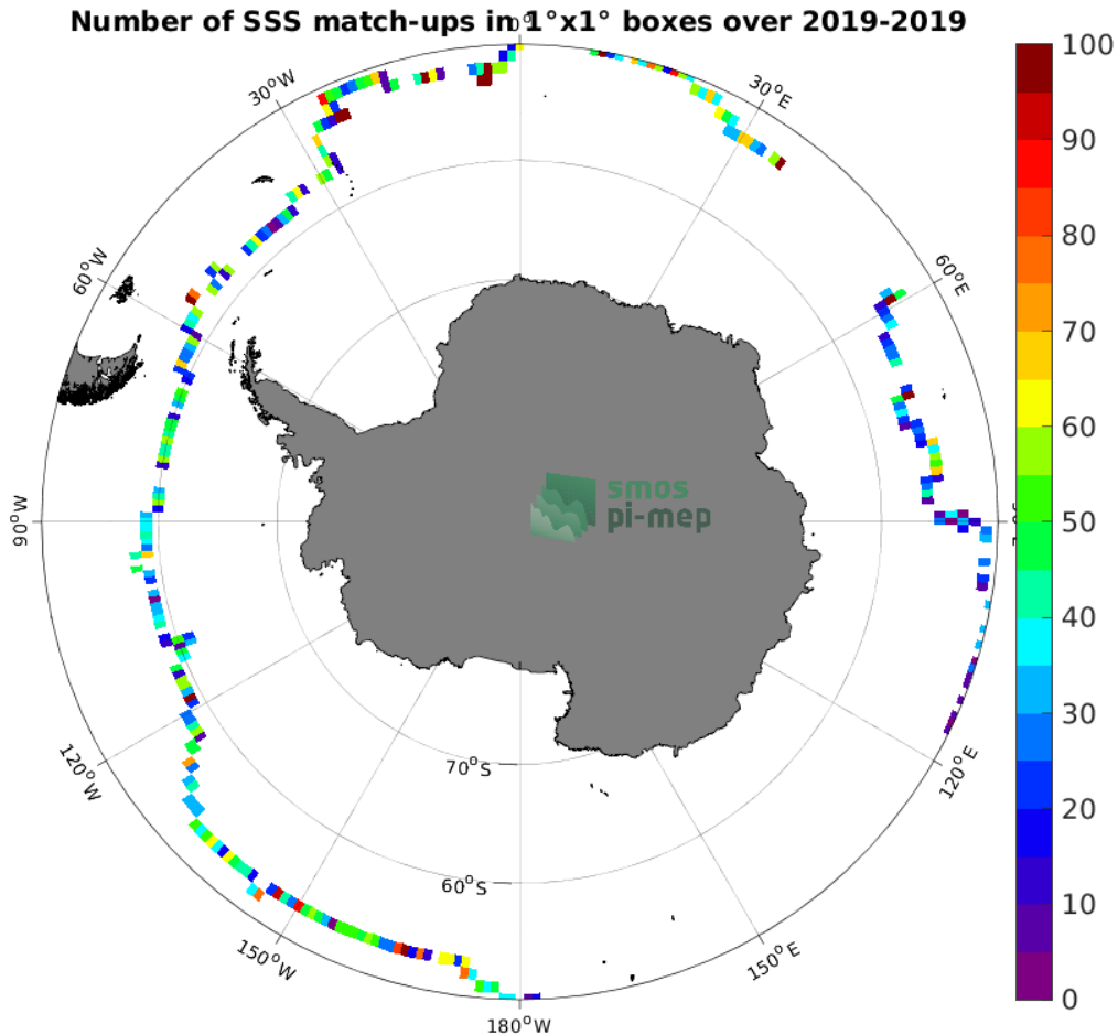
Figure 4: Number of SSS match-ups between Saildrone SSS and the CCI SSS L4 Merged-OI v3.2 - 7-day running (ESA) SSS product for the Southern Ocean Pi-MEP region over 1^\circ \times 1^\circ boxes and for the full satellite product period.
