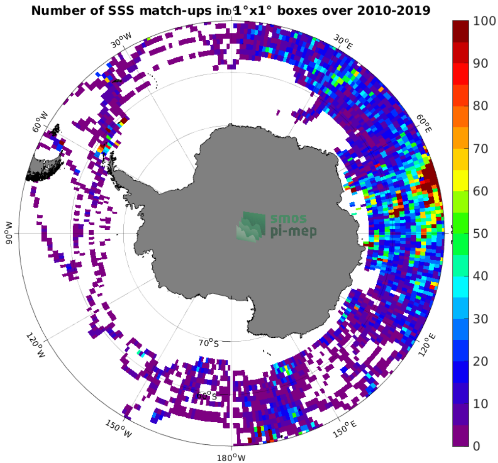
Figure 4: Number of SSS match-ups between Marine mammals SSS and the CCI SSS L4 Merged-OI v3.2 - 7-day running (ESA) SSS product for the Southern Ocean Pi-MEP region over 1^\circ \times 1^\circ boxes and for the full satellite product period.
