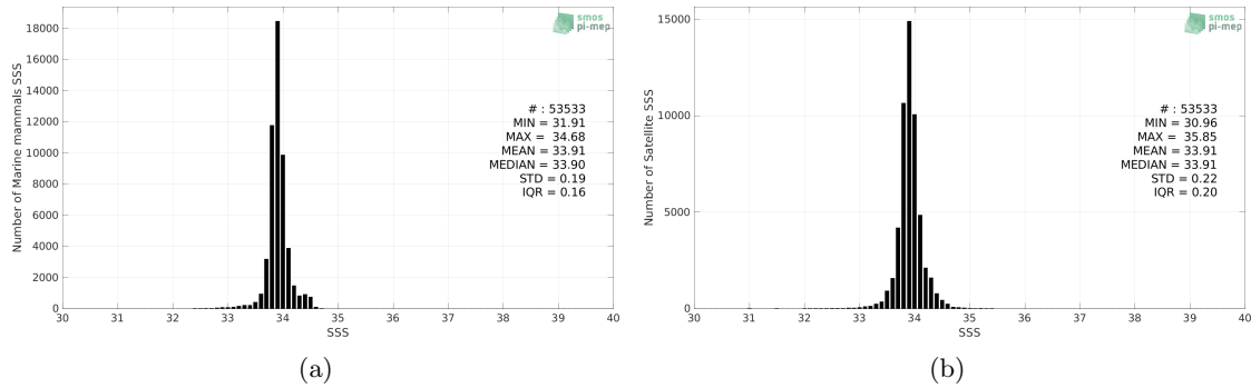
Figure 2: Histograms of SSS from Marine mammals (a) and CCI SSS L4 Merged-OI v3.2 - 7-day running (ESA) (b) considering all match-up pairs per bins of 0.1 over the Southern Ocean Pi-MEP region and for the full satellite product period.
