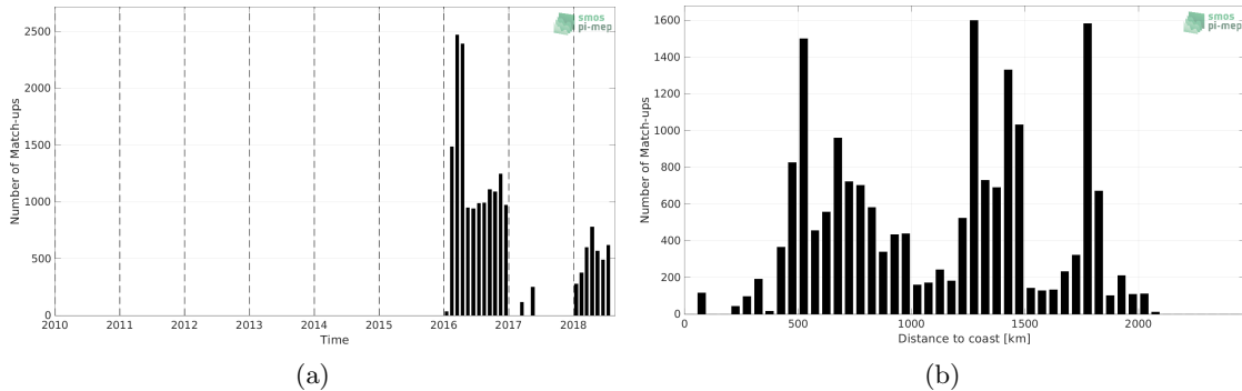
Figure 1: Number of match-ups between Surface drifters and CCI SSS L4 Merged-OI v3.2 - 7-day running (ESA) SSS as a function of time (a) and as function of the distance to coast (b) over the Southern Ocean Pi-MEP region and for the full satellite product period.
