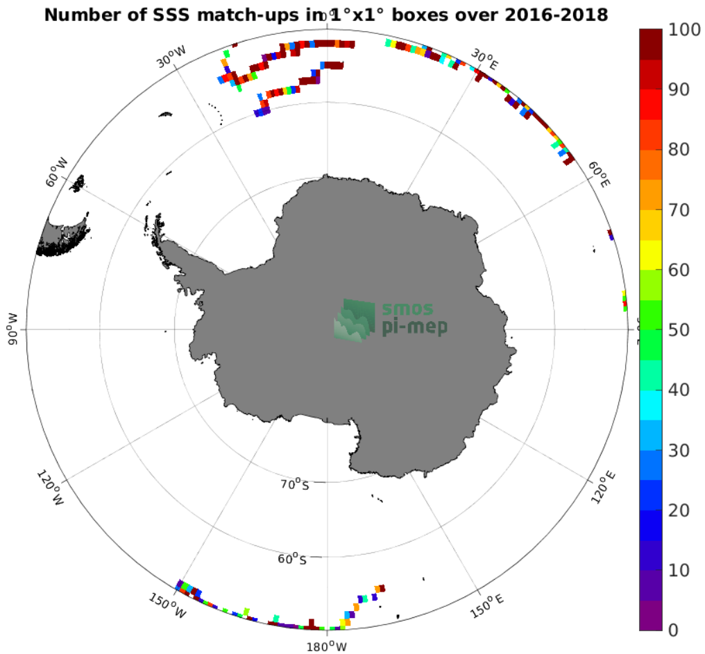
Figure 3: Number of SSS match-ups between Surface drifters SSS and the CCI SSS L4 Merged-OI v3.2 - 7-day running (ESA) SSS product for the Southern Ocean Pi-MEP region over 1^\circ \times 1^\circ boxes and for the full satellite product period.
