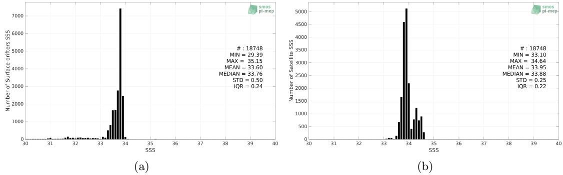
Figure 2: Histograms of SSS from Surface drifters (a) and CCI SSS L4 Merged-OI v3.2 - 7-day running (ESA) (b) considering all match-up pairs per bins of 0.1 over the Southern Ocean Pi-MEP region and for the full satellite product period.
